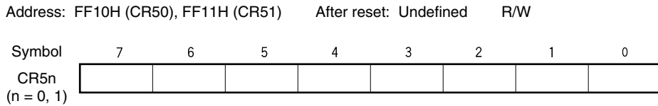
★ Figure 9-4. Format of 8-Bit Timer Compare Register 5n (CR5n)
