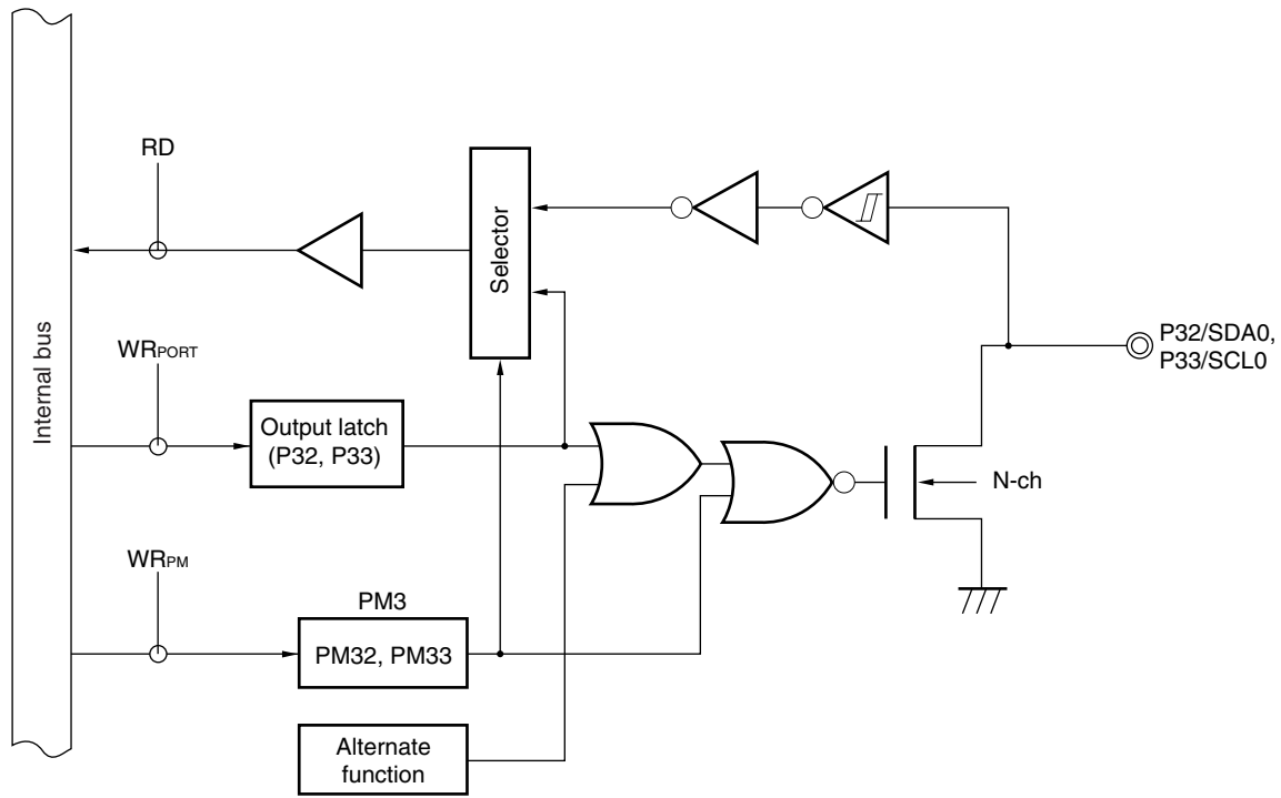
Figure 6-12. Block Diagram of P32 and P33 ( \mu PD780078Y Subseries)
