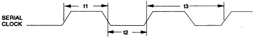
FIGURE 8 - CLOCK TIMING
