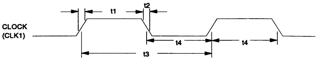
FIGURE 7 - RESET TIMING
