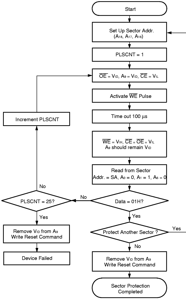
Figure 16 Sector Protection Algorithm
