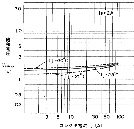
飽和電圧—コレクタ電流特性 Base and Saturation Voltage
