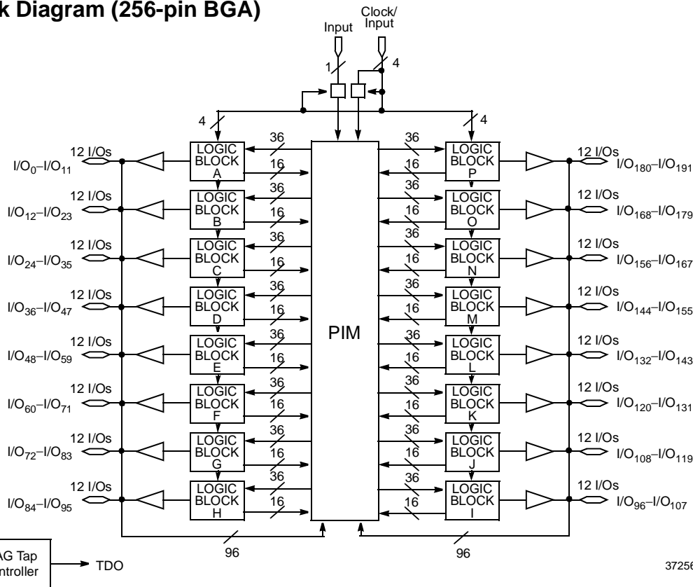
Logic Block Diagram (256-pin BGA)
