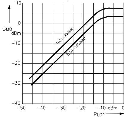
10.3 Diagram 3: First Mixer: Mixer gain versus LO-Level P_{LO1} , IF = 336MHz
