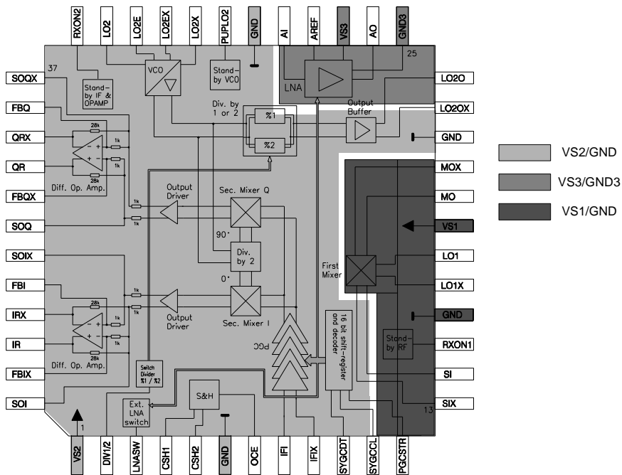
Figure 2.2: Supply Function
