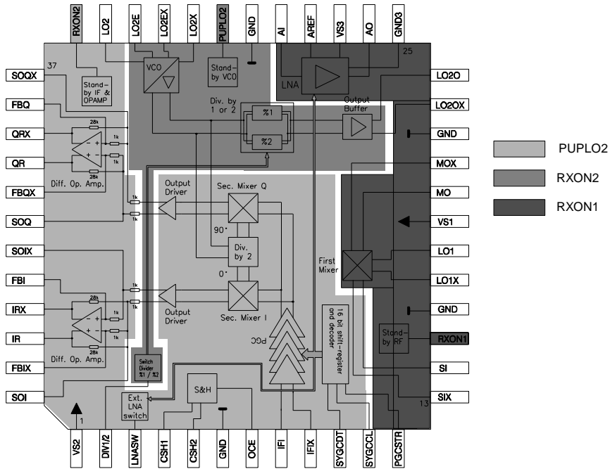
Figure 2.2: Supply Function
