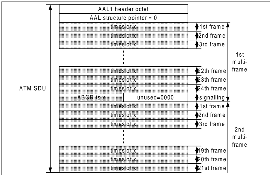
Figure 79 Example Multiframe Structure for 1x64 kbit/s DS1 with CAS
