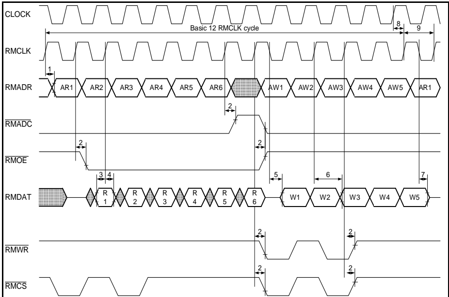
Figure 71 RAM Interface Timing Diagram
