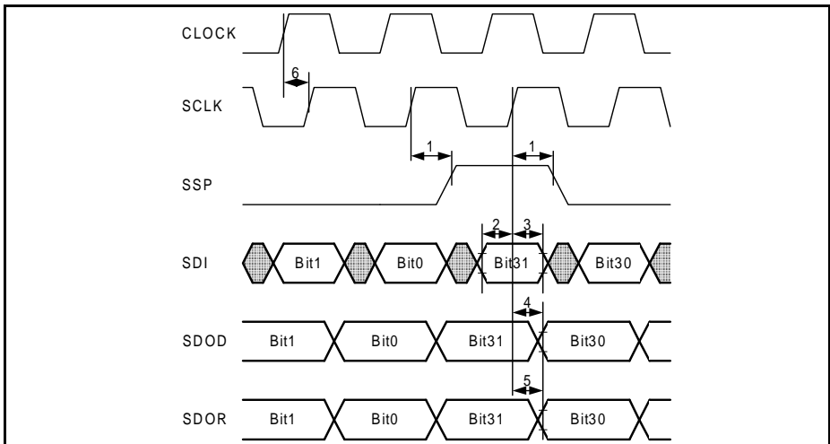
Figure 67 Clock Recovery Interface Timing Diagram
