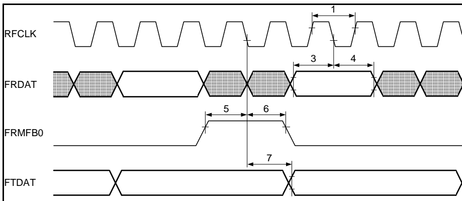
Figure 62 Framer Interface Timing in SYM 8.192 MHz
