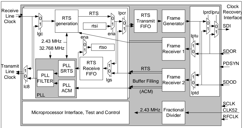
Figure 19 Block Diagram of the ICRC
