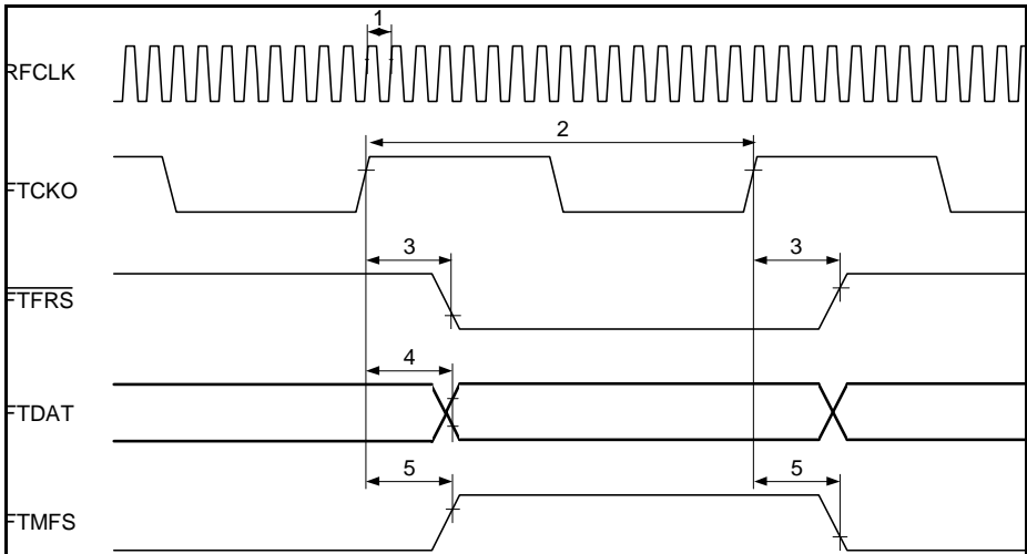
Figure 60 Framer Transmit Interface Timing in GIM
