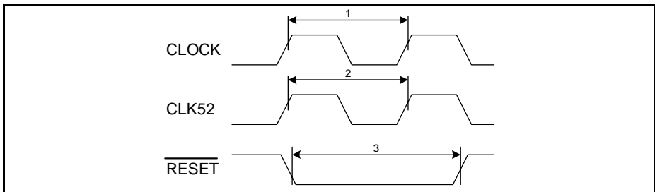
Figure 56 Clock and Reset Interface Timing Diagram
