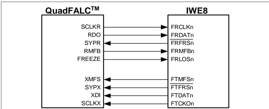
Figure 22 Connection of IWE8 to QuadFALC
