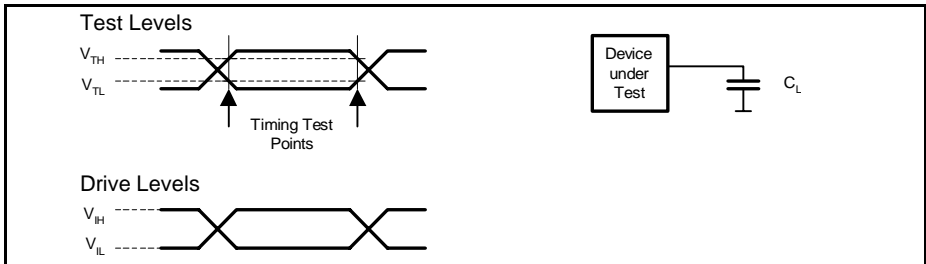
Figure 55 Input/Output Waveforms for AC Measurements
