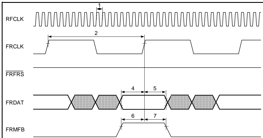
Figure 59 Framer Receive Interface Timing in GIM
