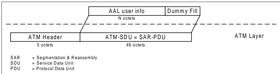
Figure 13 SAR-PDU of AAL Type 0
