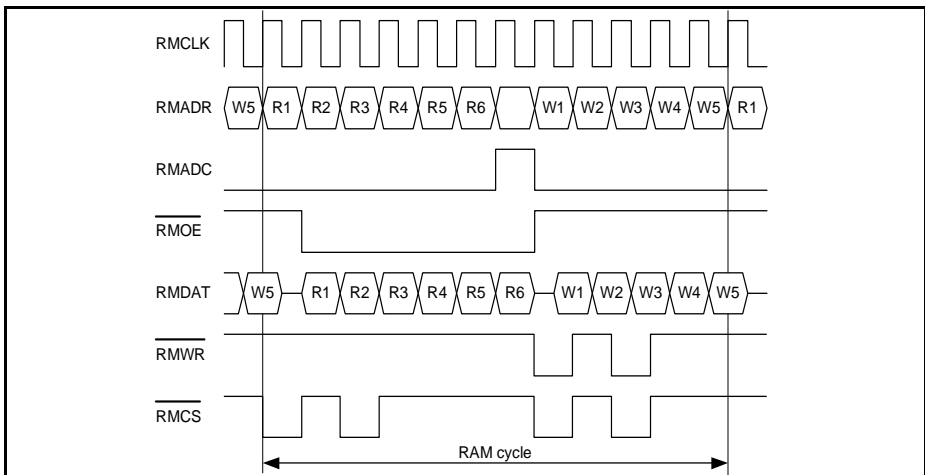
Figure 35 RAM Interface Protocol
