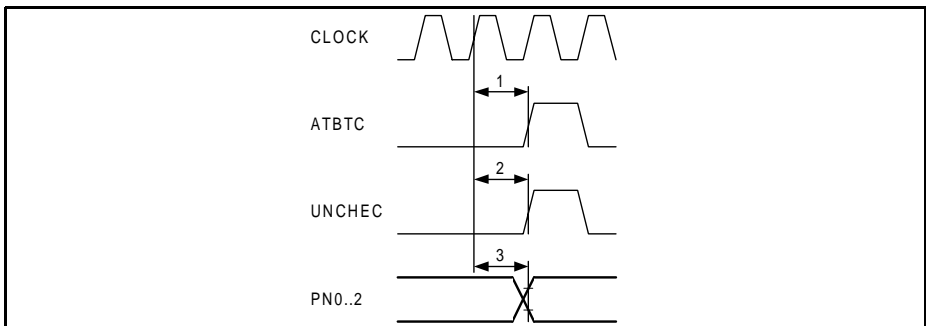
Figure 66 Timing of the IMA Interface
