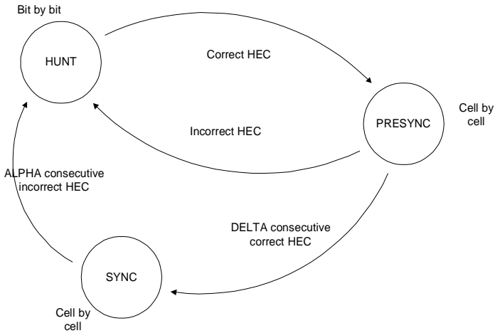
Figure 7 Cell delineation state diagram (Figure 5/I.432.1)
