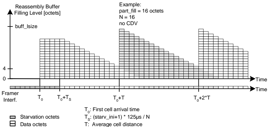
Figure 15 Reassembly Buffer Initialization: No CDV
