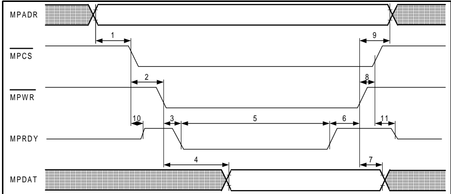
Figure 68 Intel Mode Write Cycle Timing Diagram
