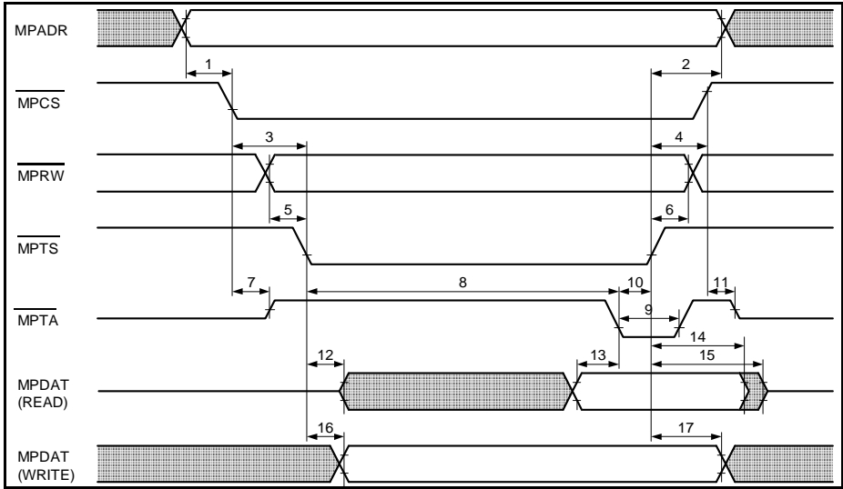
Figure 70 Motorola Mode Timing Diagram
