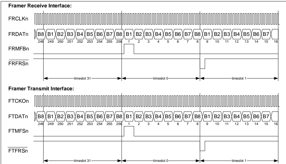
Figure 23 Framers Interface in FAM
