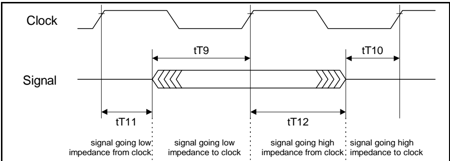
Figure 65 Tri-state timing (multi-PHY, multiple devices only)
