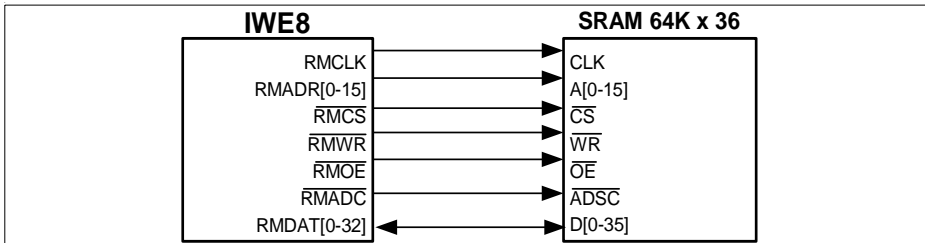
Figure 34 External RAM Connection
