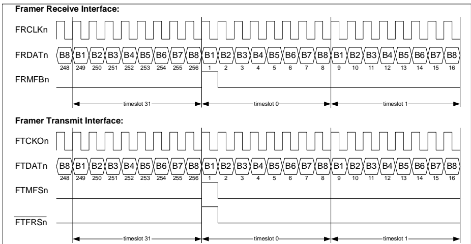
Figure 25 Framer Interface in GIM E1
