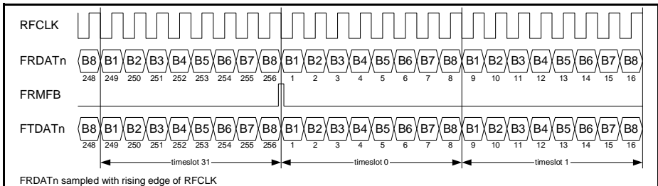
Figure 26 Framer Interface in SYM2 E1
