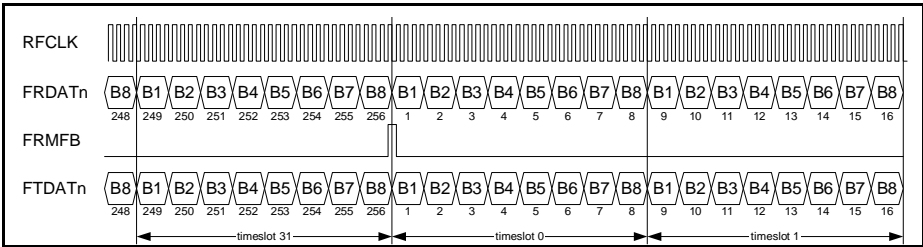
Figure 27 Framer Interface in SYM8 E1
