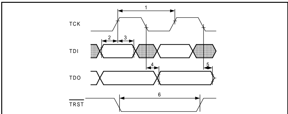
Figure 72 Boundary-Scan Test Interface Timing Diagram
