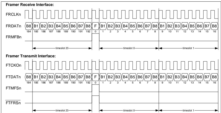
Figure 24 Framer Interface in GIM T1
