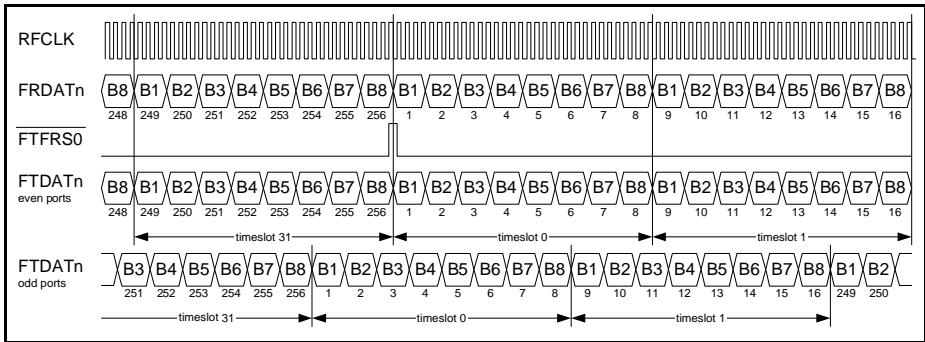
Figure 28 Framer Interface in EC Mode
