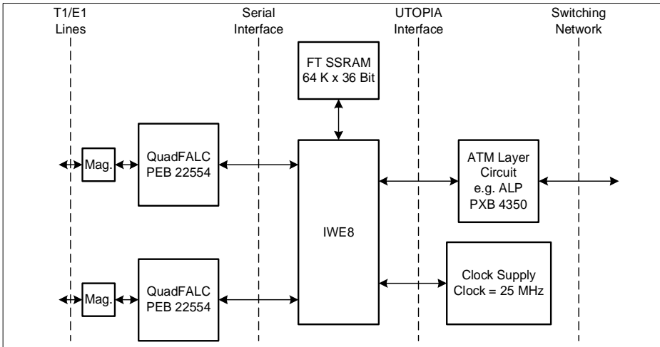
Figure 3 Line Card for 8 T1/E1 Channels
