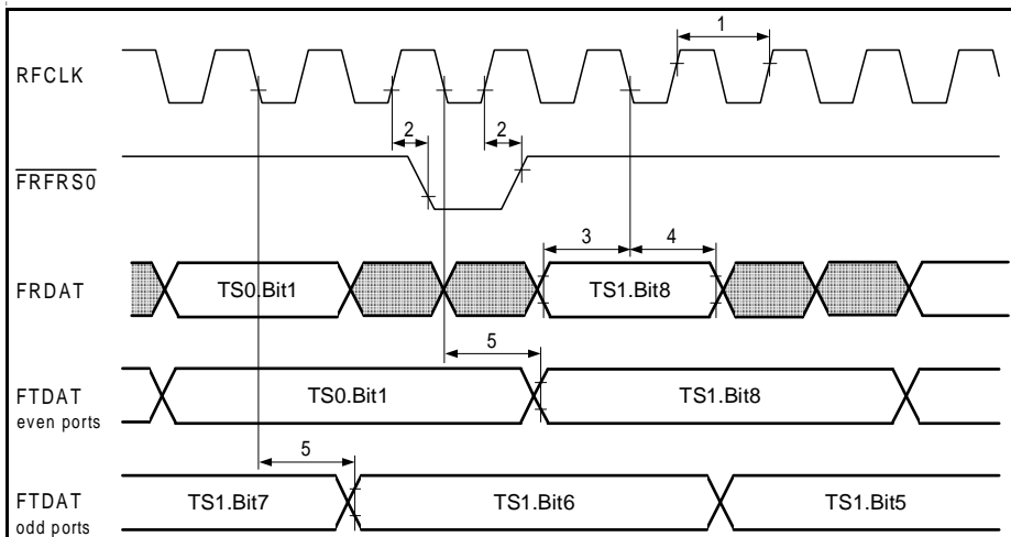
Figure 63 Framers Interface Timing in EC Mode
