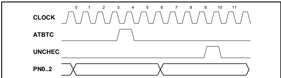
Figure 31 IMA Interface Protocol
