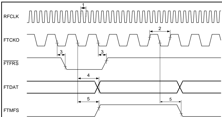
Figure 58 Framer Transmit Interface Timing in FAM
