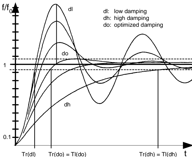
Figure 21 Influence of Damping on Lock in Time
