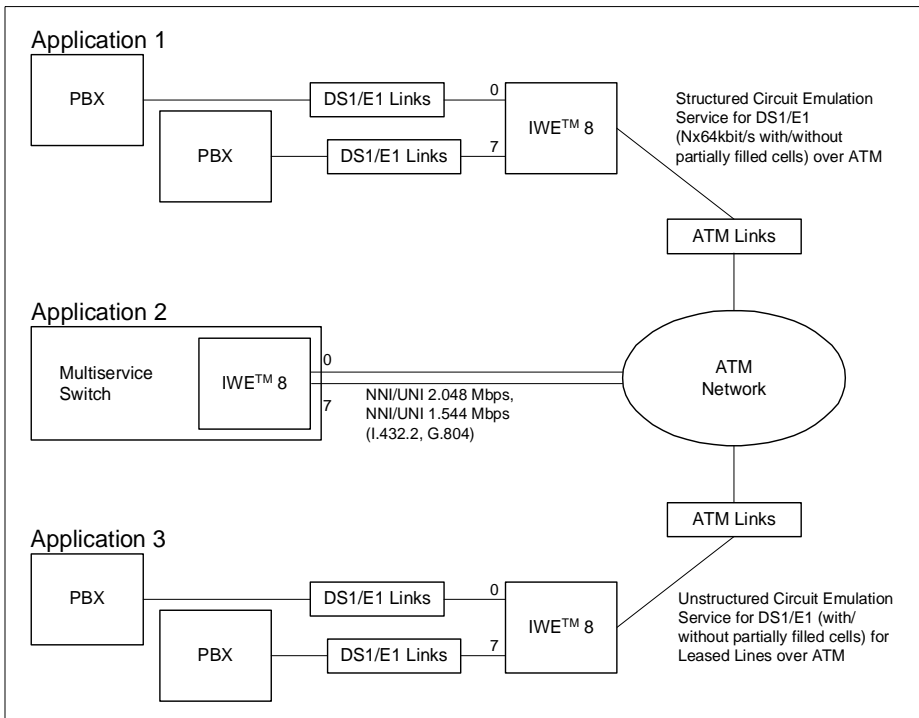
Figure 2 Typical IWE8 Applications
