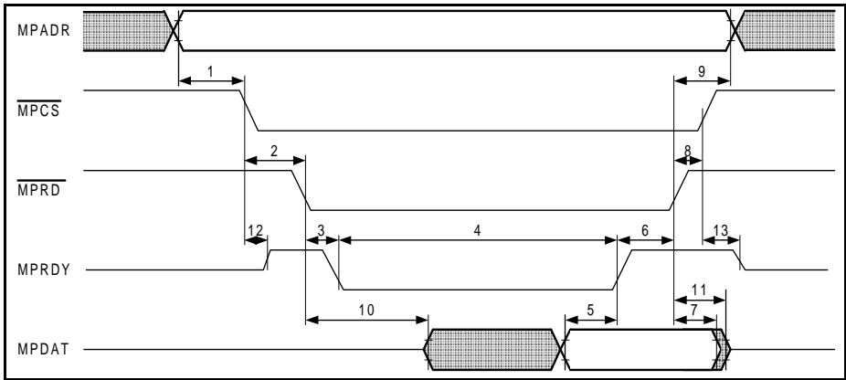
Figure 69 Intel Mode Read Cycle Timing Diagram
