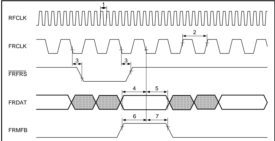
Figure 57 Framer Receive Interface Timing in FAM
