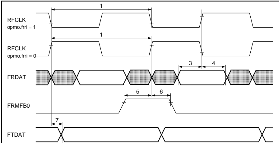
Figure 61 Framers Interface Timing for SYM 2.048 MHz
