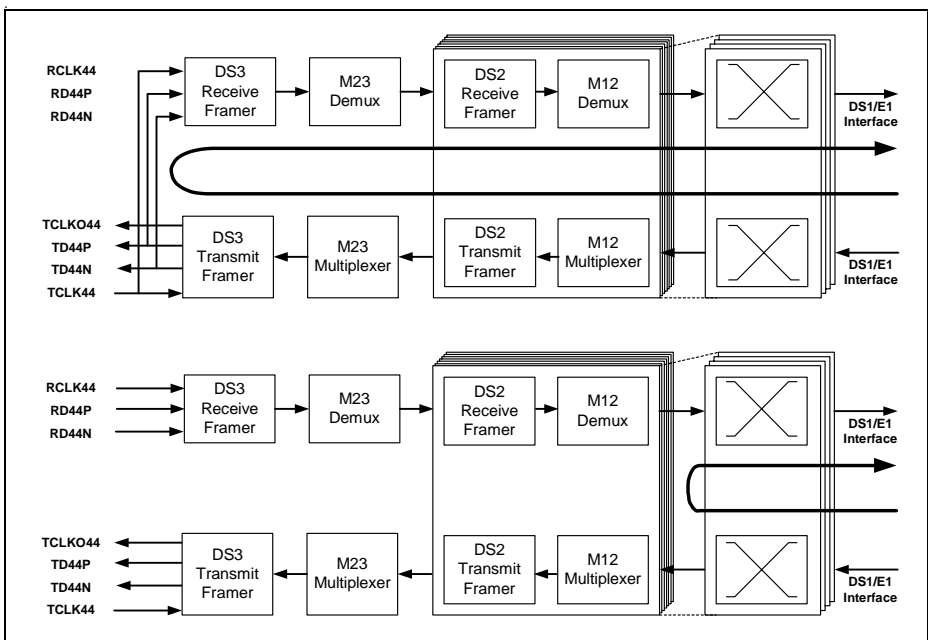
Figure 5 Local Loops
