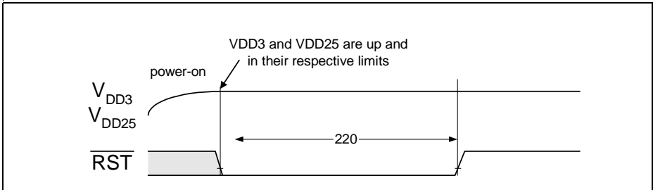
Figure 51 Reset Timing
