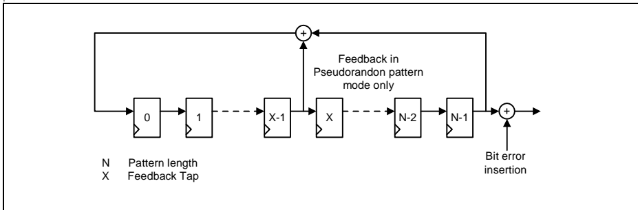
Figure 15 Pattern Generator
