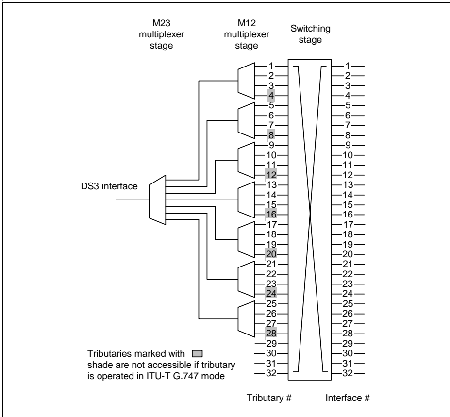
Figure 7 Tributary Mapper
