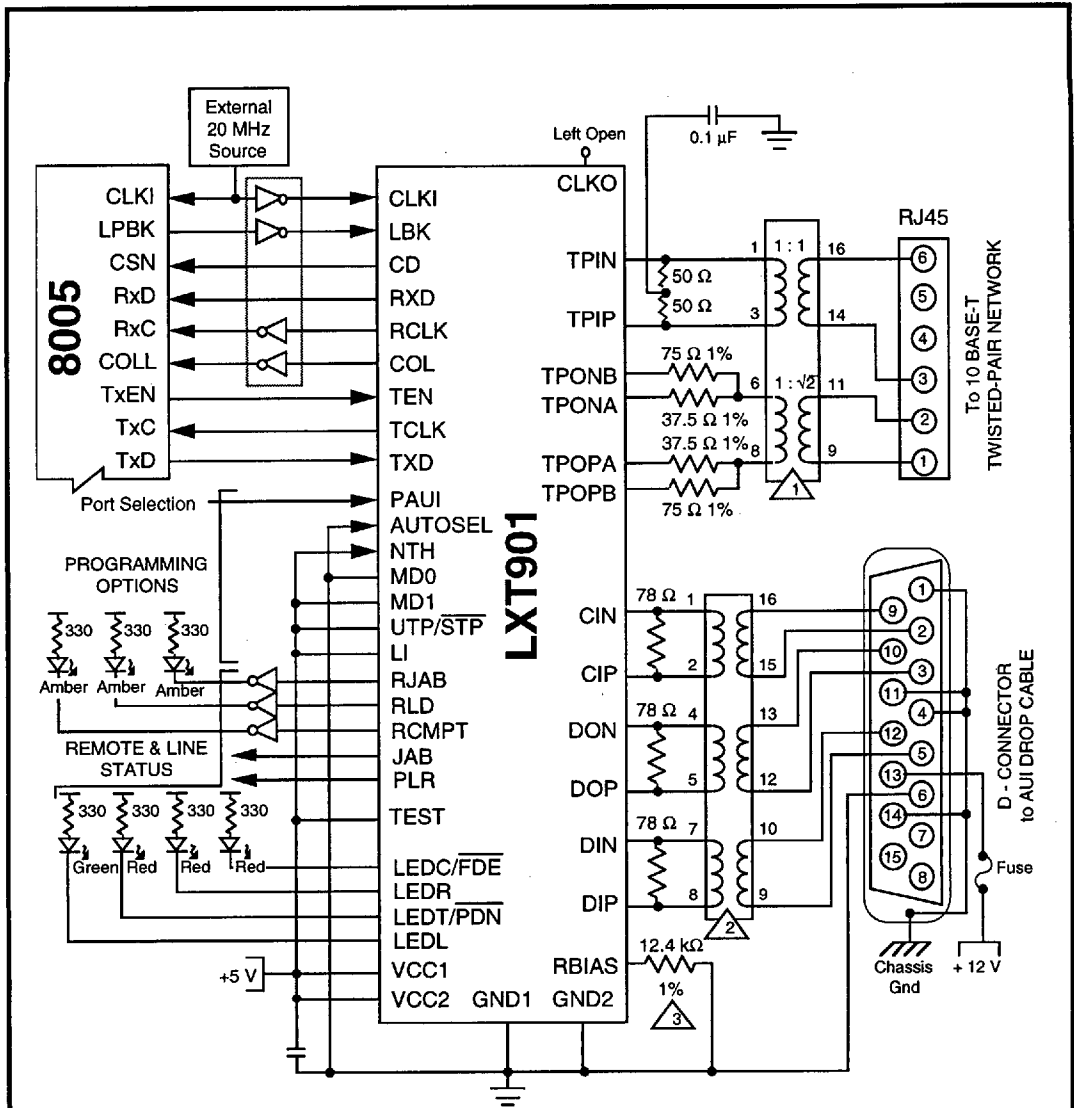
Figure 11: Manual Port Select with Seeq 8005 Controller
