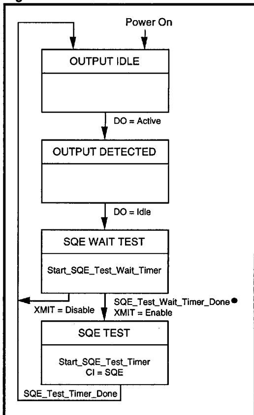
Figure 4: SQE Function
