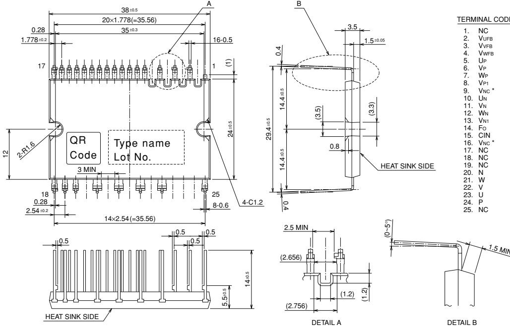
Fig. 2 LONG TERMINAL TYPE PACKAGE OUTLINES (PS21962-AT)
