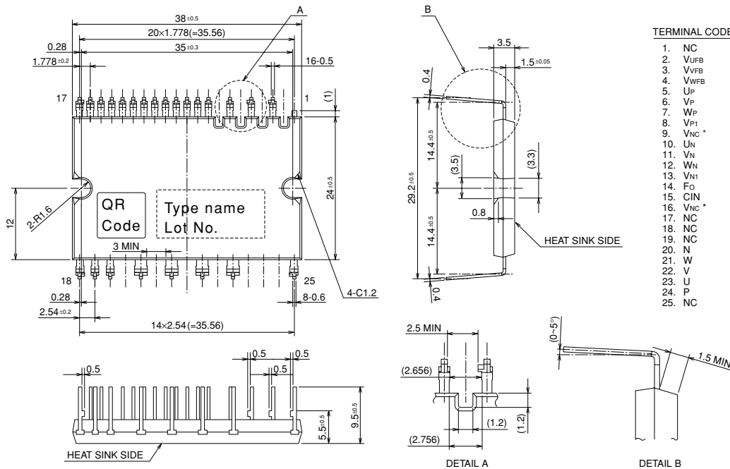
Fig. 1 PACKAGE OUTLINES (PS21962-T)
