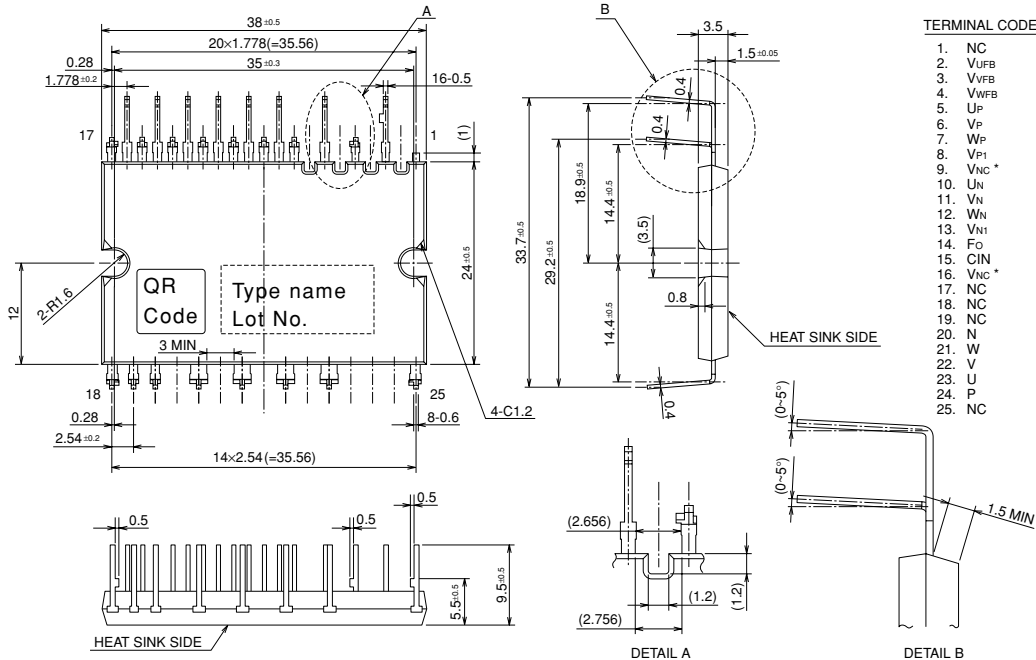
Fig. 3 ZIGZAG TERMINAL TYPE PACKAGE OUTLINES (PS21962-CT)
