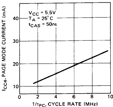
Fig. 13 – PAGE MODE CURRENT vs CYCLE RATE
