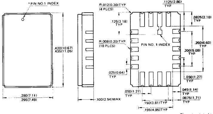
18-PAD CERAMIC (FRIT SEAL) LEADLESS CHIP CARRIER (CASE No.: LCC-18C-F02)
