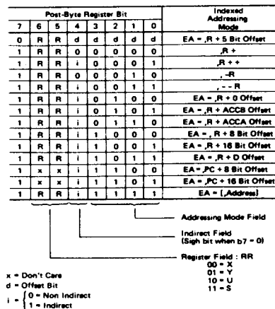
Figure 16 Index Addressing Postbyte Register Bit Assignments
