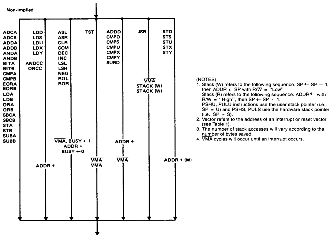
Figure 18 Address Bus Cycle-by-Cycle Performance (Continued)
