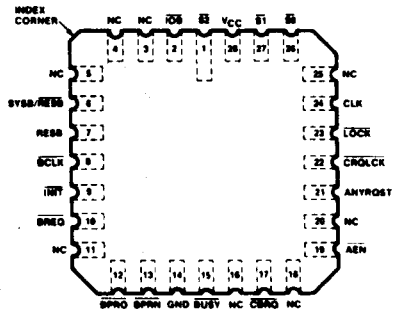
Figure 3. M8289 Pin Diagram
