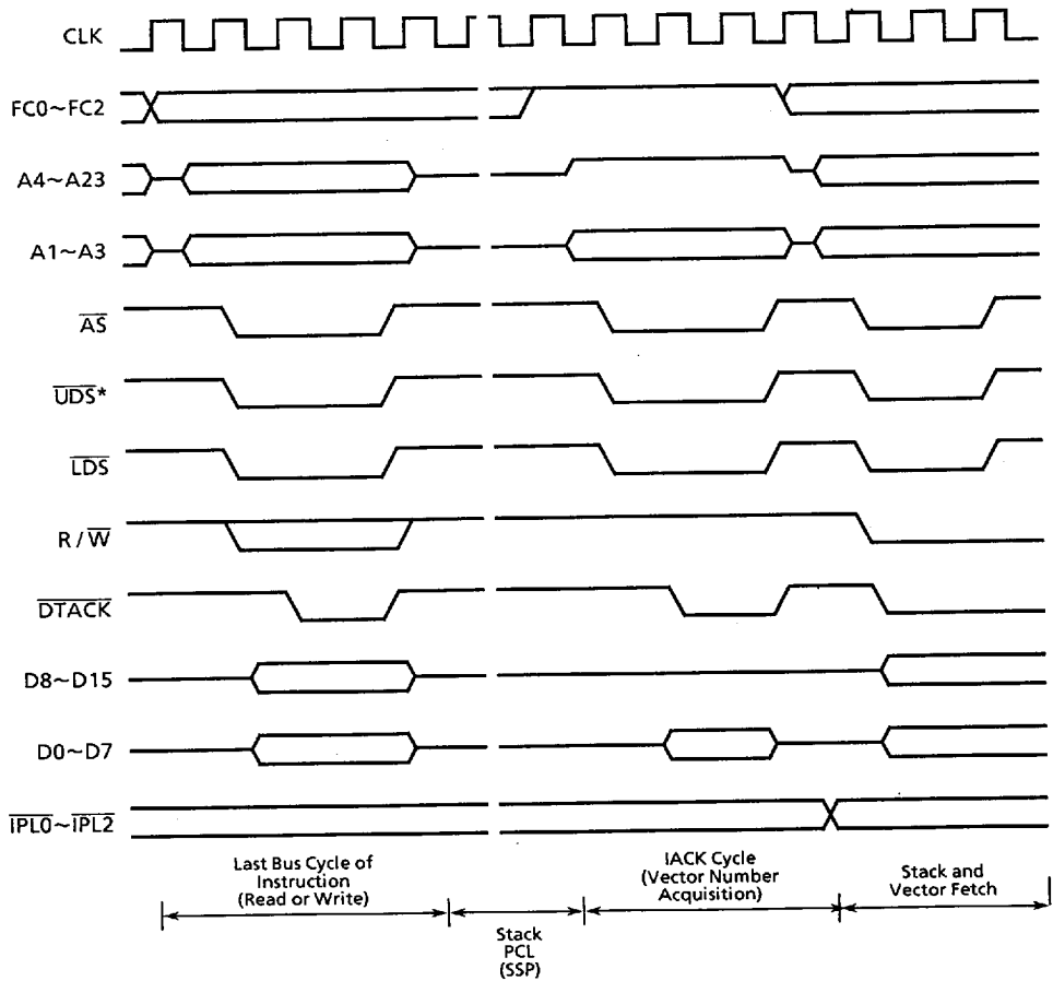
Figure5.6 Interrupt Acknowledge Cycle Timing Diagram
