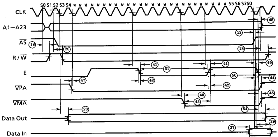
Figure 8.5 TMP68000 to 6800 Peripheral Timing Diagram – Best Case
