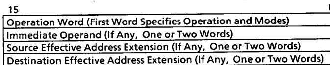
Figure 2.3 Instruction Operation Word General Format
