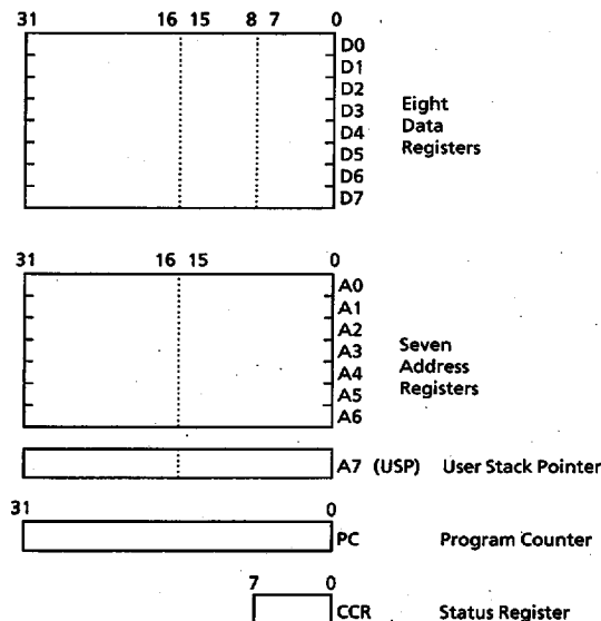
Figure 1.1 User-Programming Model
