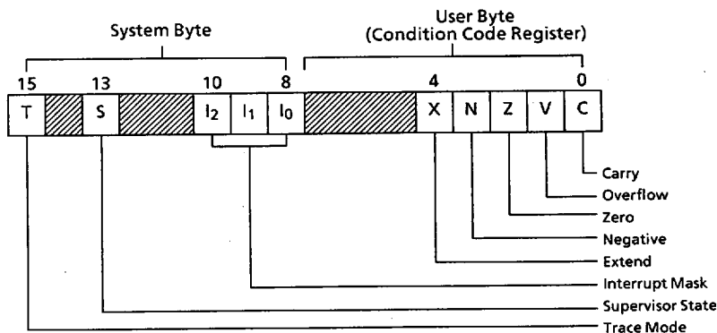
Figure 1.3 Status Register
