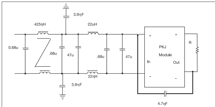
L1: 425µH, 8.1A (Coilcraft P3217A) L2: 22µH, 7A (Coilcraft D055022-223)
