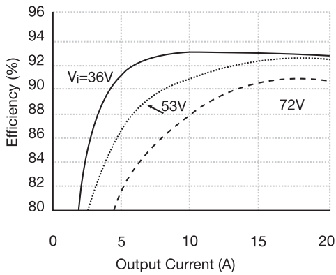
Efficiency (typ)
