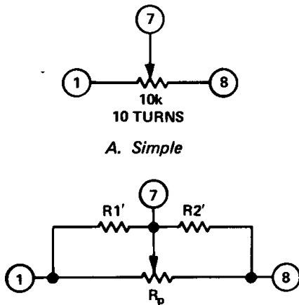
Figure 1. Nulling Circuits
