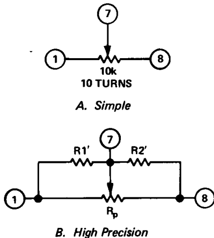
Figure 1. Nulling Circuits
