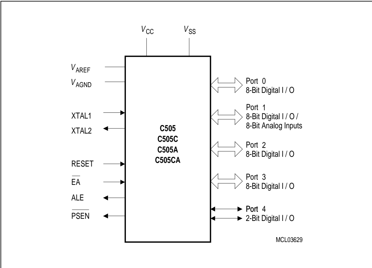
Figure 2 Logic Symbol
