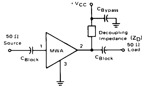
FIGURE 27 – AMPLIFIER SCHEMATIC DIAGRAM
