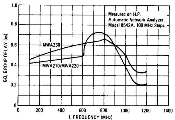
FIGURE 25 – GROUP DELAY versus FREQUENCY
