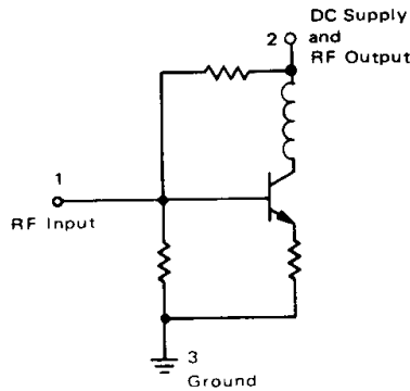
FIGURE 26 – INTERNAL CIRCUIT
