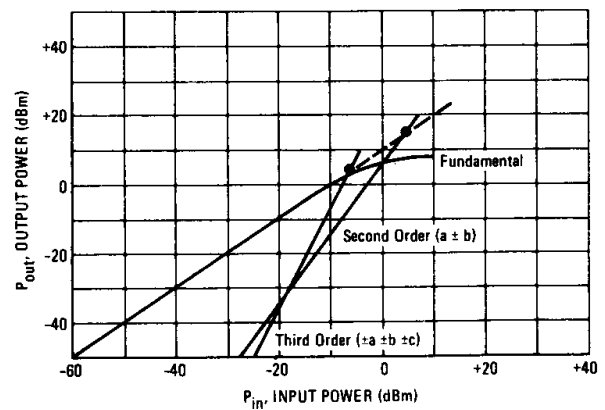
FIGURE 19 – SECOND AND THIRD ORDER INTERCEPT MWA210
