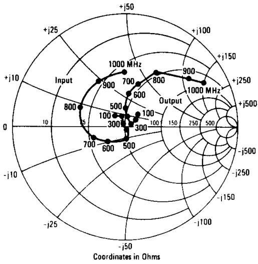
FIGURE 10 – INPUT AND OUTPUT IMPEDANCE versus FREQUENCY MWA210
