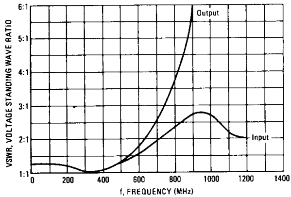
FIGURE 7 – VSWR versus FREQUENCY MWA210
