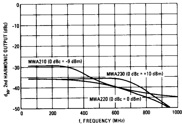
FIGURE 18 – SECOND HARMONIC OUTPUT versus FREQUENCY
