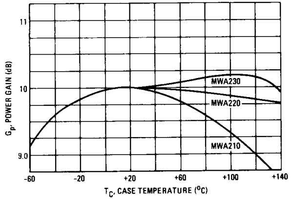
FIGURE 6 – POWER GAIN versus CASE TEMPERATURE f = 600 MHz
