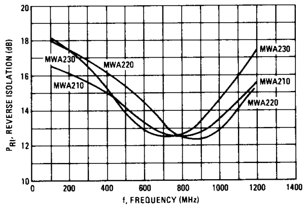
FIGURE 17 – REVERSE ISOLATION versus FREQUENCY
