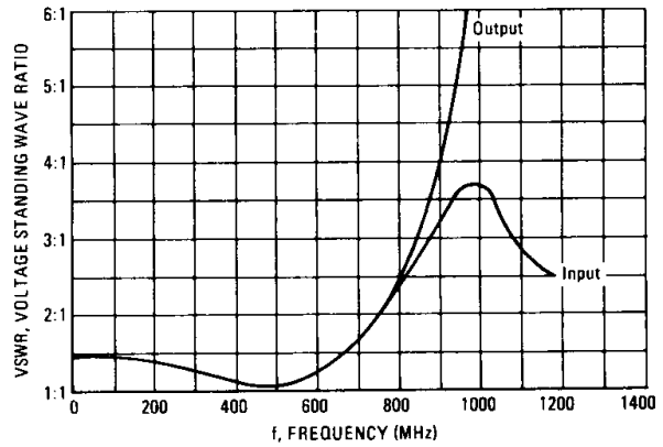
FIGURE 8 – VSWR versus FREQUENCY MWA220
