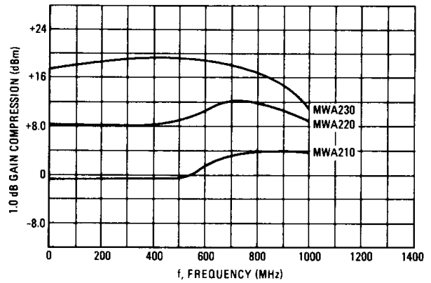
FIGURE 13 – 1.0 dB GAIN COMPRESSION versus FREQUENCY
