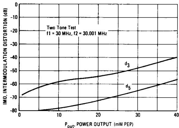
FIGURE 24 – INTERMODULATION DISTORTION versus POWER OUTPUT MWA230
