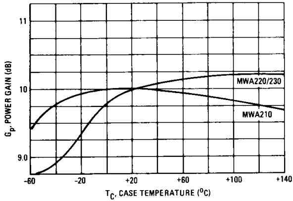
FIGURE 5 – POWER GAIN versus CASE TEMPERATURE f = 100 MHz
