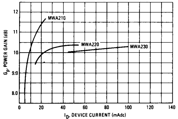
FIGURE 4 – POWER GAIN versus DEVICE CURRENT f = 600 MHz
