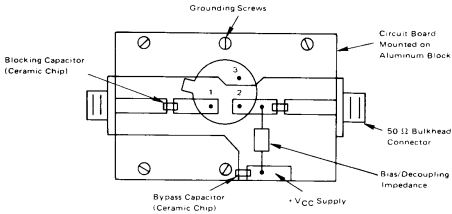
FIGURE 28 — TEST FIXTURE
