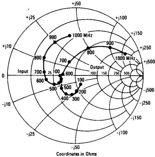
FIGURE 12 – INPUT AND OUTPUT IMPEDANCE versus FREQUENCY MWA230
