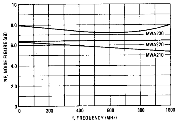
FIGURE 16 – NOISE FIGURE versus FREQUENCY
