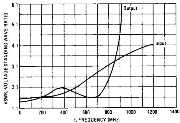
FIGURE 9 – VSWR versus FREQUENCY MWA230
