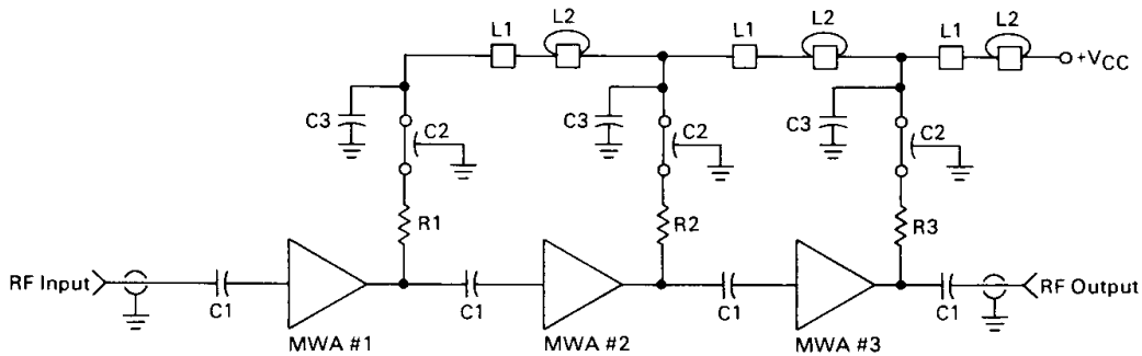
FIGURE 29 — TYPICAL CASCADE
