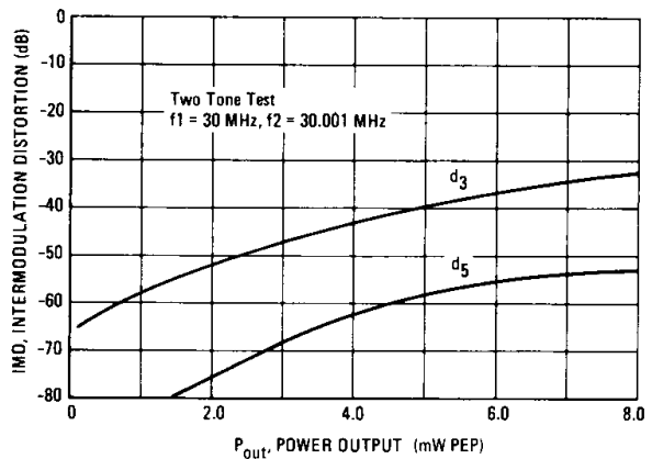
FIGURE 23 – INTERMODULATION DISTORTION versus POWER OUTPUT MWA220
