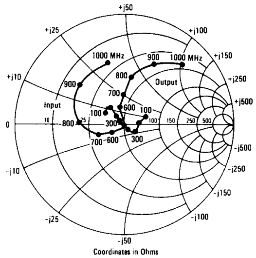
FIGURE 11 – INPUT AND OUTPUT IMPEDANCE versus FREQUENCY MWA220
