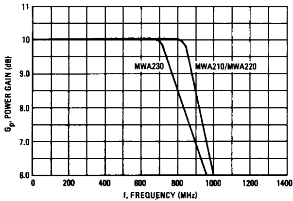
FIGURE 3 – POWER GAIN versus FREQUENCY
