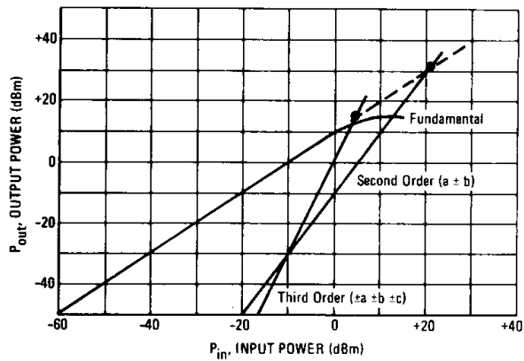
FIGURE 20 – SECOND AND THIRD ORDER INTERCEPT MWA220
