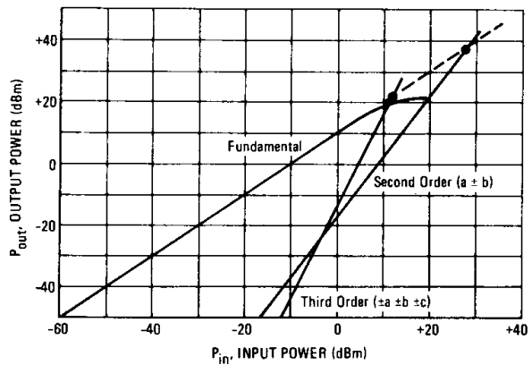
FIGURE 21 – SECOND AND THIRD ORDER INTERCEPT MWA230
