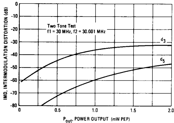
FIGURE 22 – INTERMODULATION DISTORTION versus POWER OUTPUT MWA210
