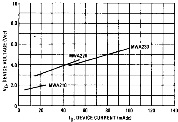
FIGURE 1 – DEVICE VOLTAGE versus DEVICE CURRENT
