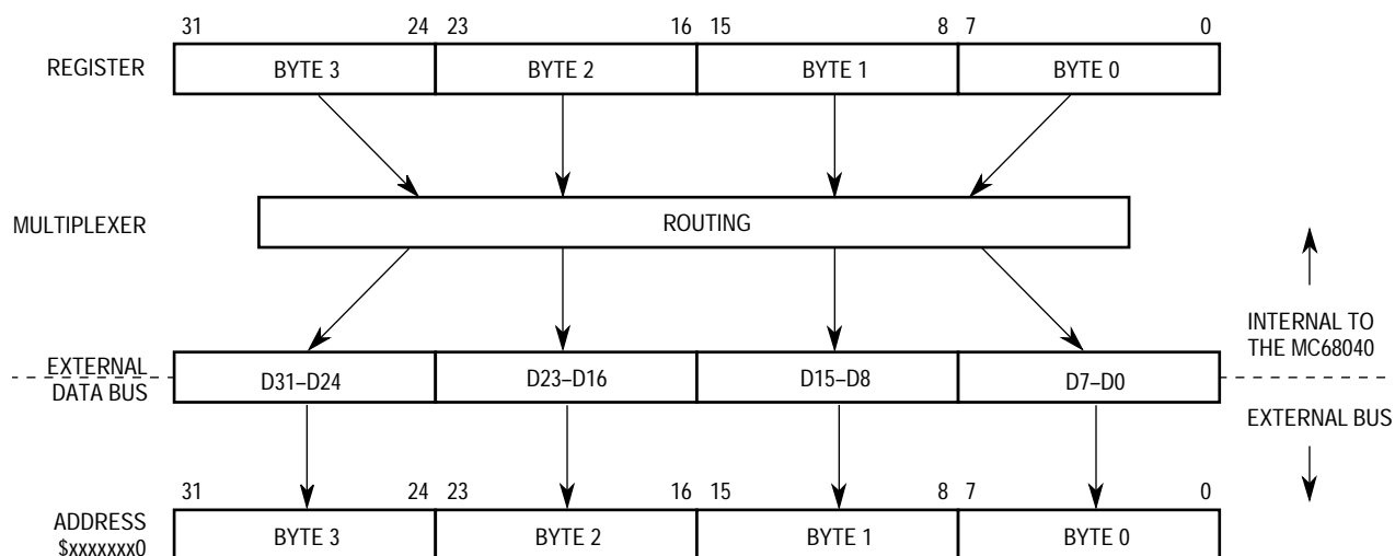
Figure 7-3. Data Multiplexing
