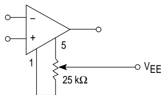
MC34181 Input Offset Voltage Null Circuit
