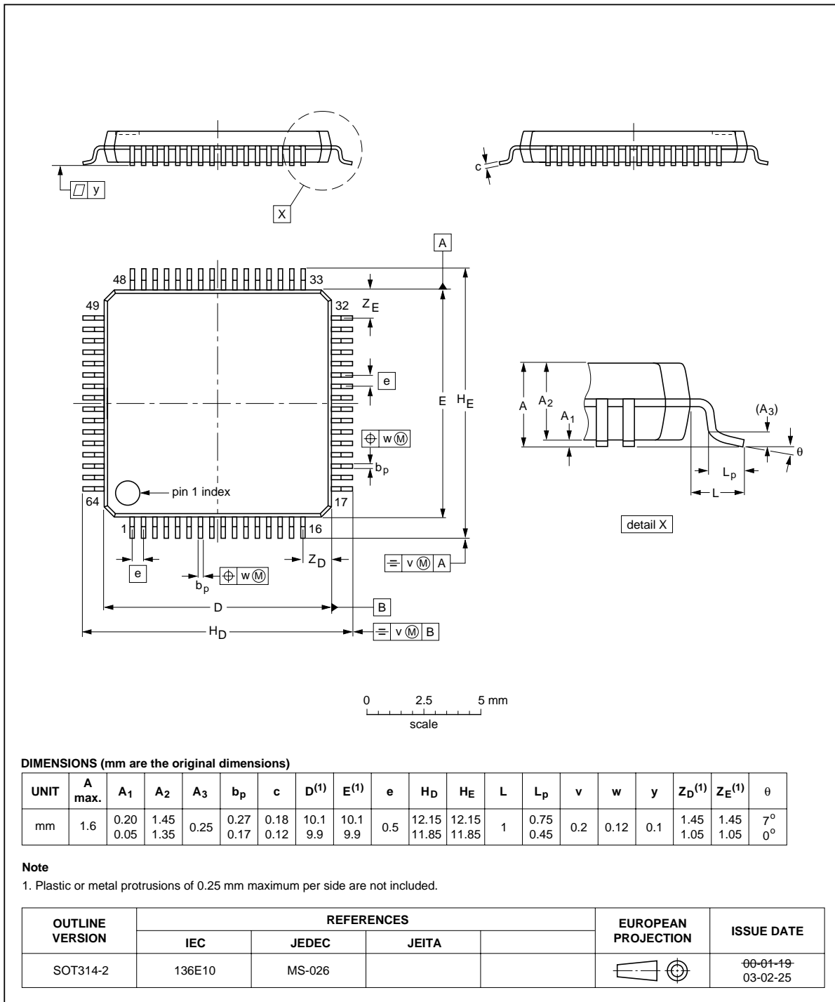
Fig 19. Package outline SOT314-2 (LQFP64)
