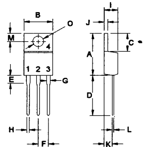
TO-220
