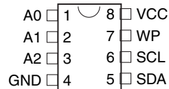
8-lead PDIP
