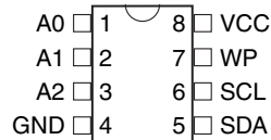
8-lead TSSOP
