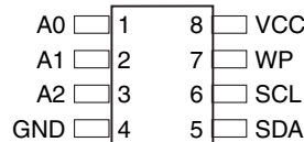
8-lead SOIC
