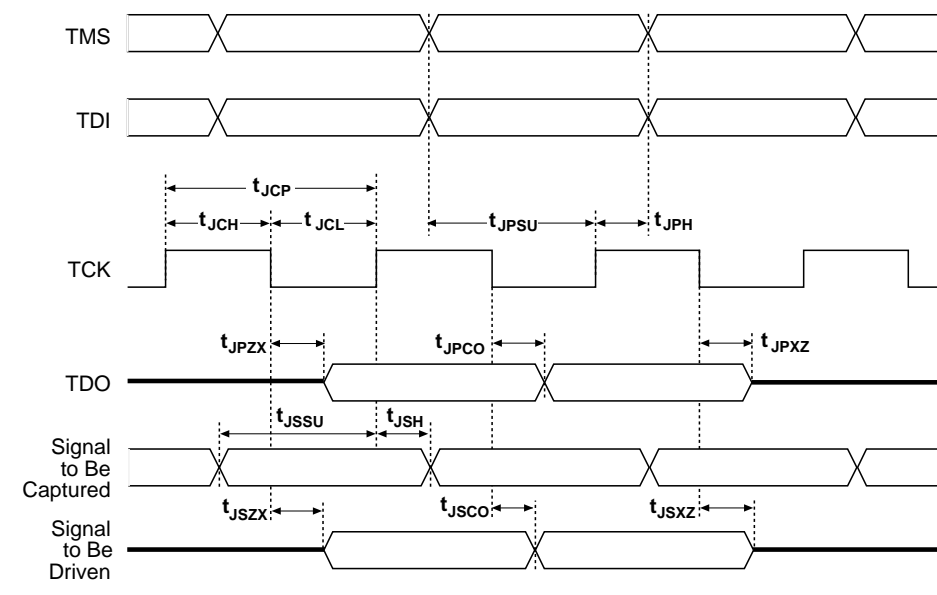
Figure 36. Cyclone JTAG Waveforms
