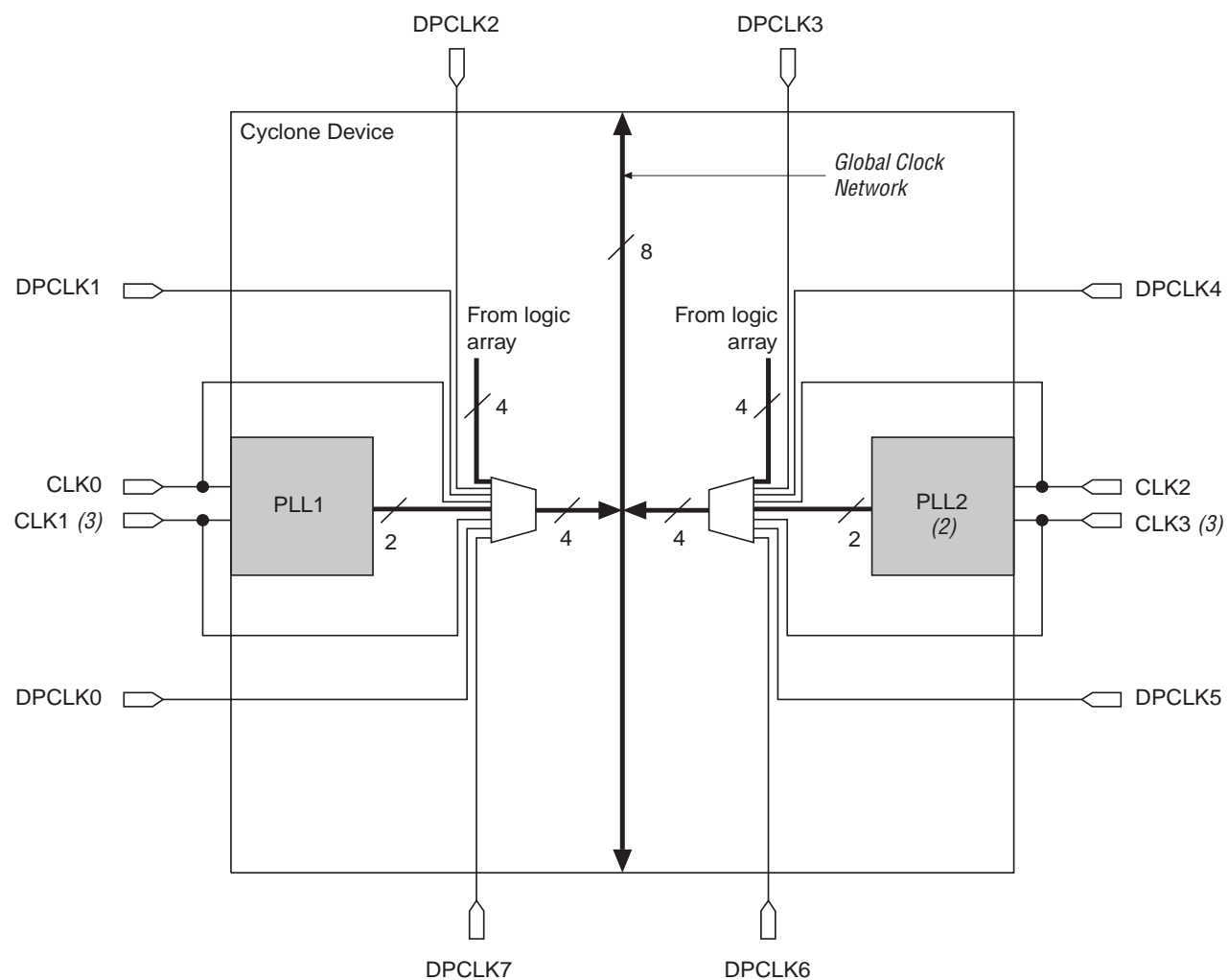
Figure 22. Global Clock Generation Note (1)
