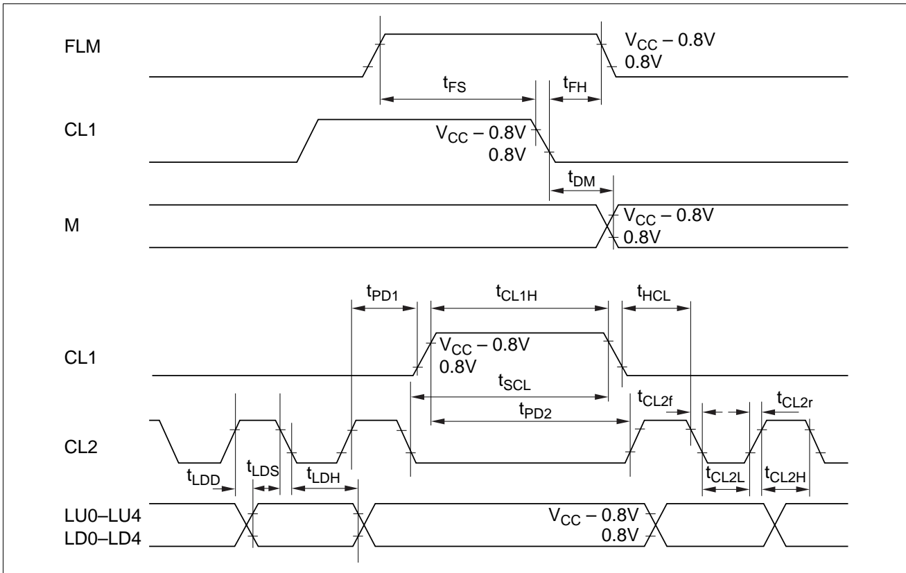
Figure 39 LCD Interface
