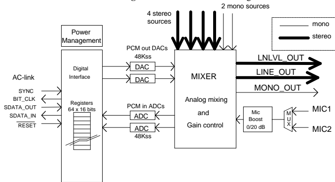
Figure 2. STAC9704 Block Diagram
