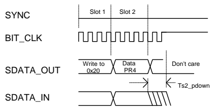
Figure 19: AC-link Low Power Mode Timing
