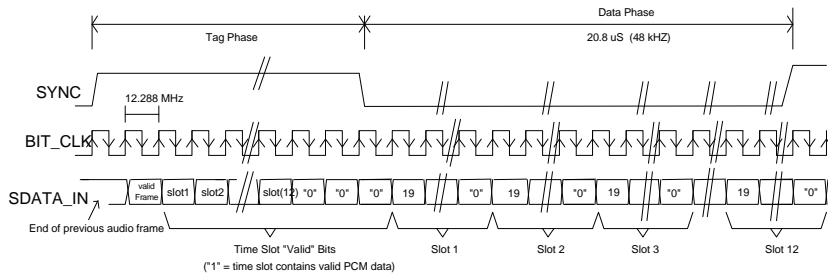
Figure 8: STAC9704/7 Audio Input Frame
