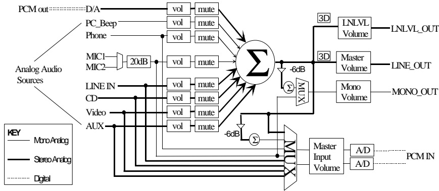
Figure 11. STAC9704/7 Mixer Functional Diagram
