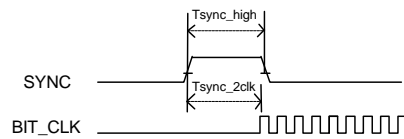
Figure 15: Warm Reset
