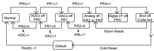
Figure 12: Example of STAC9704/7 Powerdown/Powerup flow
