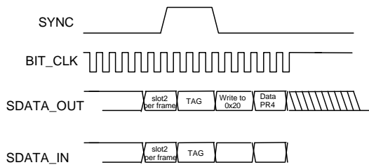
Figure 10. STAC9704/7 Powerdown Timing
