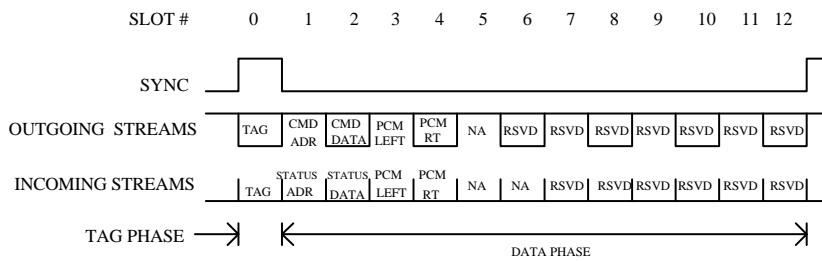
Figure 5. AC'97 Standard Bi-directional Audio Frame
