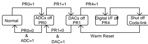
Figure 13: STAC9704/7 Powerdown/Powerup flow with analog still alive
