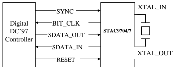
Figure 4. STAC9704/7's AC97-link to its companion controller
