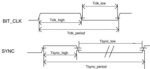
Figure 16: Clocks
