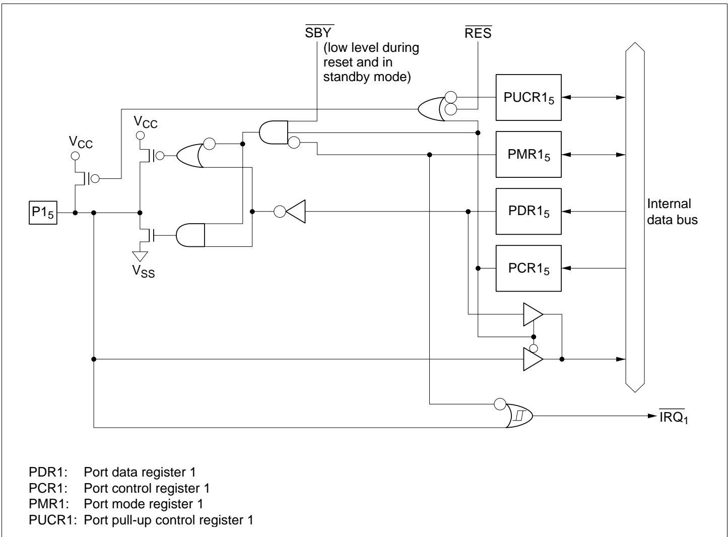
Figure C.1 (b) Port 1 Block Diagram (Pin P1 5 )
