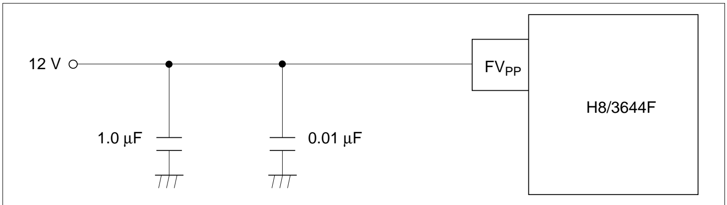
Figure 6.26 Example of V_{PP} Power Supply Circuit Design
