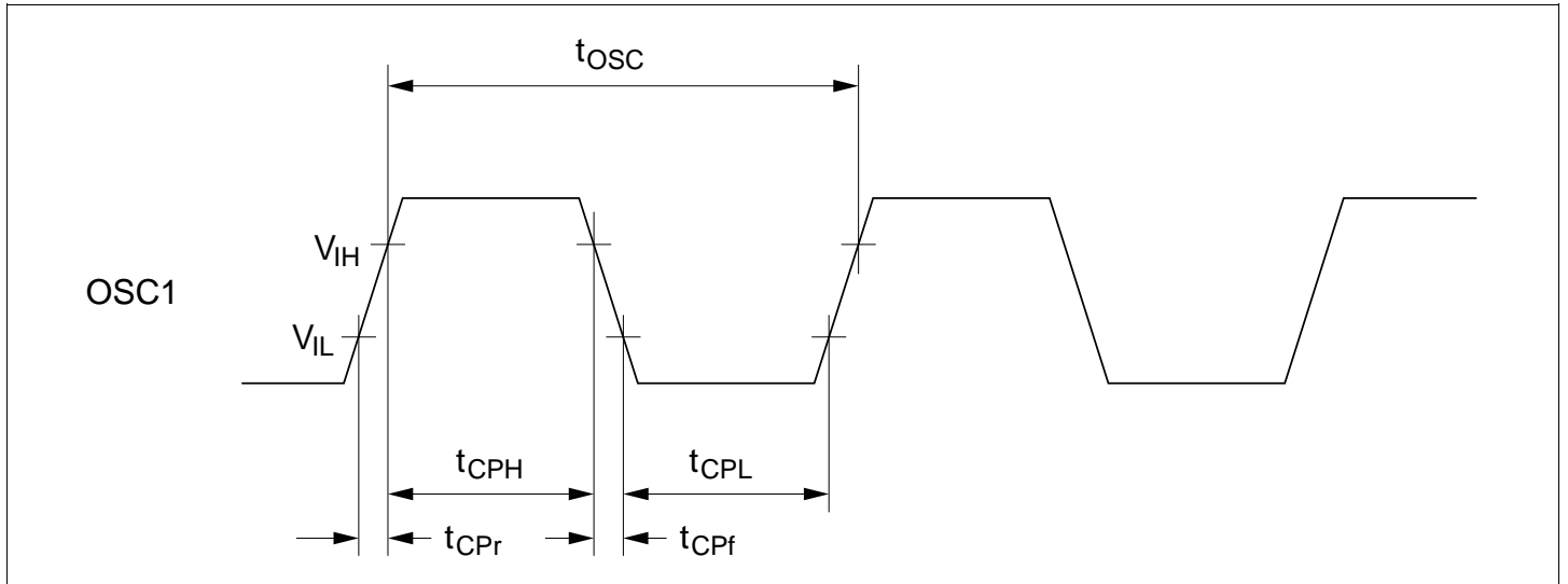
Figure 13.1 System Clock Input Timing
