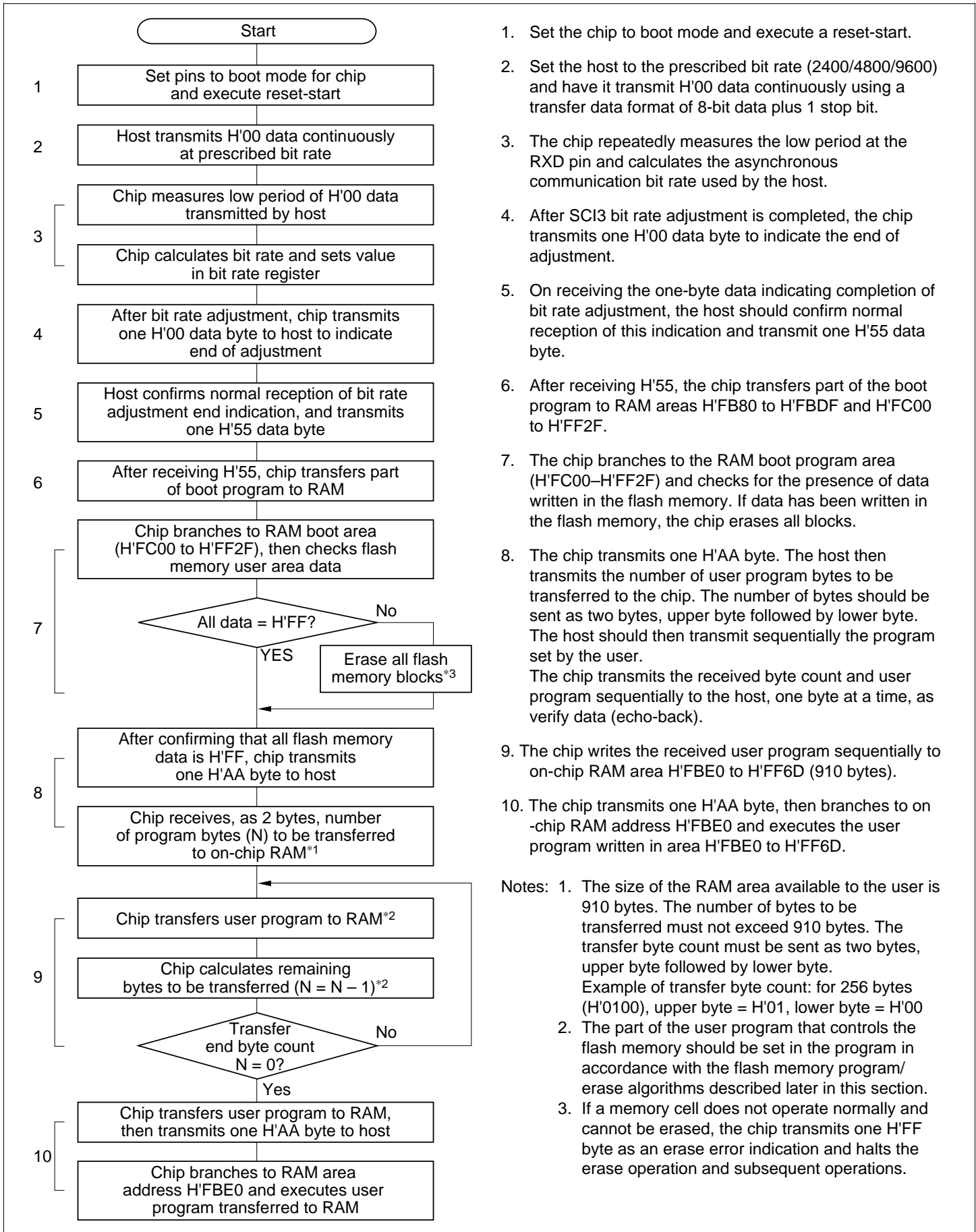
Figure 6.10 Boot Mode Operation Flowchart
