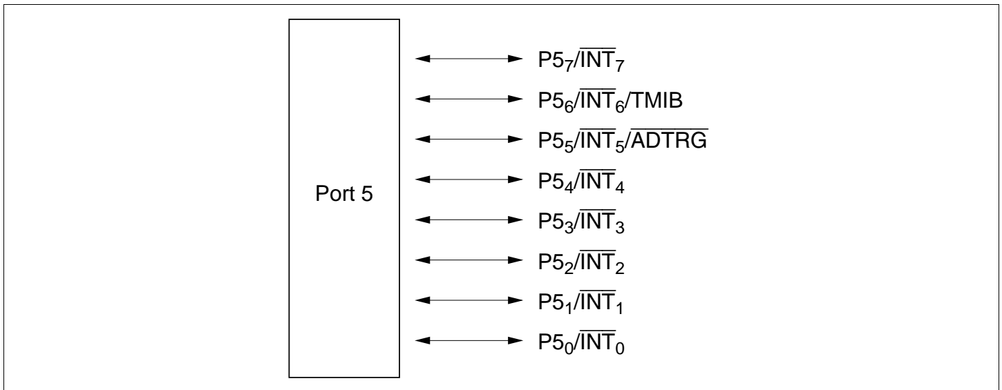
Figure 8.4 Port 5 Pin Configuration
