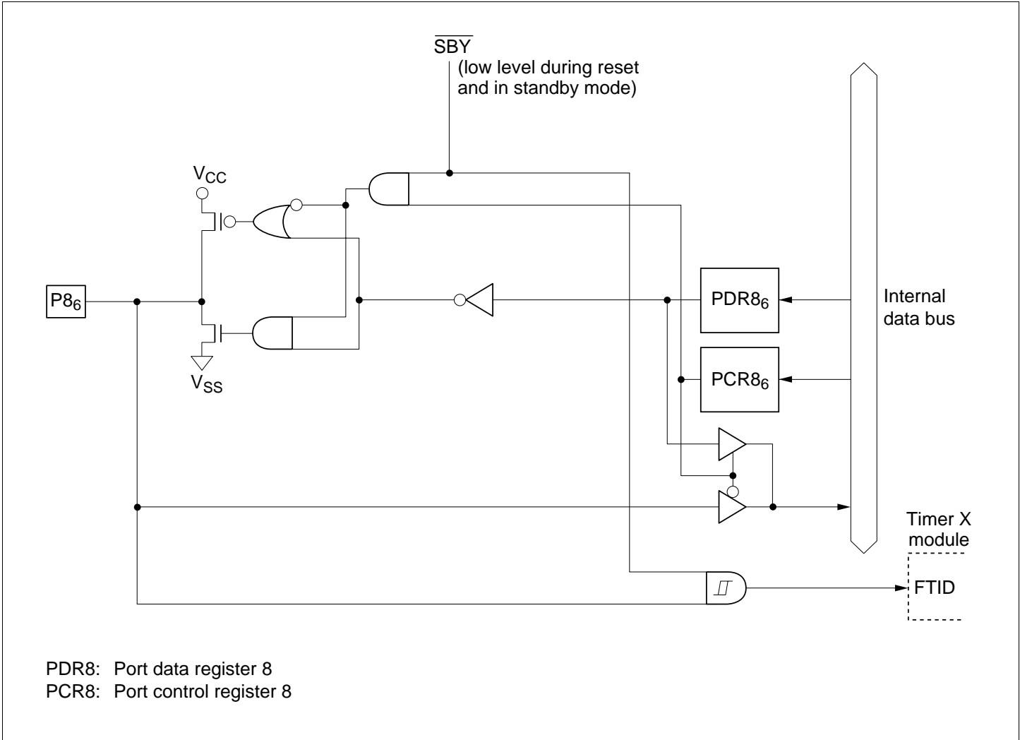
Figure C.7 (b) Port 8 Block Diagram (Pin P8 6 )
