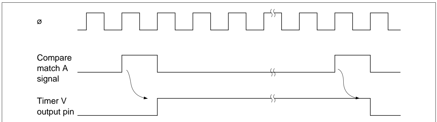
Figure 9.8 TMOV Output Timing
