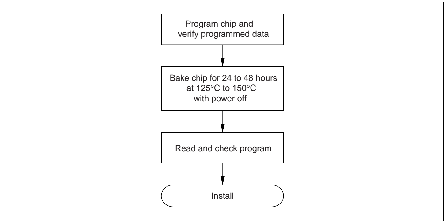
Figure 6.6 Recommended Screening Procedure
