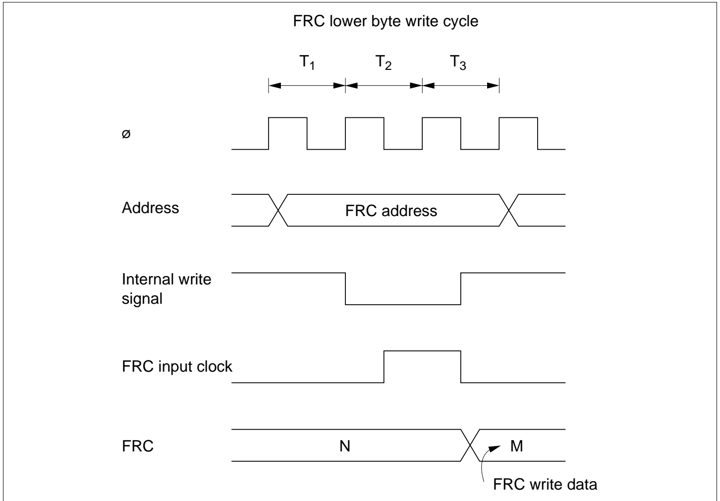
Figure 9.33 Contention between FRC Write and Increment
