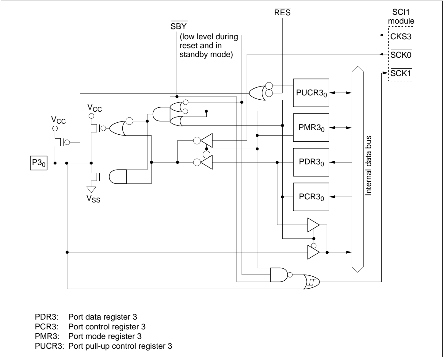
Figure C.3 (c) Port 3 Block Diagram (Pin P3 0 )
