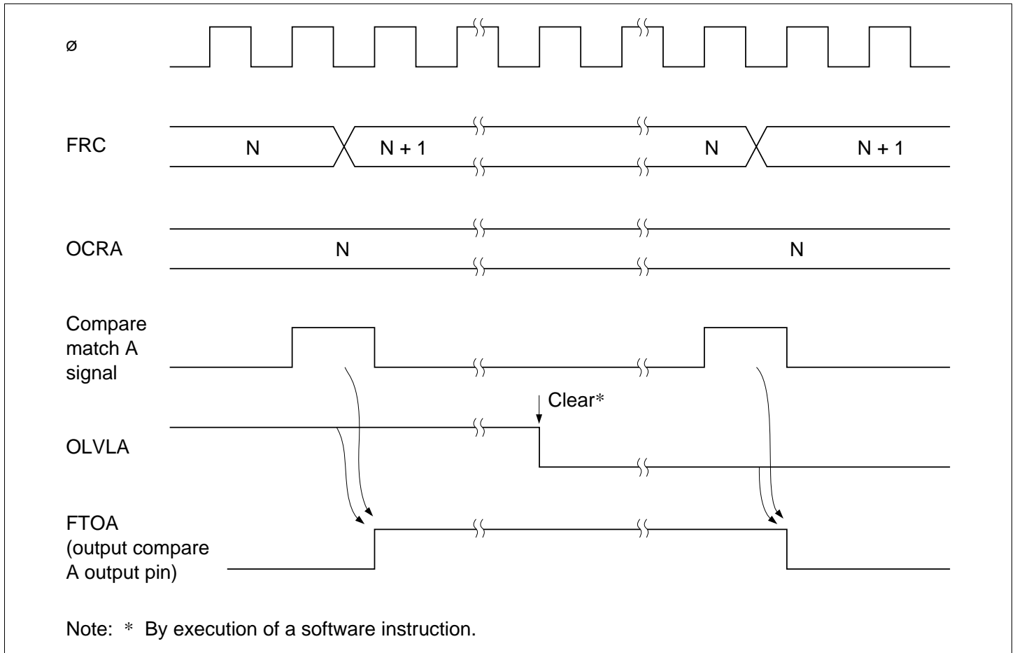
Figure 9.22 Output Compare A Output Timing
