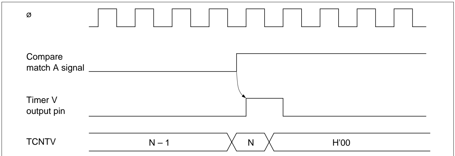
Figure 9.10 Clear Timing by TMRIV Input
