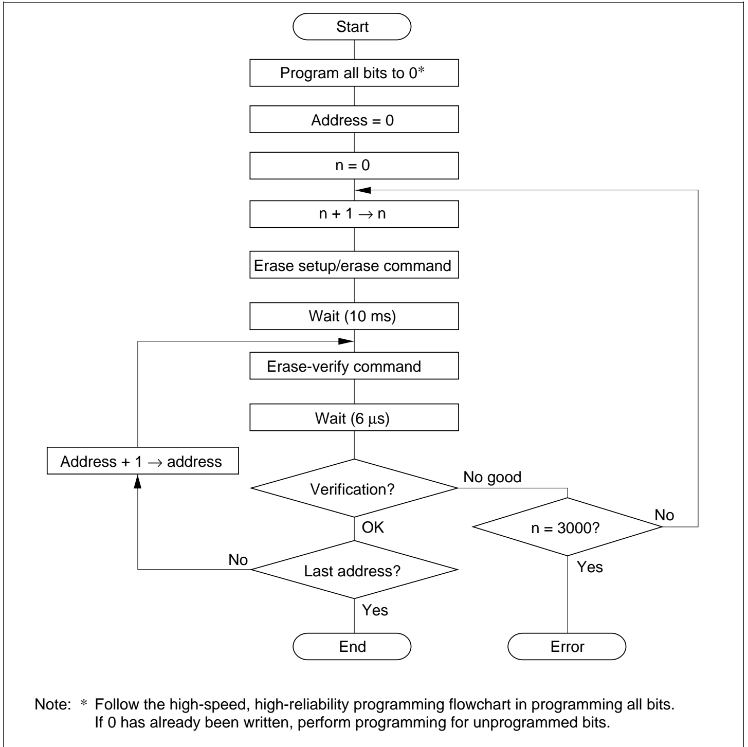
Figure 6.21 High-Speed, High-Reliability Erasing
