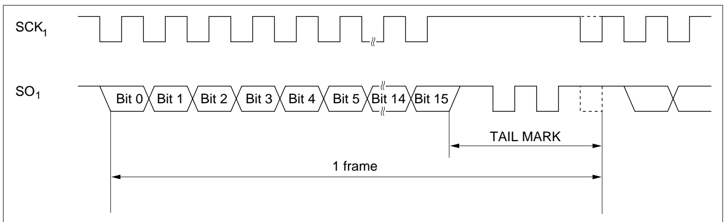
Figure 10.4 Transfer Format (When SNC1 = 0, SNC0 = 1, MRKON = 1)
