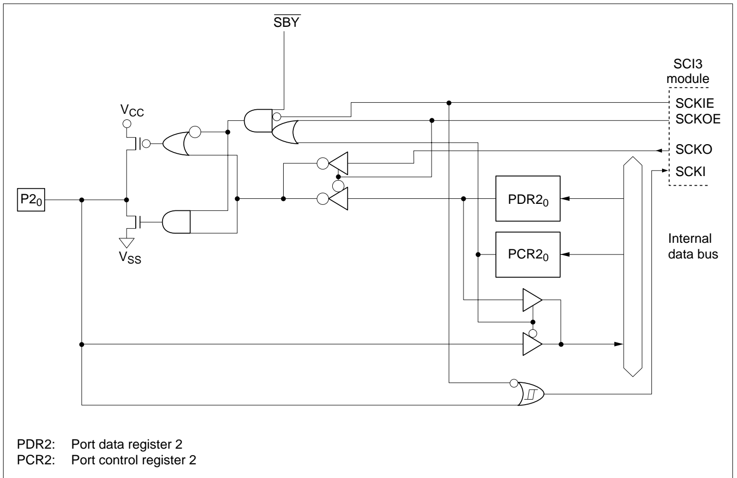
Figure C.2 (c) Port 2 Block Diagram (Pin P2 0 )
