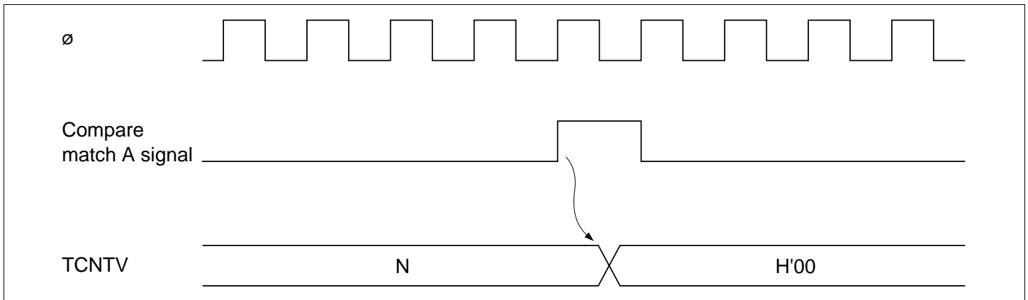
Figure 9.9 Clear Timing by Compare Match
