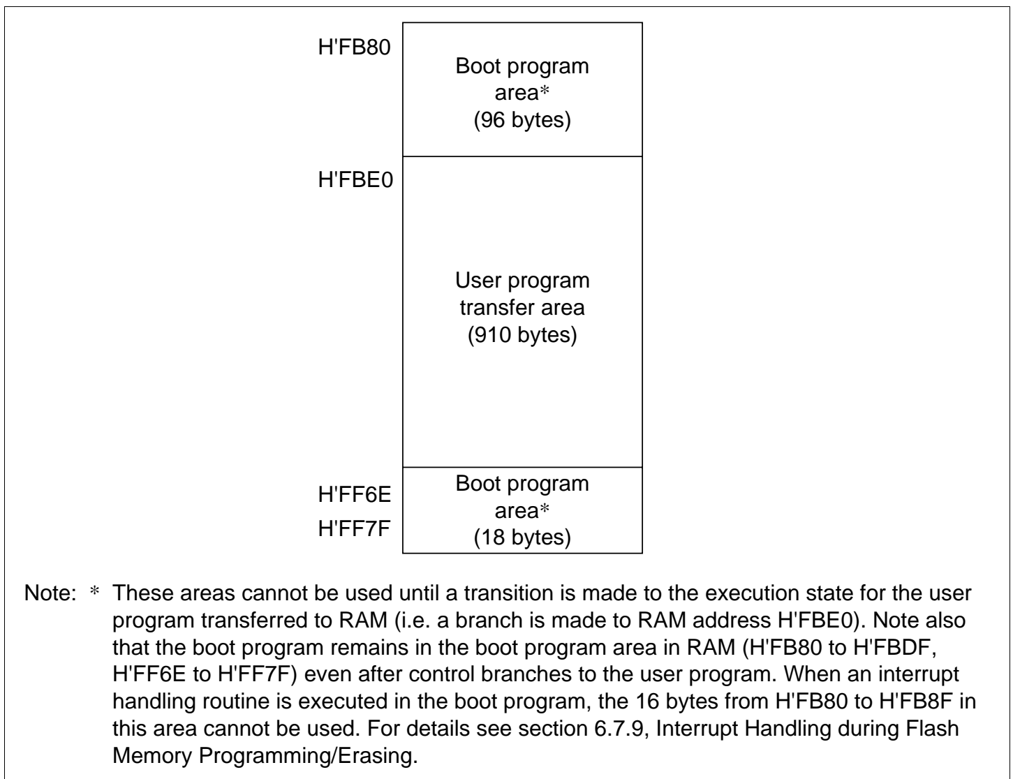
Figure 6.12 RAM Areas in Boot Mode
