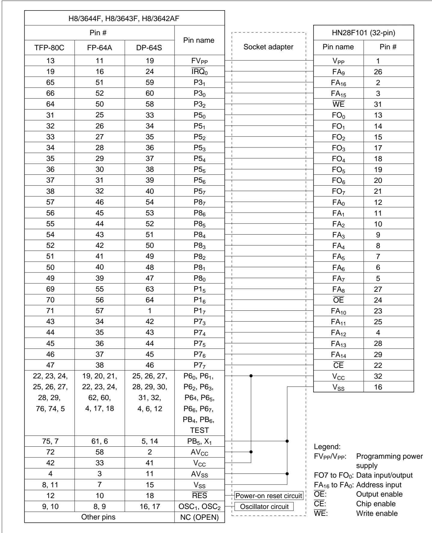
Figure 6.19 Socket Adapter Pin Correspondence (F-ZTAT)
