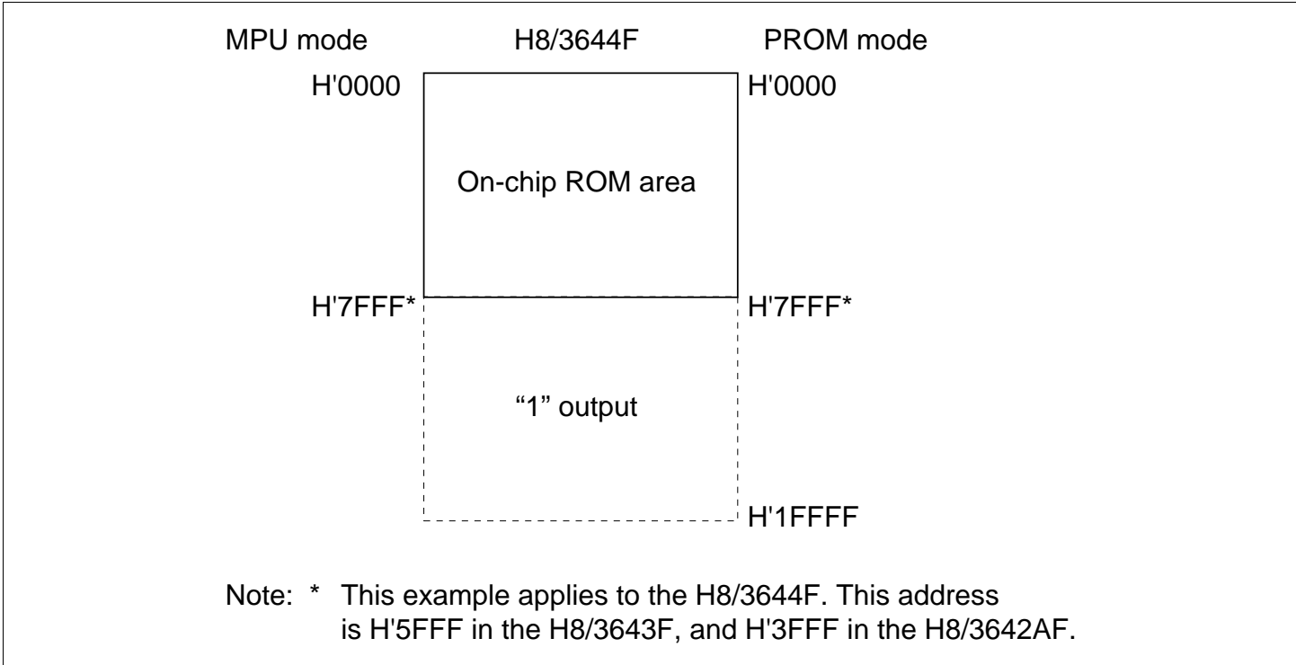
Figure 6.18 Memory Map in PROM Mode
