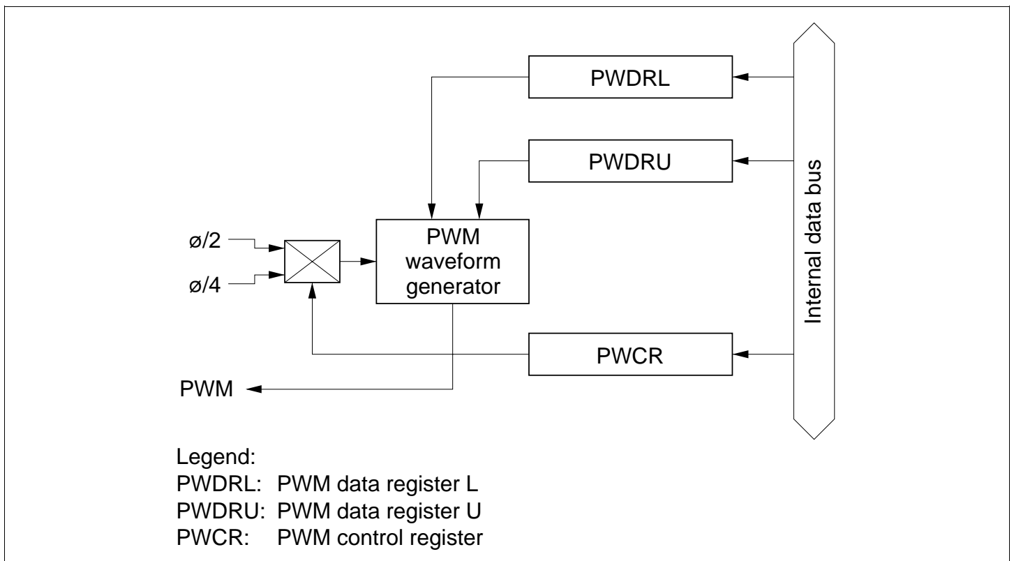
Figure 11.1 Block Diagram of the 14-Bit PWM
