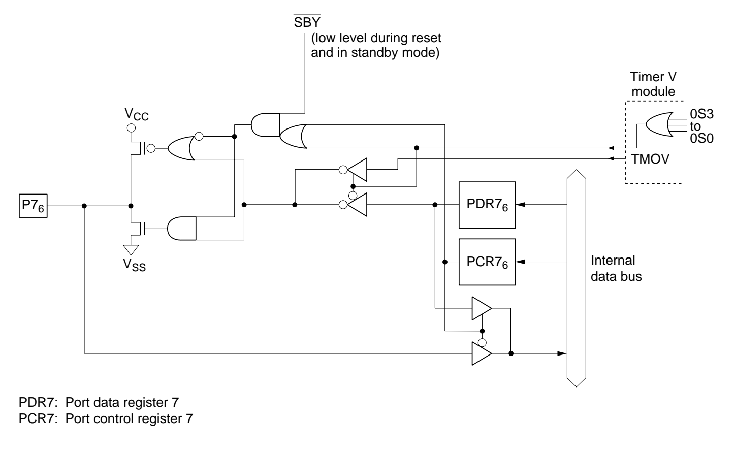
Figure C.6 (b) Port 7 Block Diagram (Pin P7 6 )
