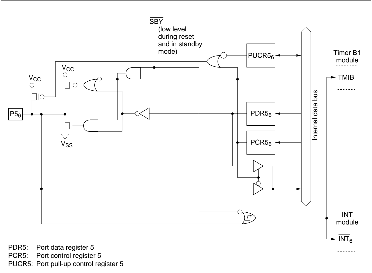
Figure C.4 (b) Port 5 Block Diagram (Pin P5 6 )
