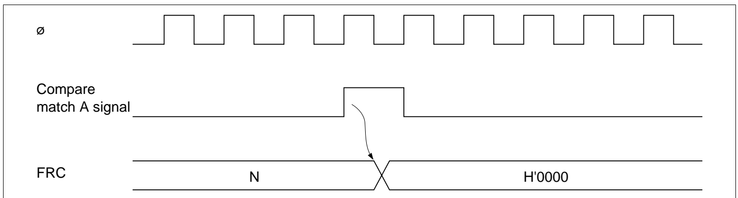
Figure 9.23 Clear Timing by Compare Match A
