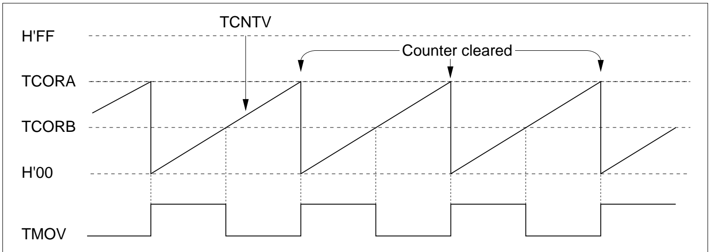
Figure 9.11 Pulse Output Example
