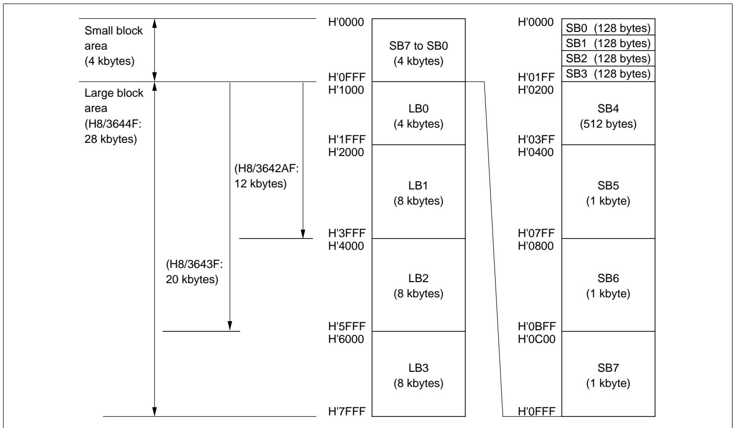
Figure 6.8 Erase Block Map
