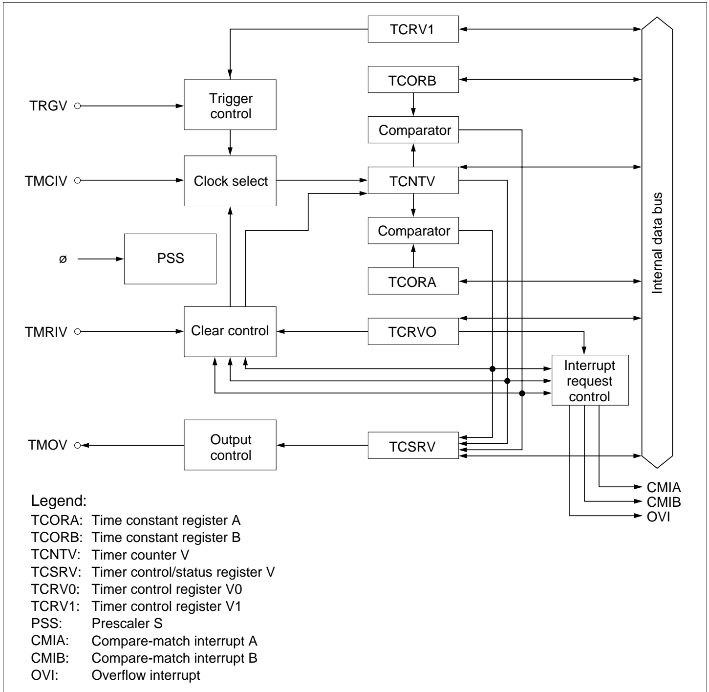
Figure 9.3 Block Diagram of Timer V
