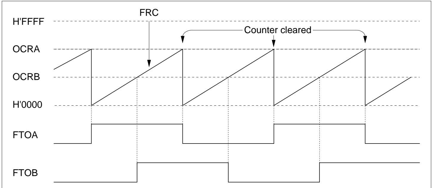
Figure 9.31 Pulse Output Example
