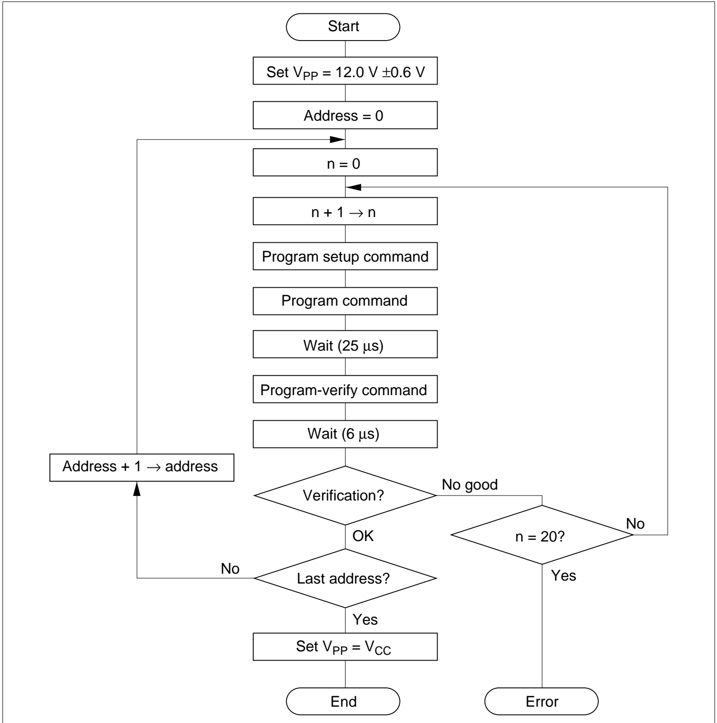
Figure 6.20 High-Speed, High-Reliability Programming
