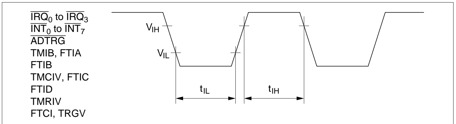
Figure 13.3 Input Timing
