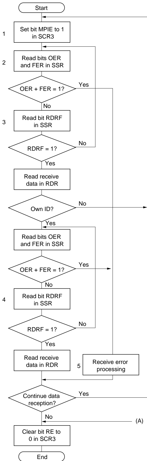
Figure 10.24 Example of Multiprocessor Data Reception Flowchart
