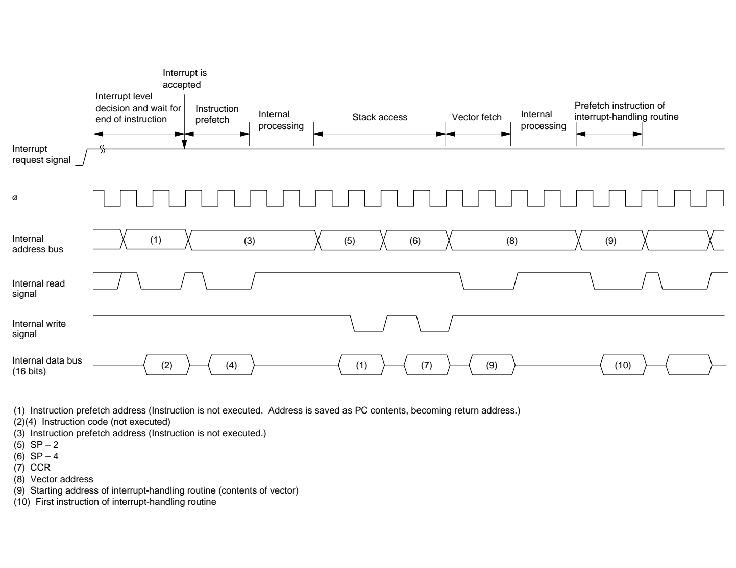
Figure 3.5 Interrupt Sequence
