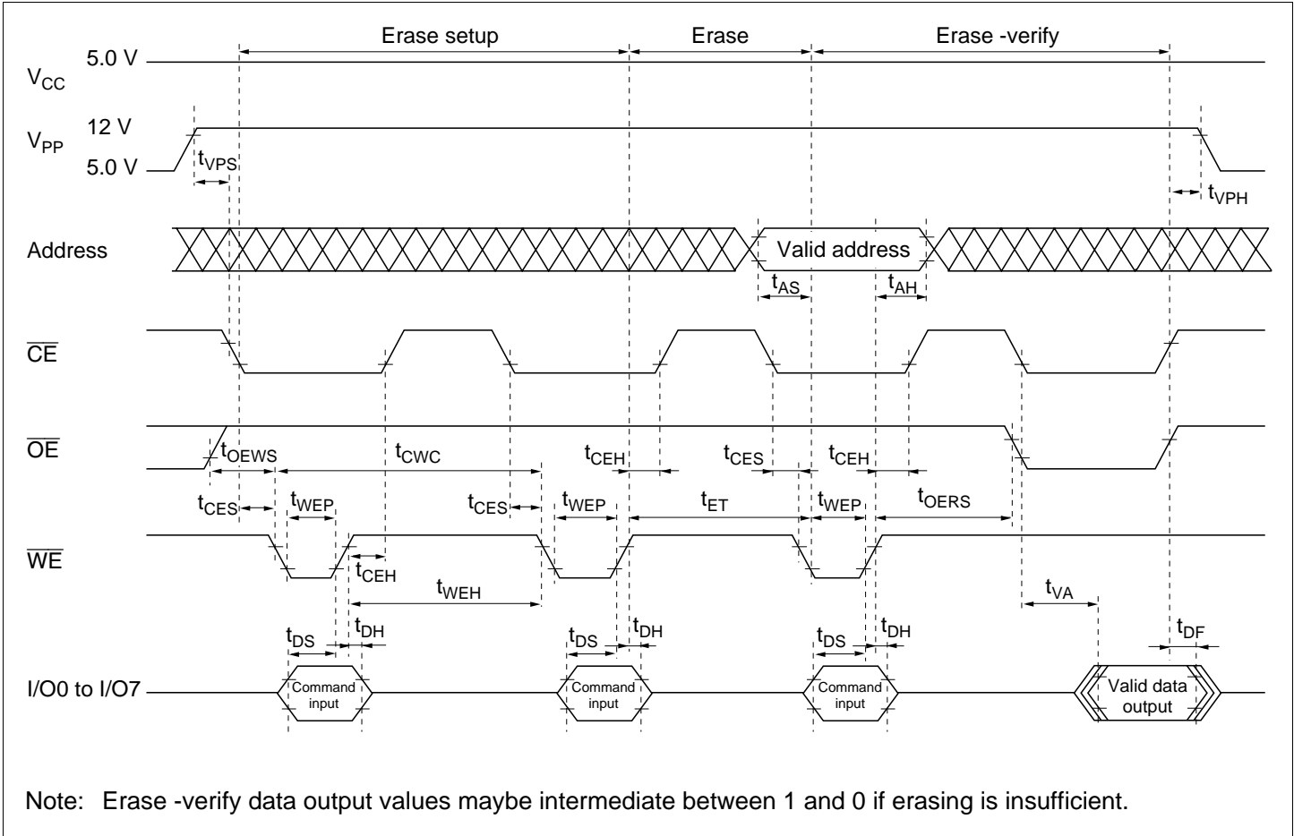
Figure 6.24 Erase Timing
