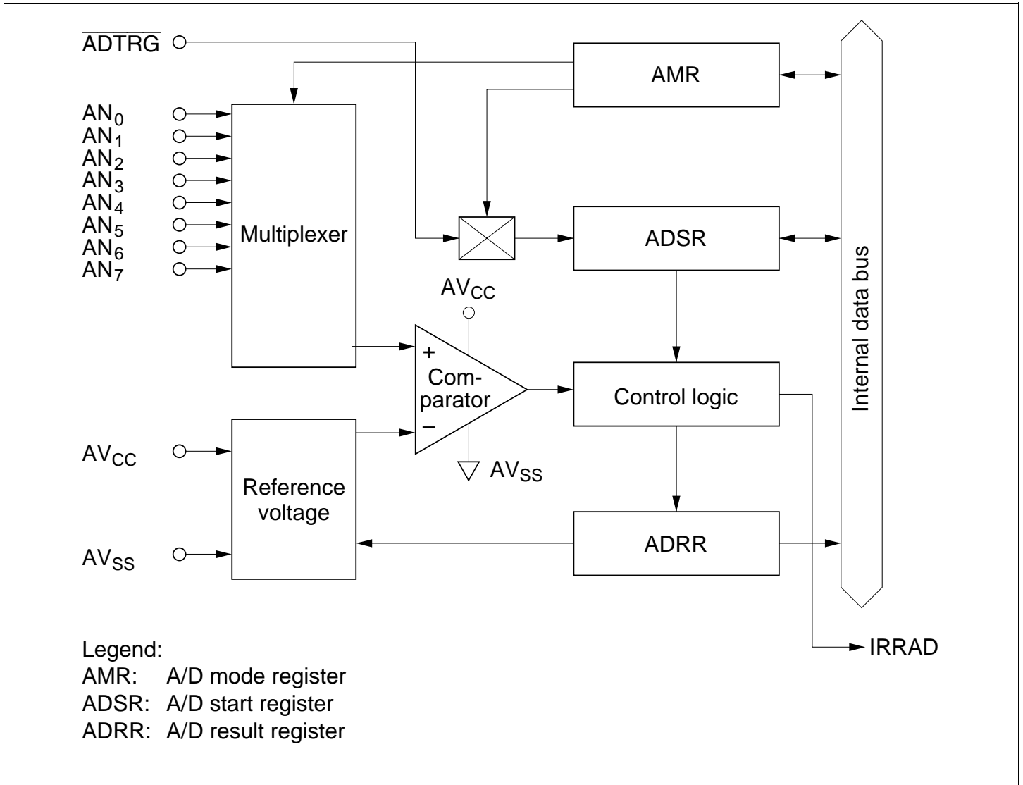
Figure 12.1 Block Diagram of the A/D Converter
