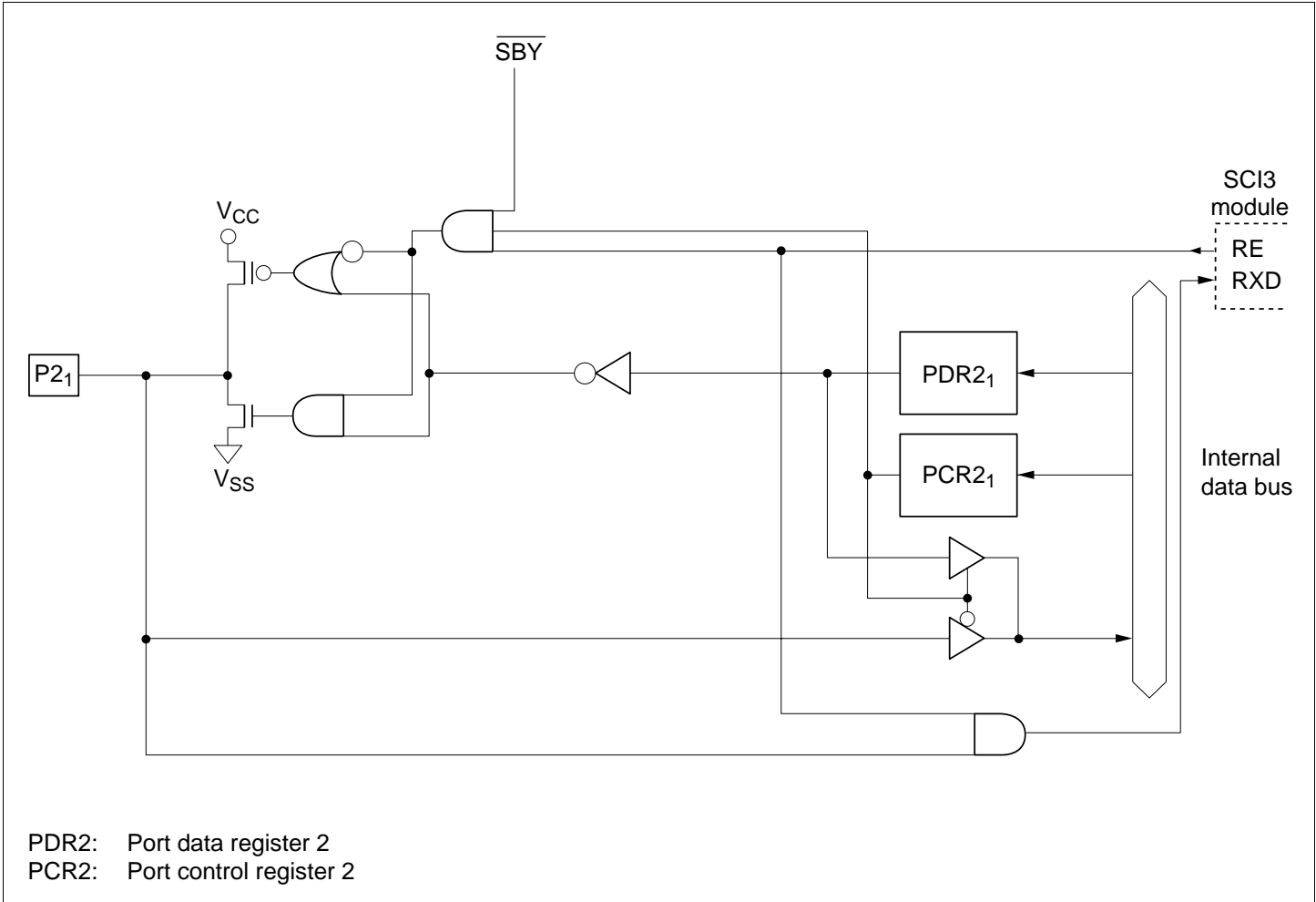
Figure C.2 (b) Port 2 Block Diagram (Pin P2 1 )
