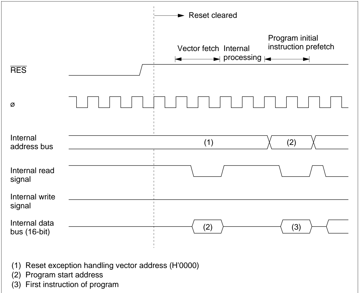
Figure 3.1 Reset Sequence
