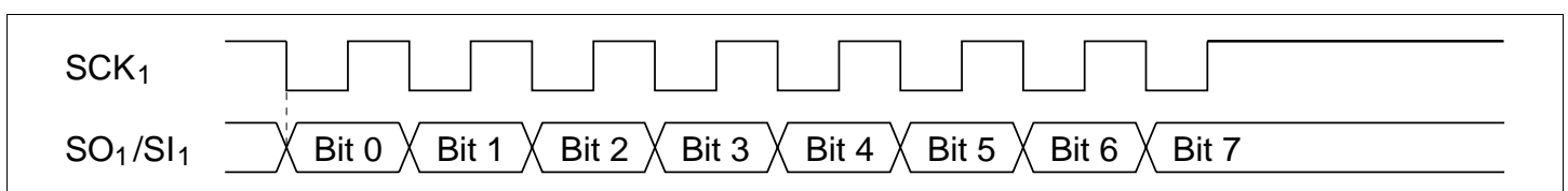
Figure 10.2 Transfer Format
