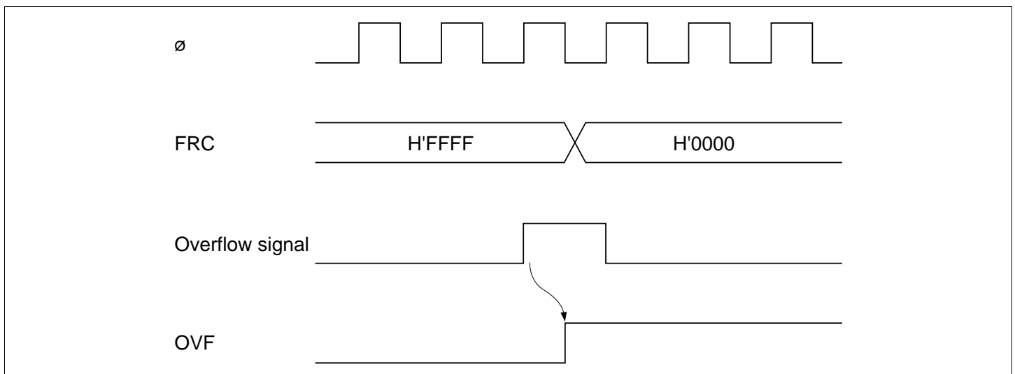
Figure 9.30 OVF Set Timing
