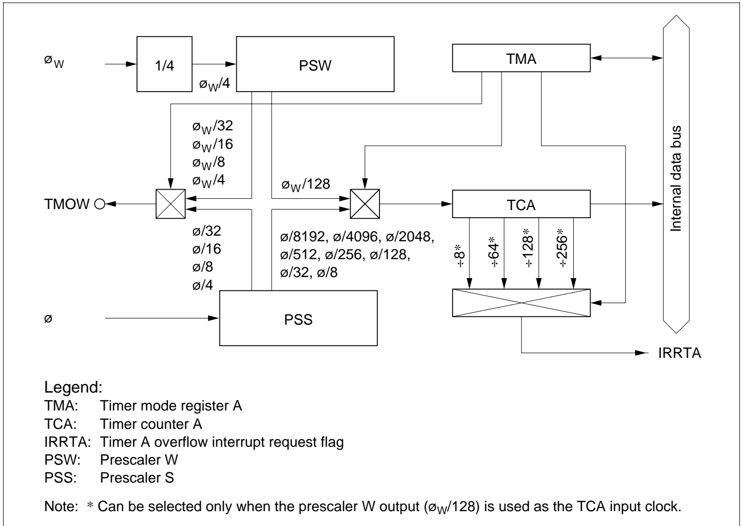
Figure 9.1 Block Diagram of Timer A
