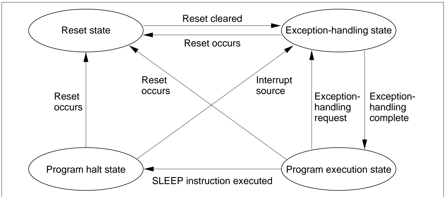
Figure 2.15 State Transitions
