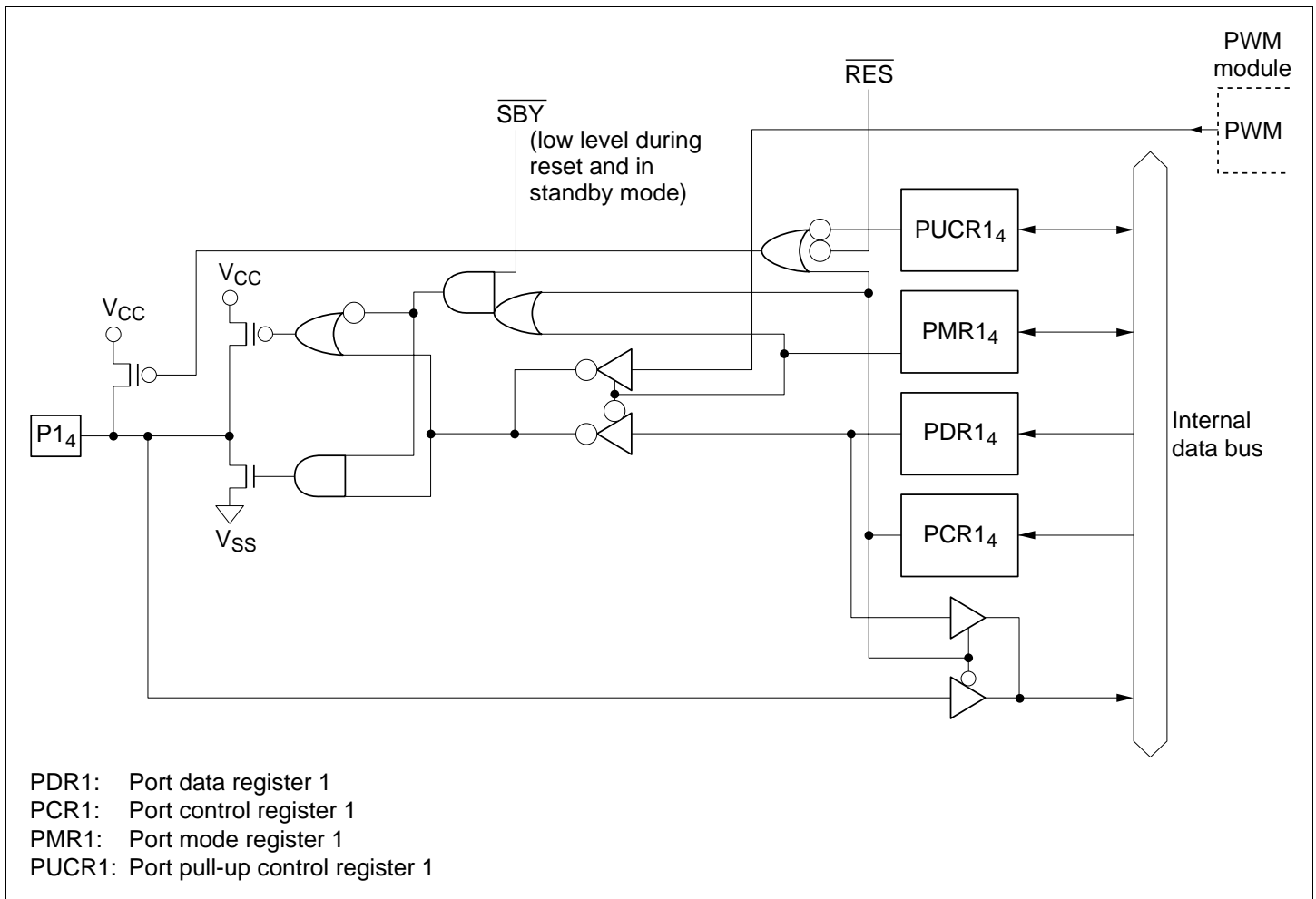
Figure C.1 (c) Port 1 Block Diagram (Pin P1 4 )
