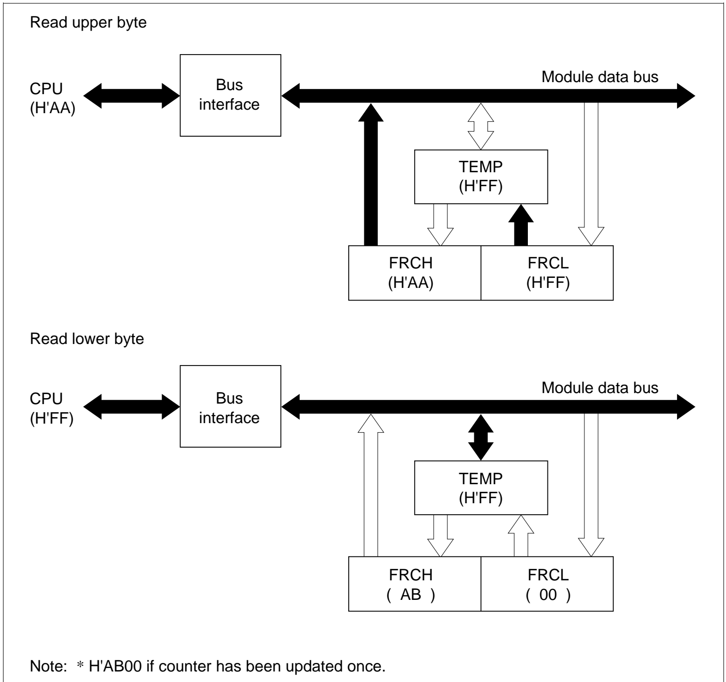
Figure 9.19 Read Access to FRC (FRC → CPU)
