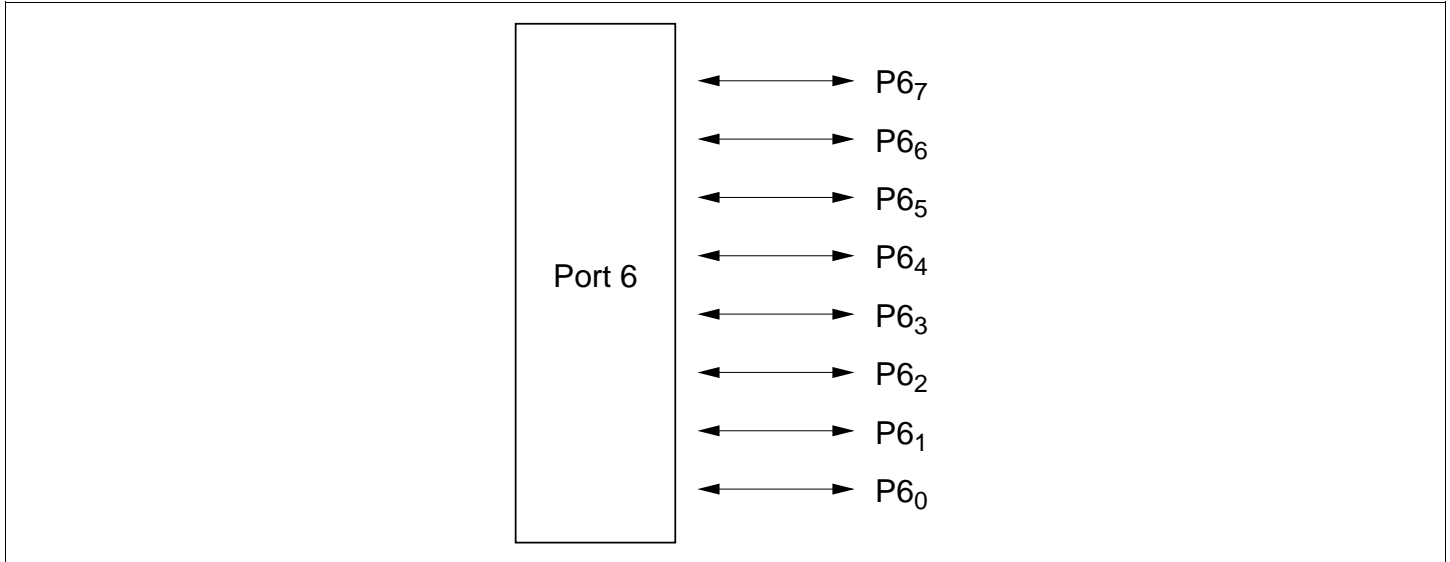
Figure 8.5 Port 6 Pin Configuration
