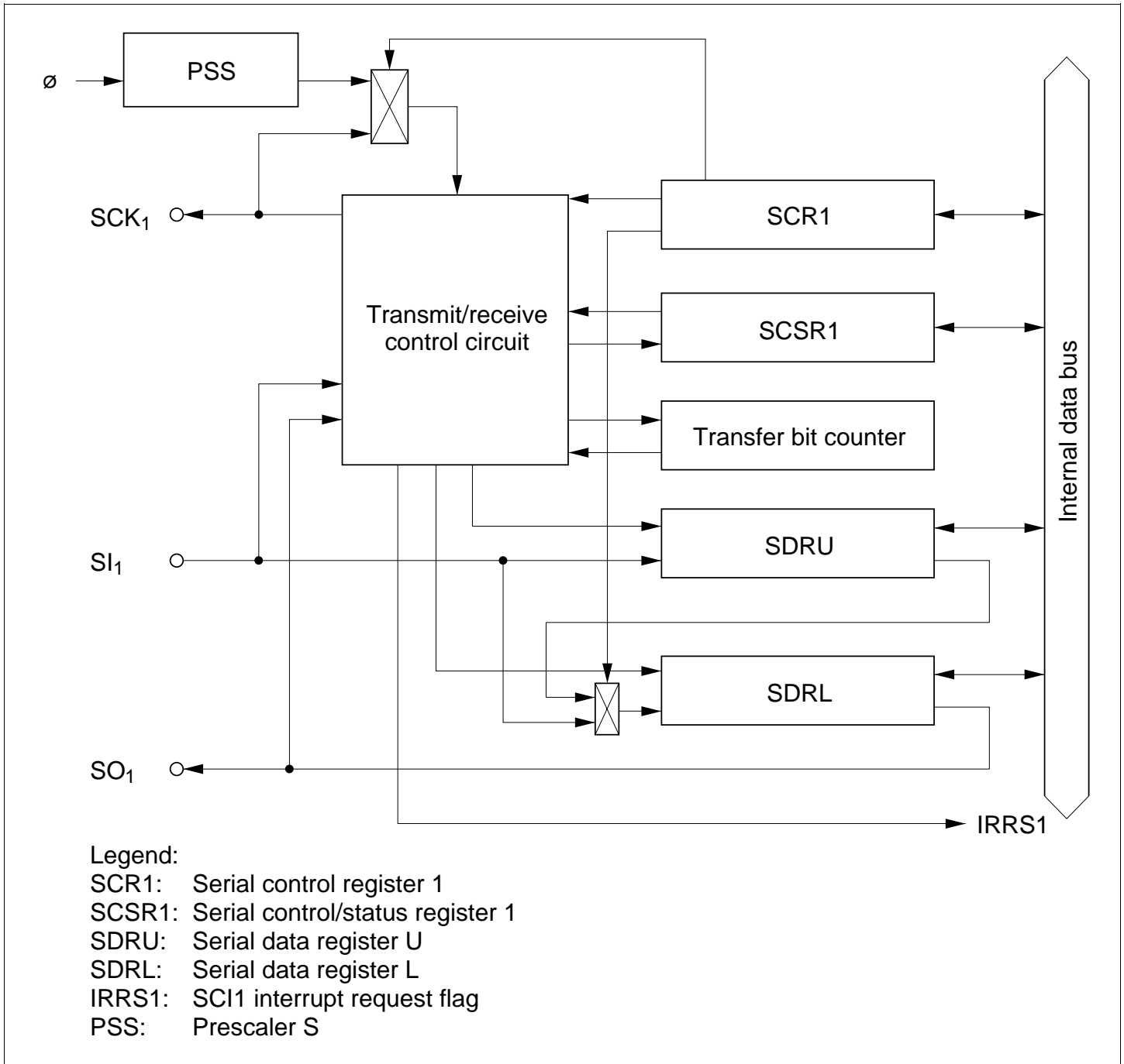
Figure 10.1 SCI1 Block Diagram
