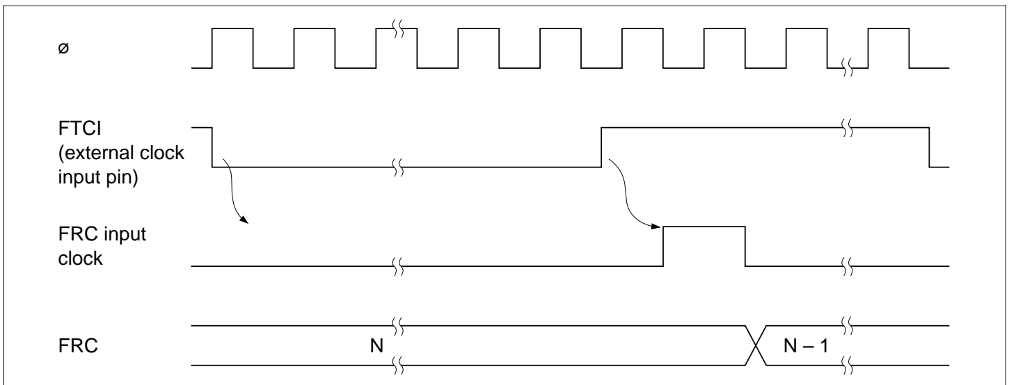
Figure 9.21 Increment Timing with External Clock
