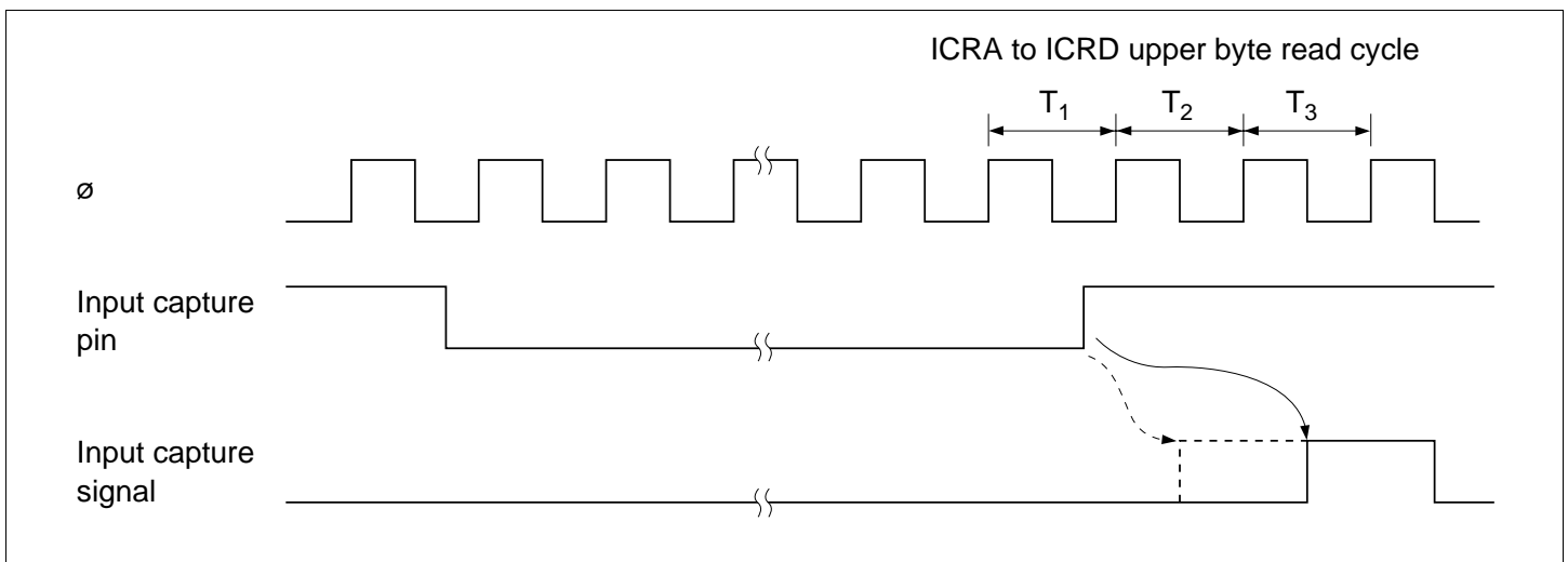
Figure 9.25 Input Capture Signal Timing (during ICRA to ICRD Read)
