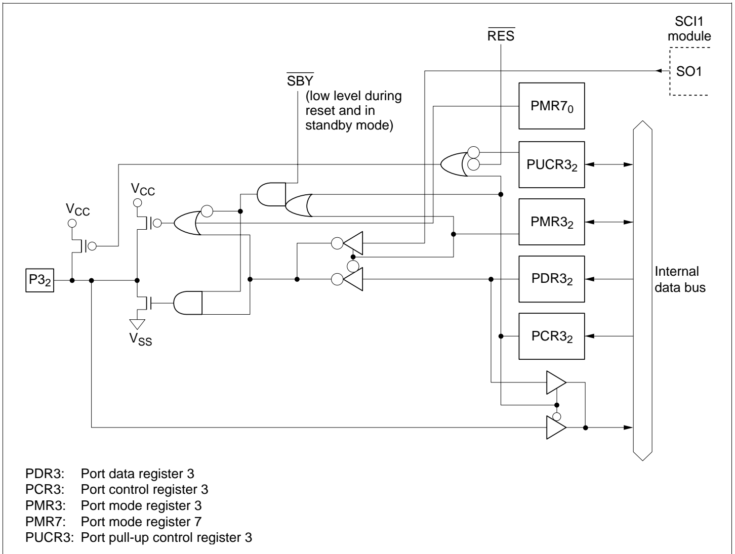
Figure C.3 (a) Port 3 Block Diagram (Pin P3 2 )
