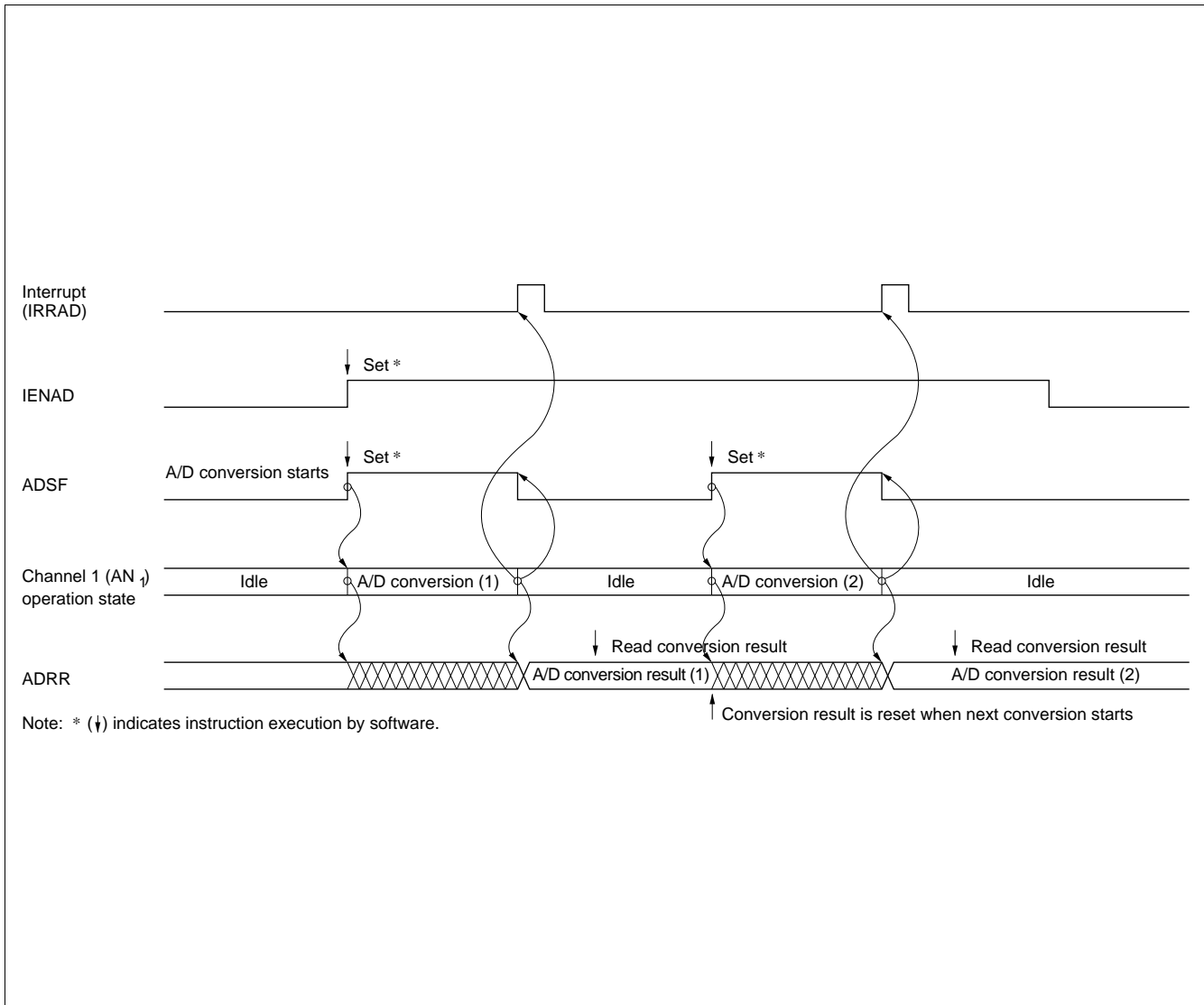
Figure 12.3 Typical A/D Converter Operation Timing
