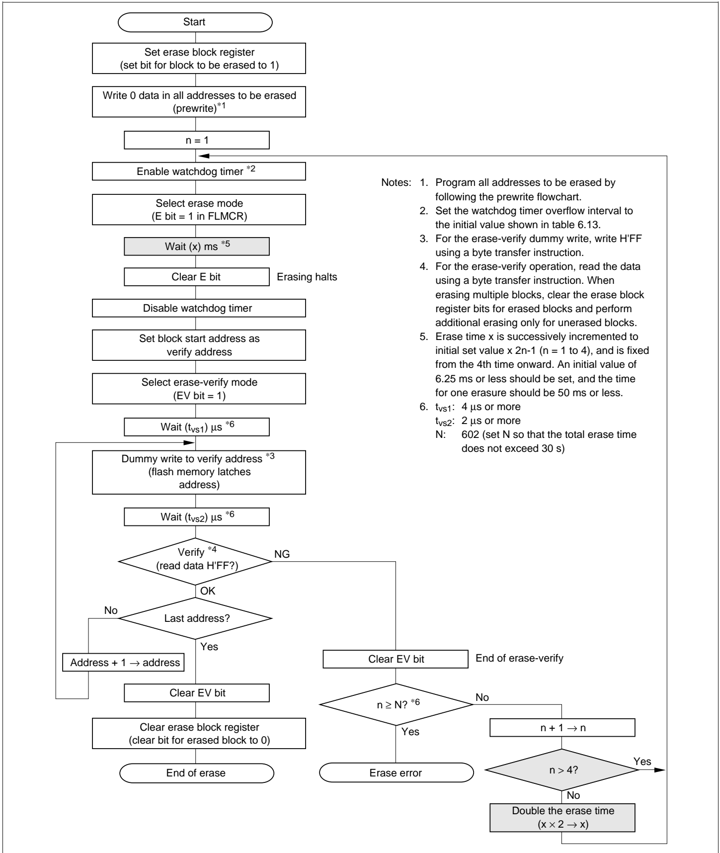
Figure 6.15 Erase Flowchart
