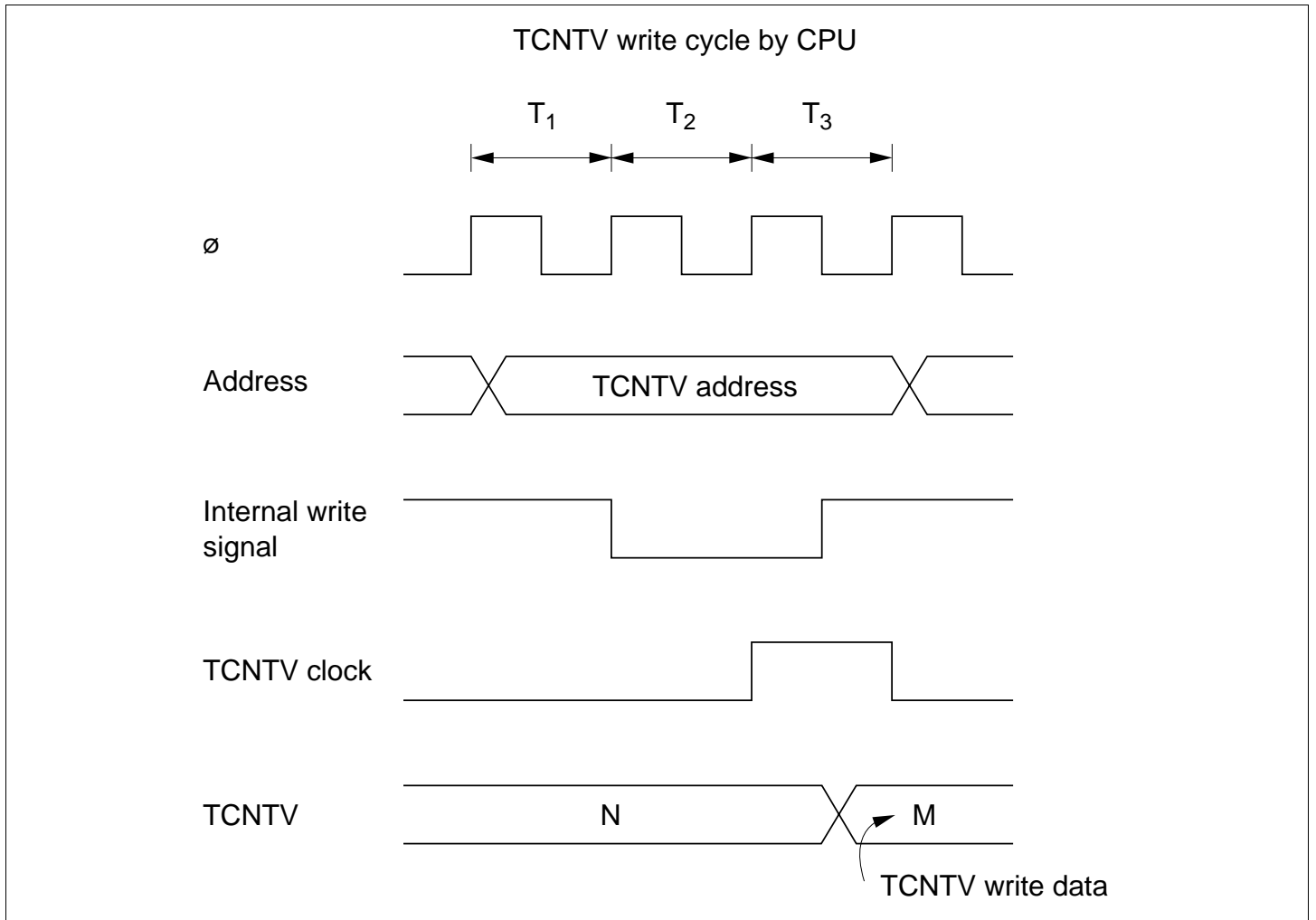
Figure 9.14 Contention between TCNTV Write and Increment
