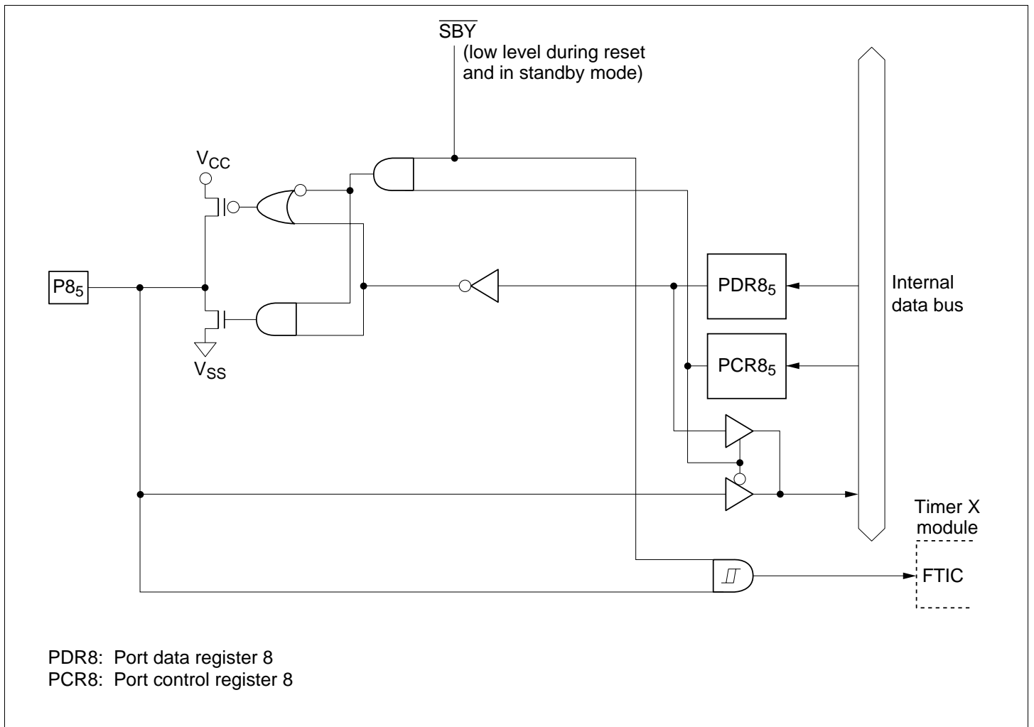
Figure C.7 (c) Port 8 Block Diagram (Pin P8 5 )
