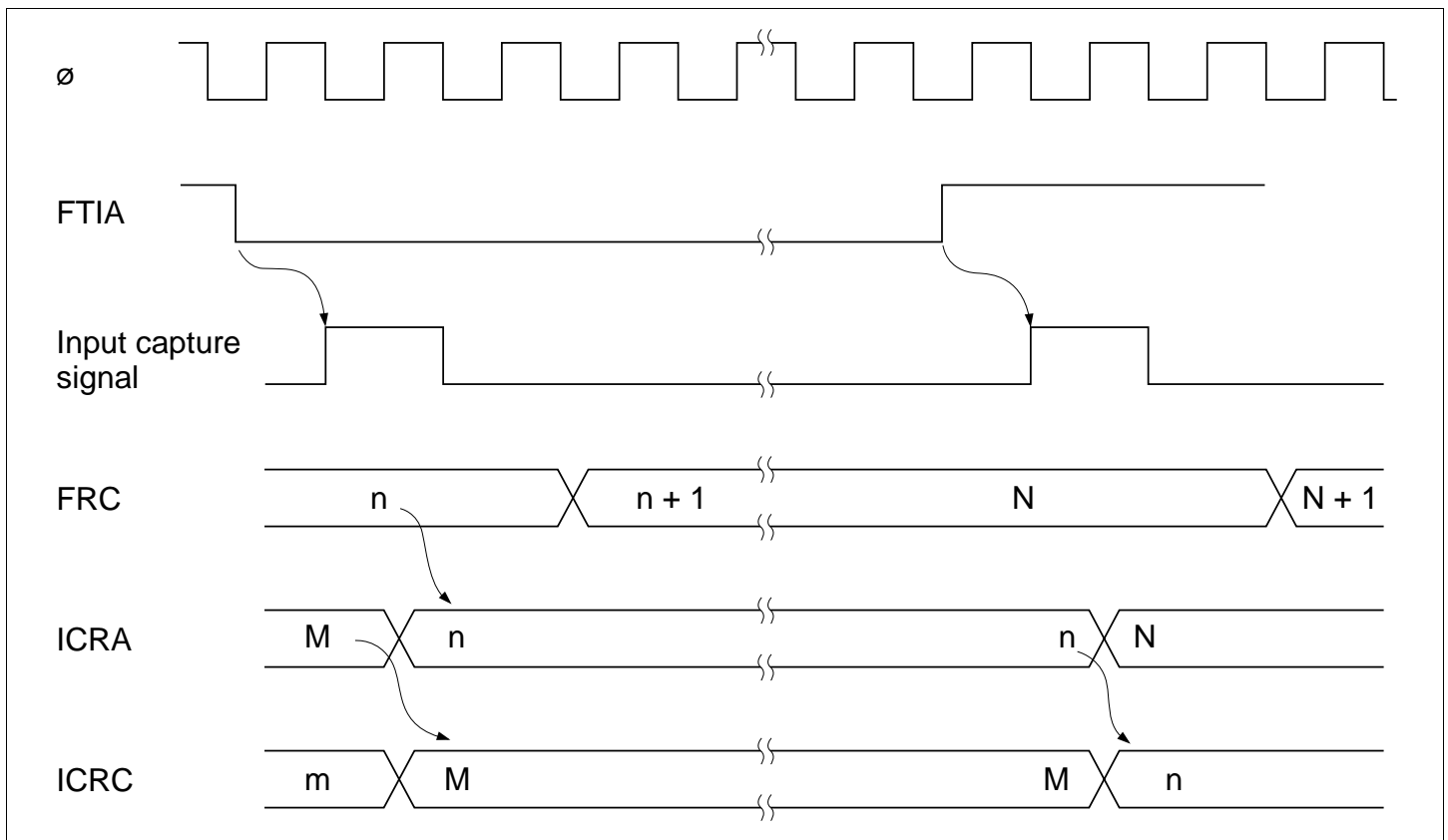
Figure 9.26 Buffered Input Capture Timing (Normal Case)
