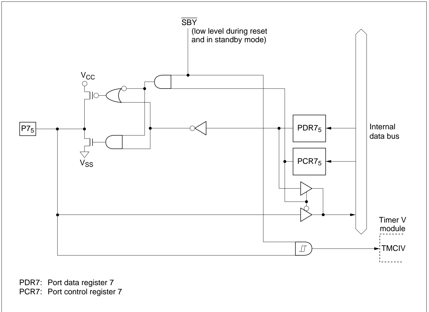
Figure C.6 (c) Port 7 Block Diagram (Pin P7 5 )
