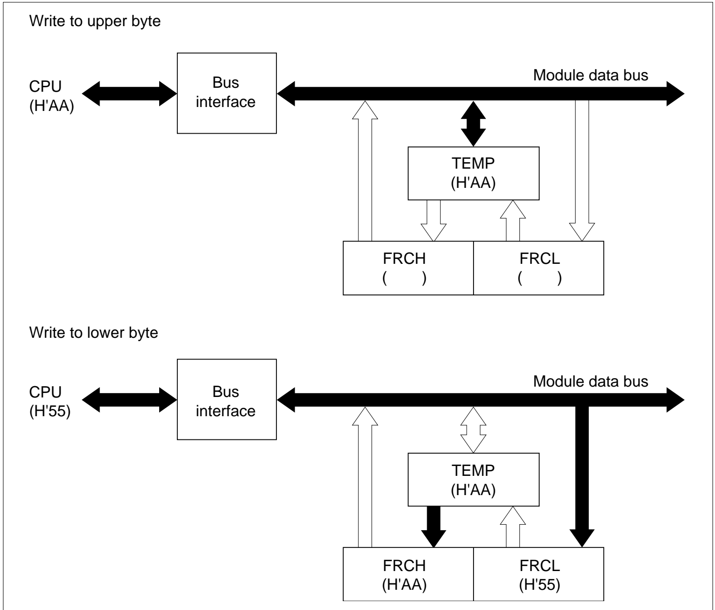
Figure 9.18 Write Access to FRC (CPU → FRC)
