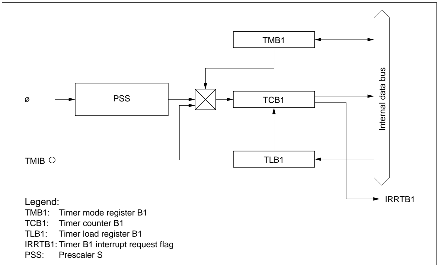
Figure 9.2 Block Diagram of Timer B1
