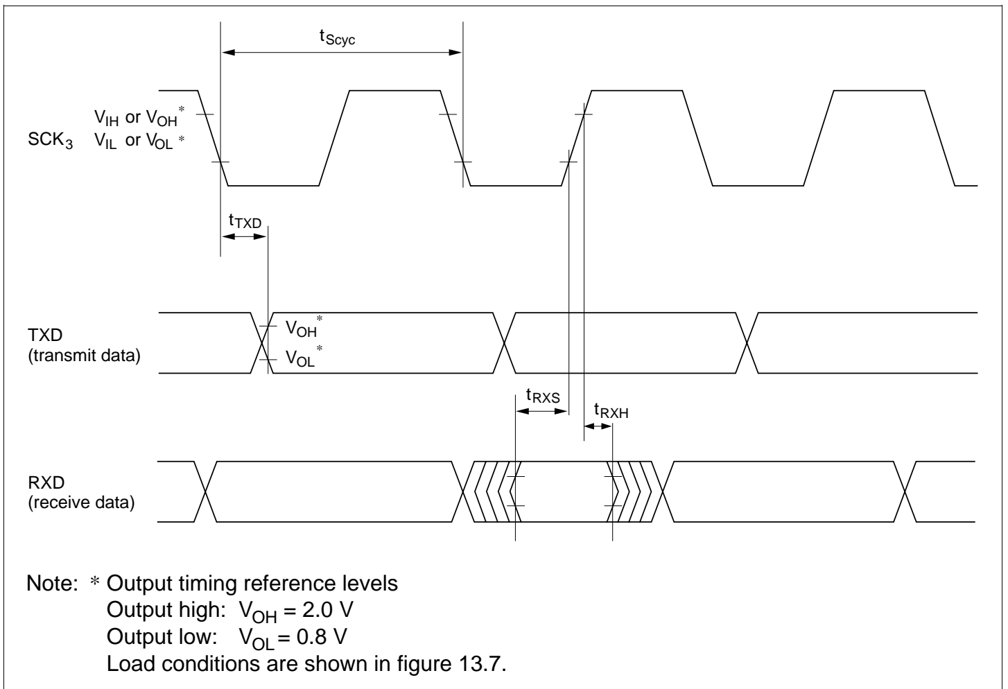
Figure 13.6 Serial Interface 3 Synchronous Mode Input/Output Timing
