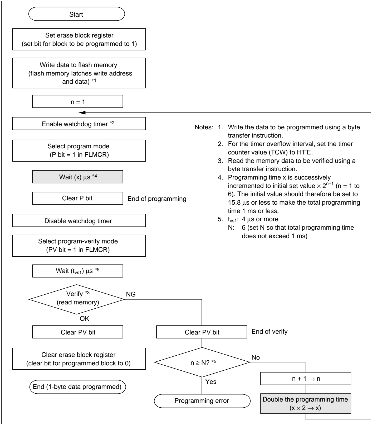
Figure 6.14 Programming Flowchart
