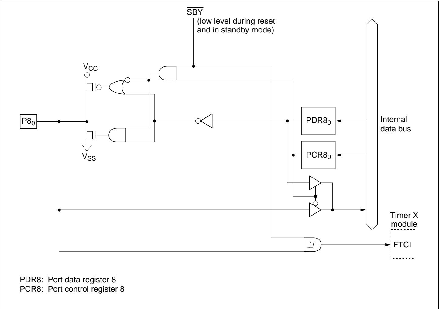
Figure C.7 (h) Port 8 Block Diagram (Pin P8 0 )
