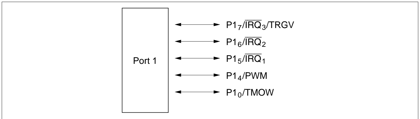
Figure 8.1 Port 1 Pin Configuration
