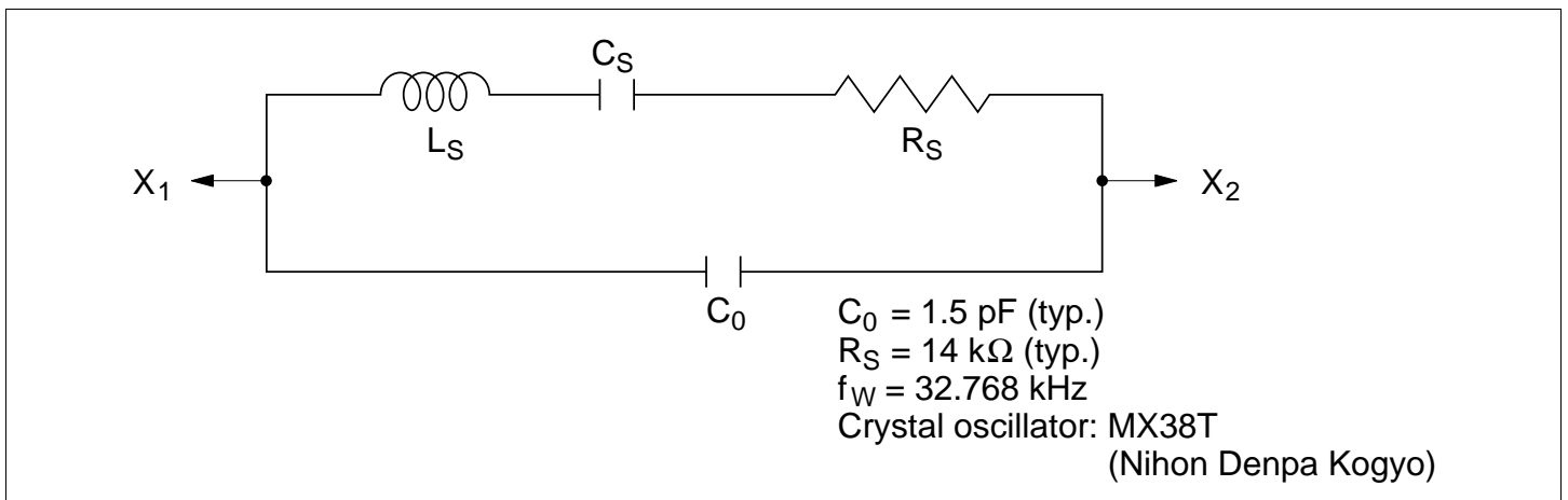
Figure 4.8 Equivalent Circuit of 32.768-kHz Crystal Oscillator
