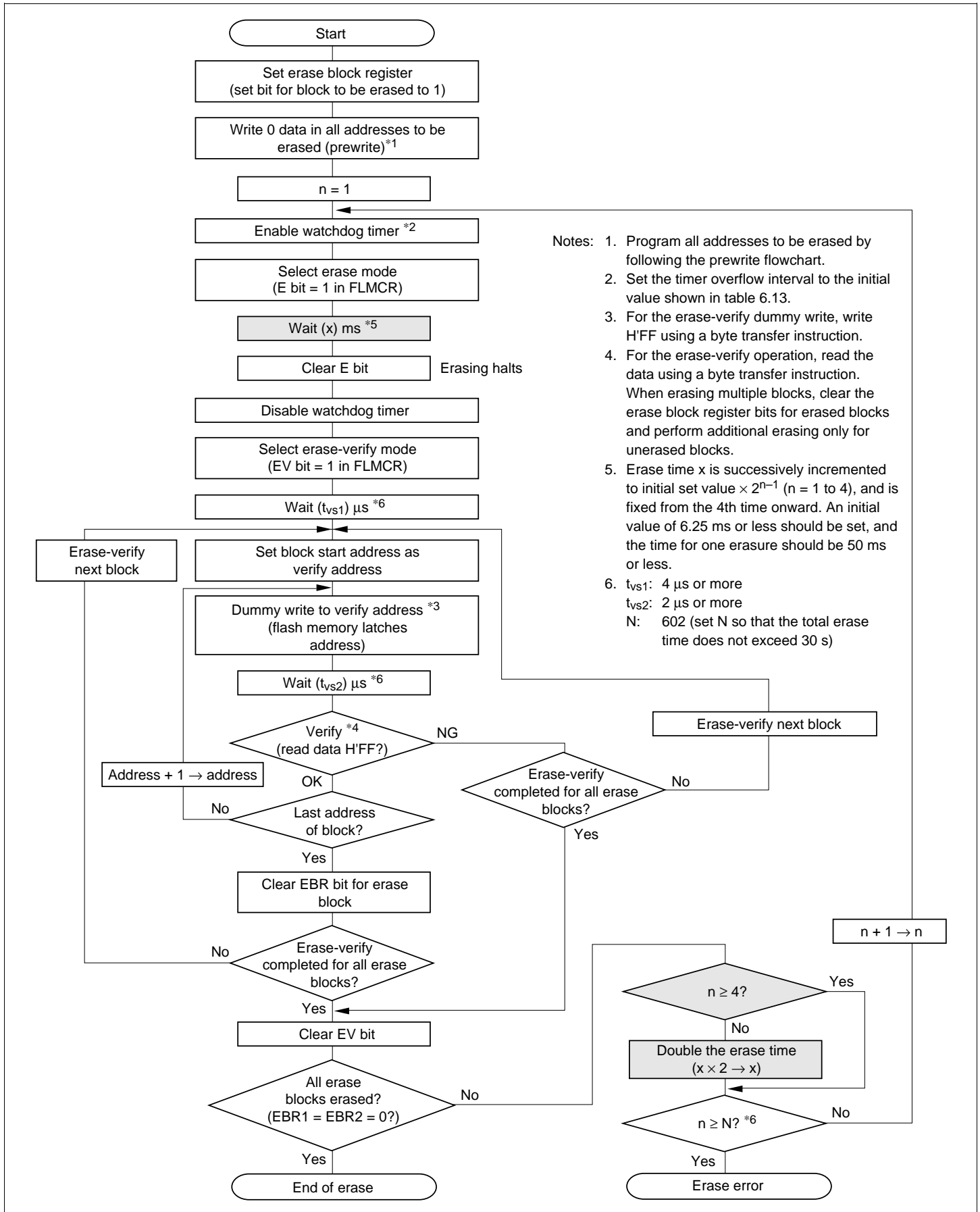
Figure 6.17 Multiple-Block Erase Flowchart
