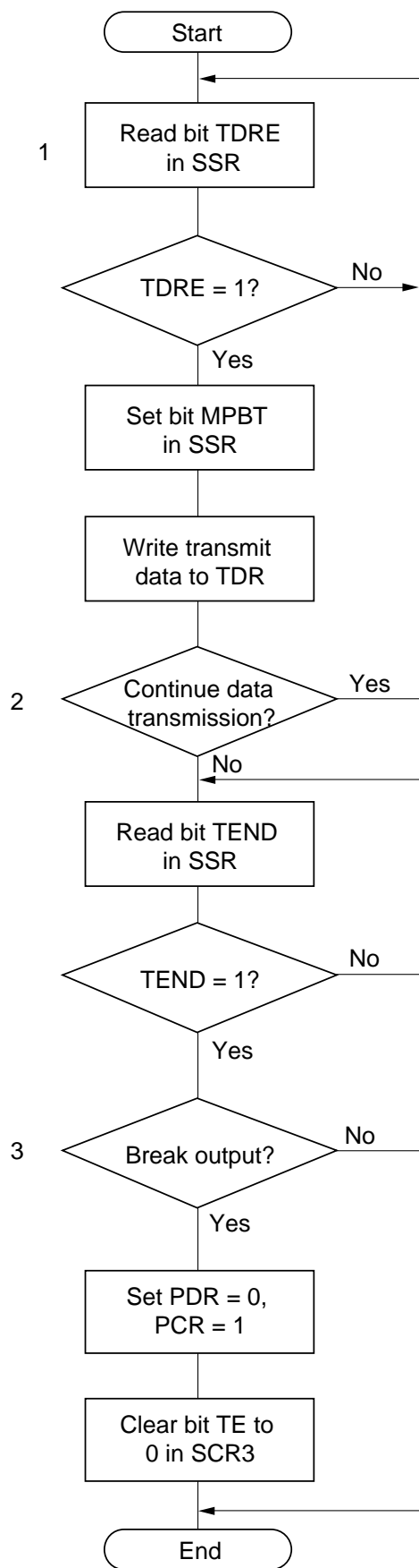
Figure 10.22 Example of Multiprocessor Data Transmission Flowchart
