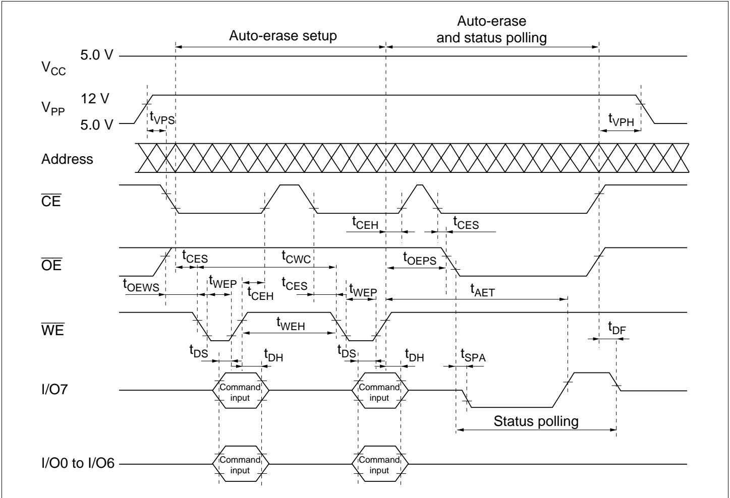
Figure 6.22 Auto-Erase Timing
