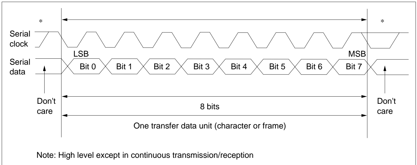
Figure 10.15 Data Format in Synchronous Communication
