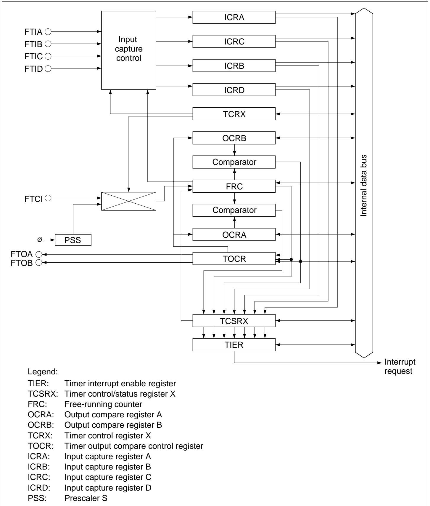
Figure 9.16 Block Diagram of Timer X
