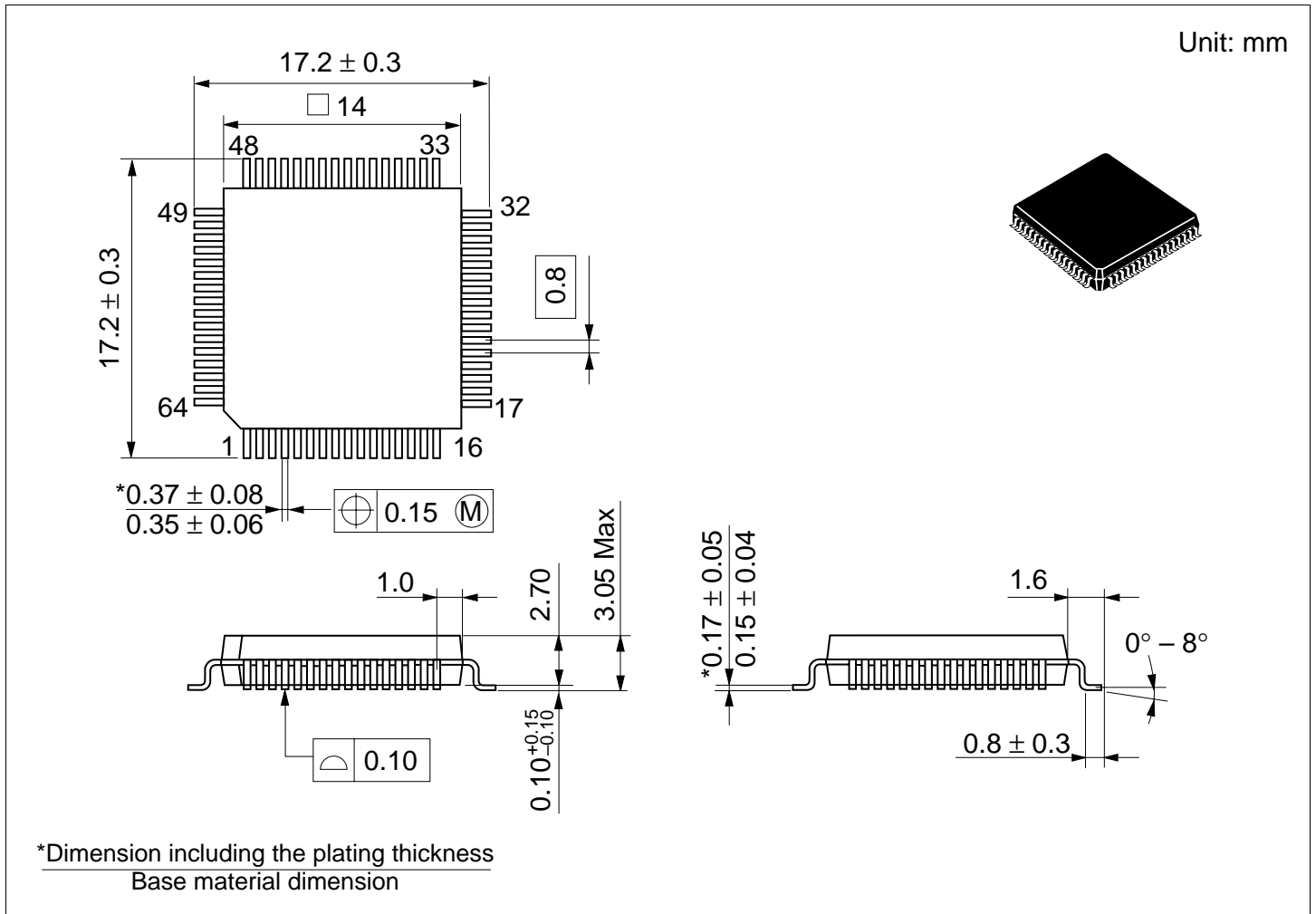
Figure F.1 FP-64A Package Dimensions
