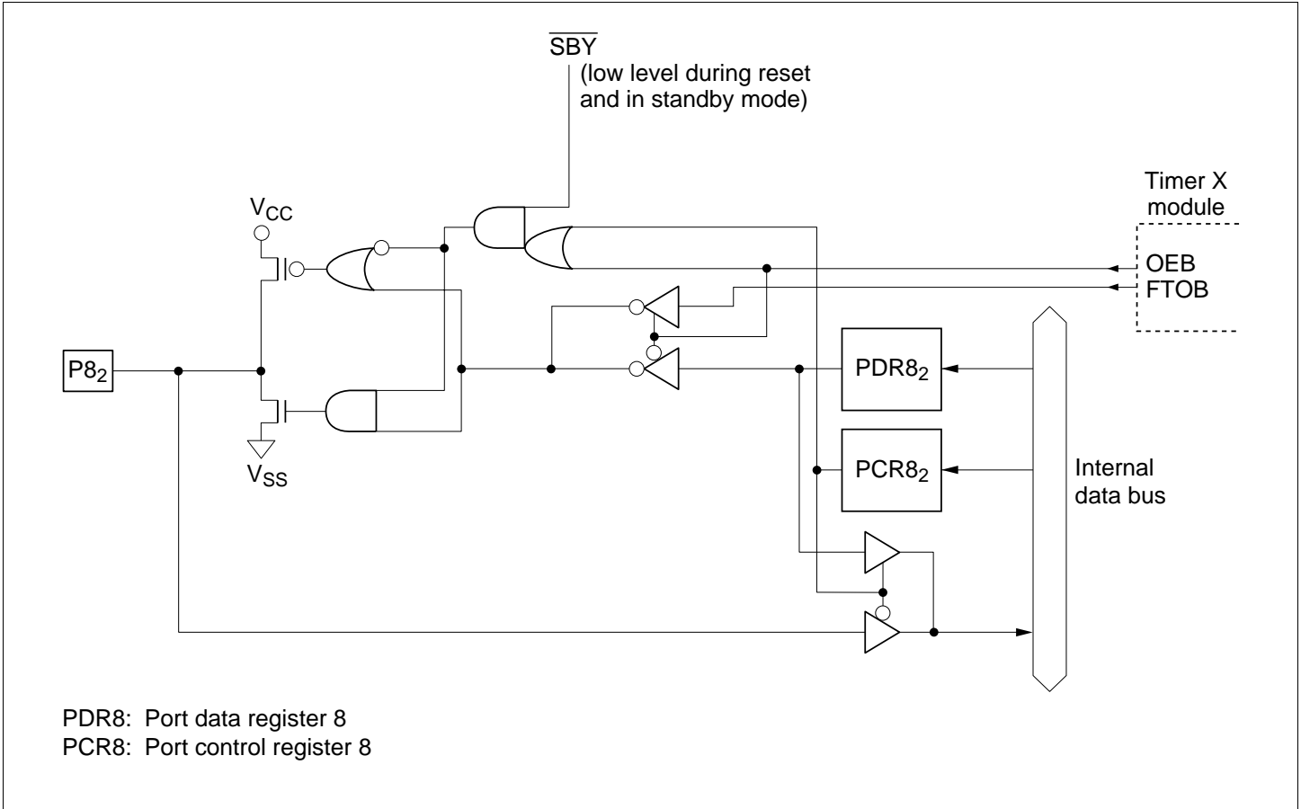
Figure C.7 (f) Port 8 Block Diagram (Pin P8 2 )
