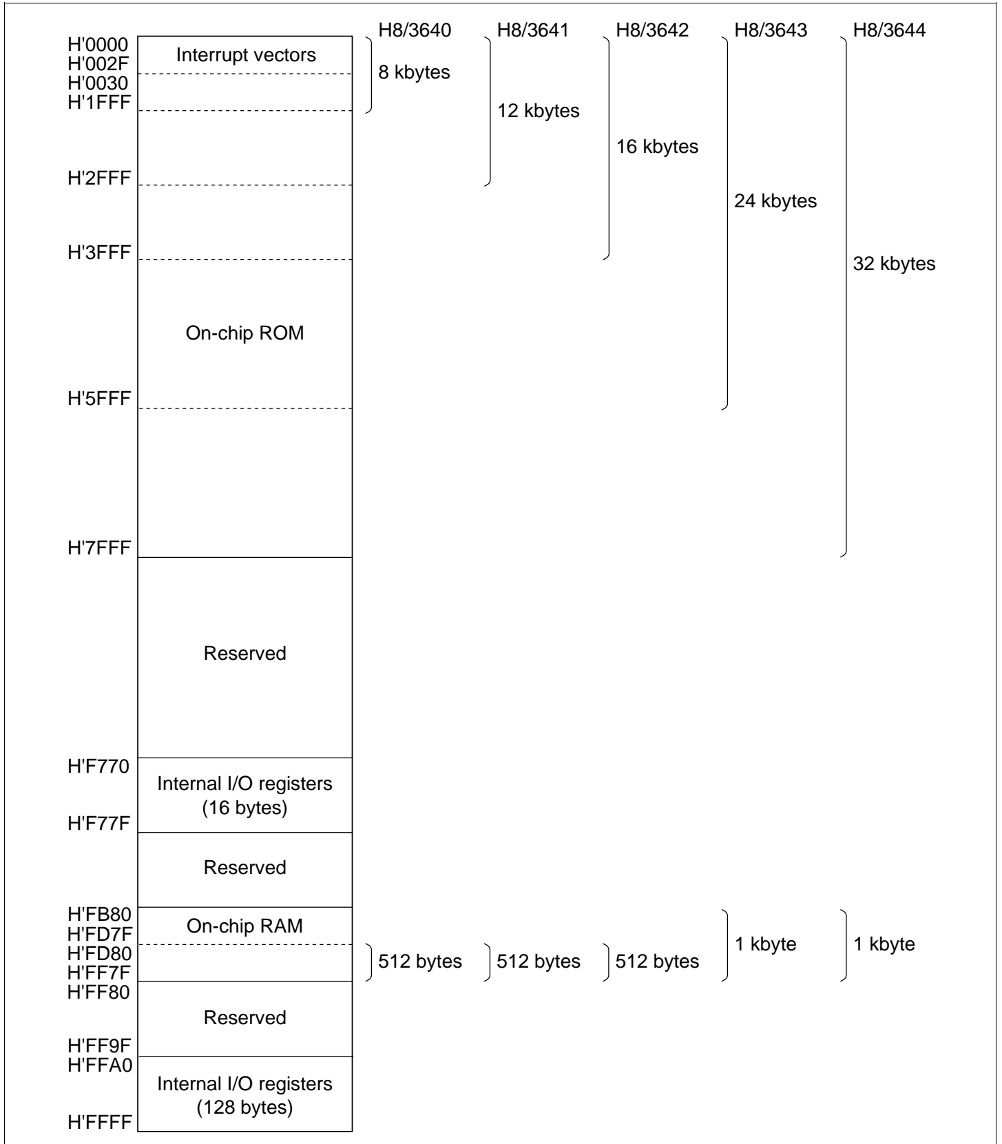
Figure 2.16 H8/3644 Series Memory Map
