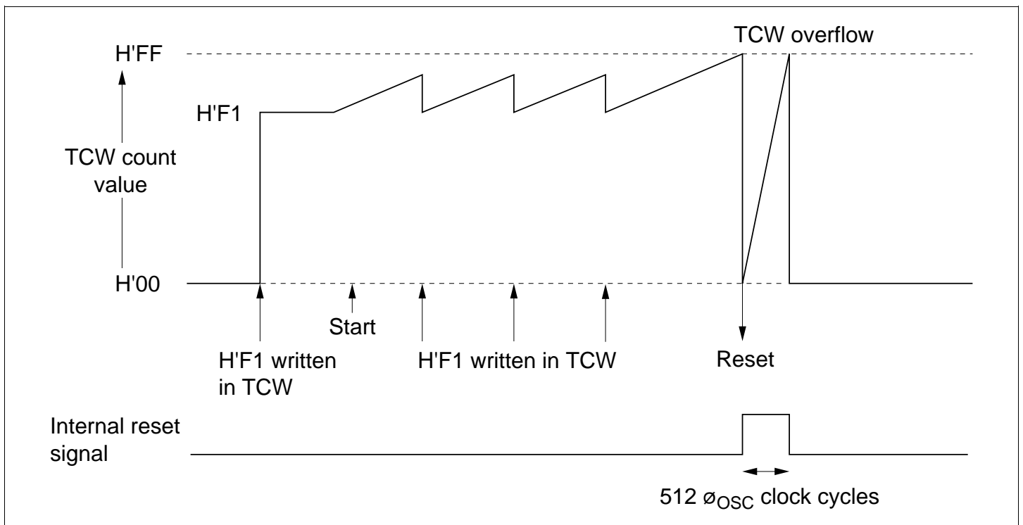
Figure 9.36 Typical Watchdog Timer Operations (Example)
