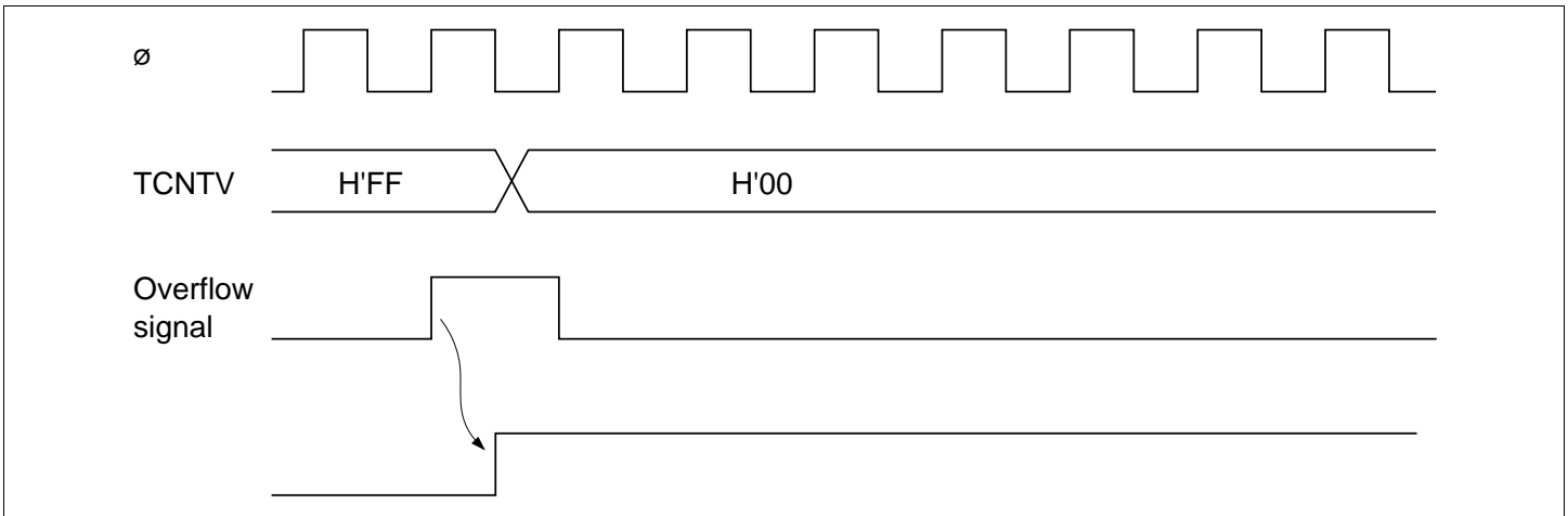
Figure 9.6 OVF Set Timing
