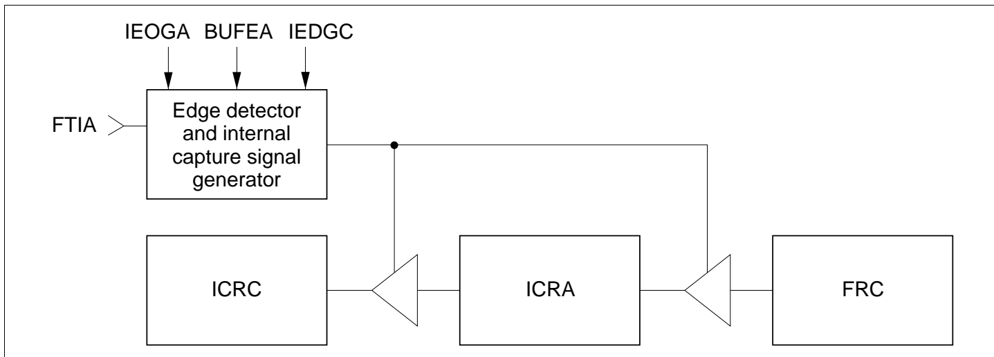
Figure 9.17 Buffer Operation (Example)
