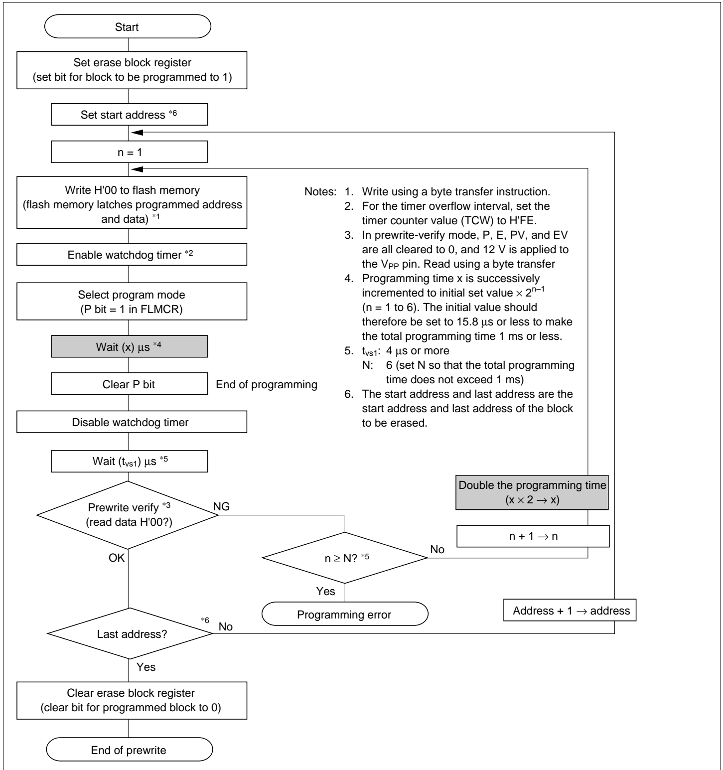
Figure 6.16 Prewrite Flowchart
