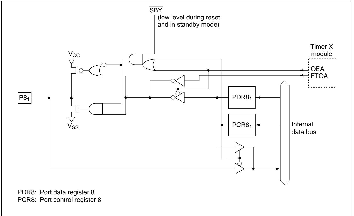
Figure C.7 (g) Port 8 Block Diagram (Pin P8 1 )
