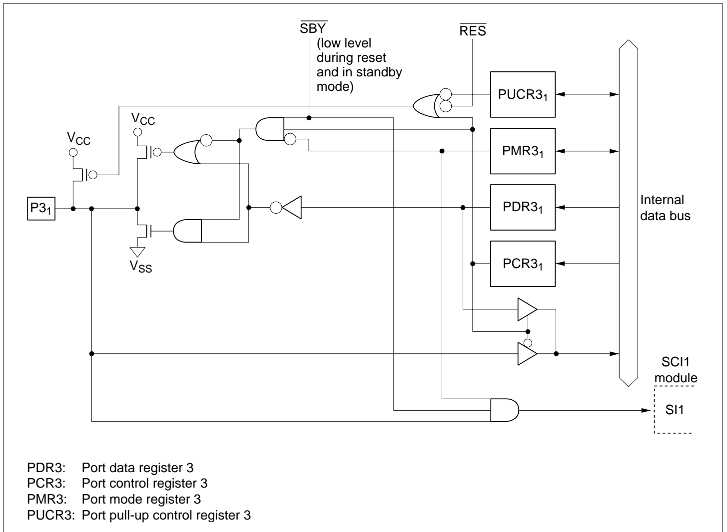
Figure C.3 (b) Port 3 Block Diagram (Pin P3 1 )
