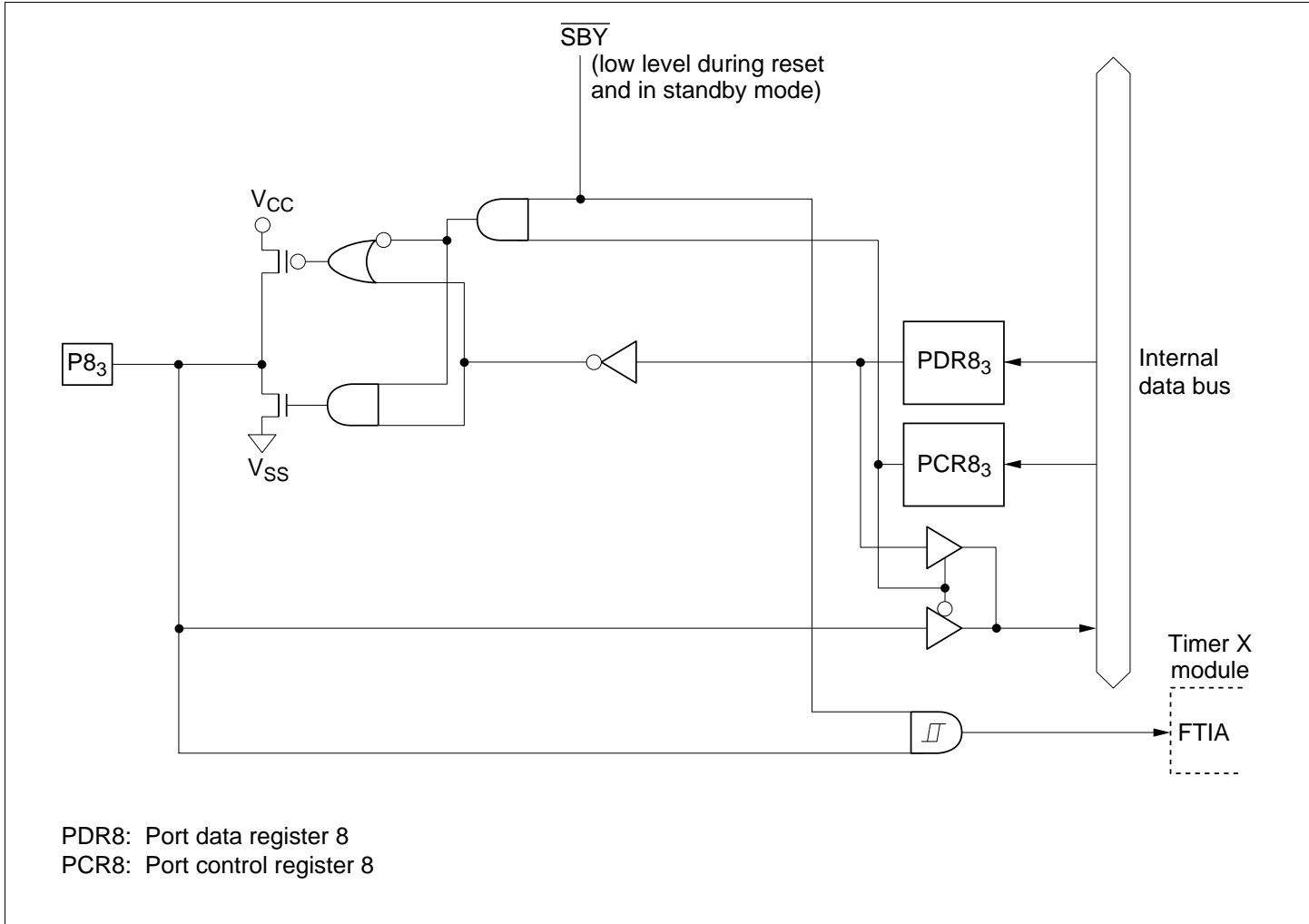
Figure C.7 (e) Port 8 Block Diagram (Pin P8 3 )
