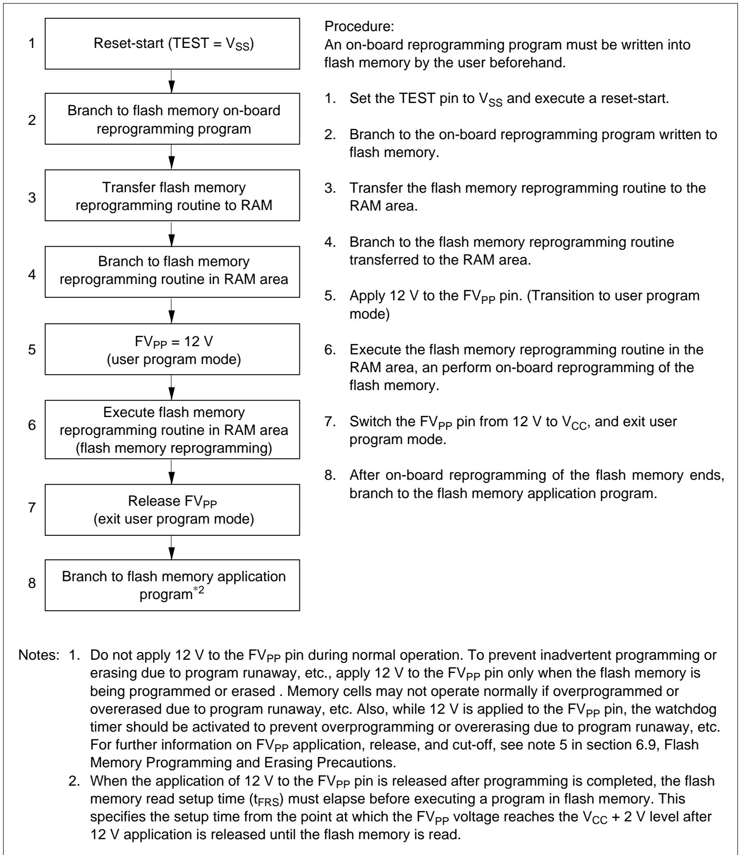
Figure 6.13 Example of User Program Mode Operation
