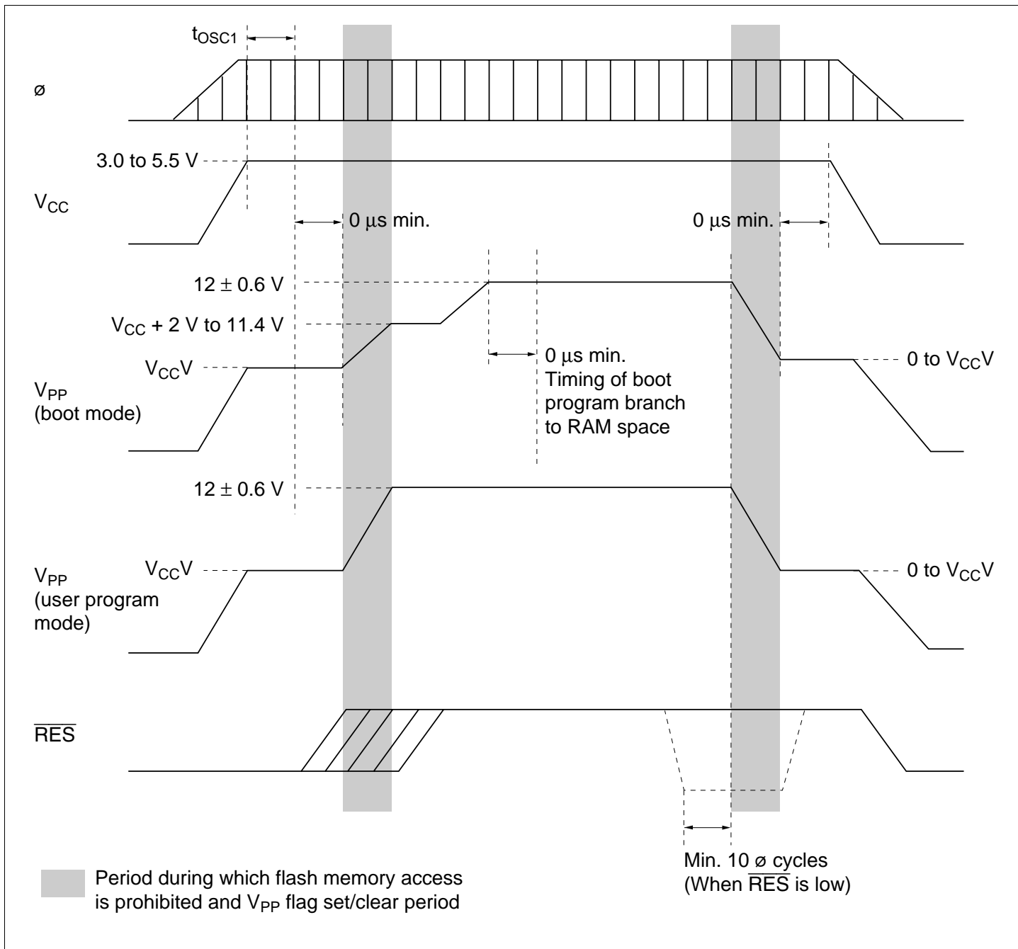
Figure 6.25 V pp Power-On and Cut-Off Timing
