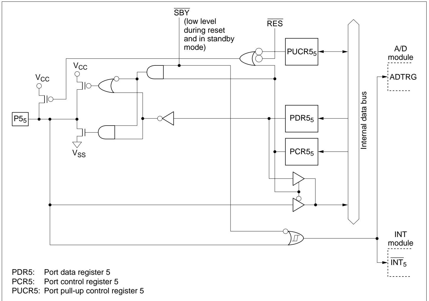
Figure C.4 (c) Port 5 Block Diagram (Pin P5 5 )
