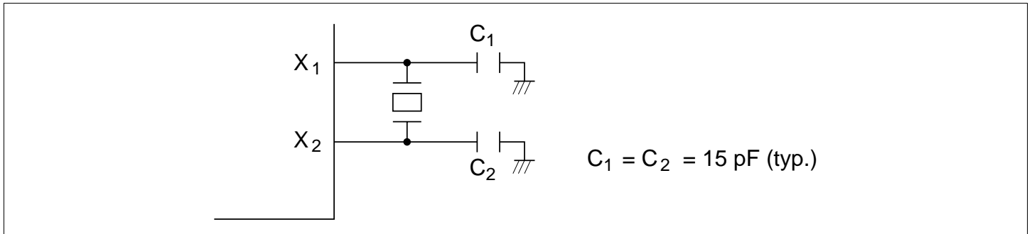
Figure 4.7 Typical Connection to 32.768-kHz Crystal Oscillator
