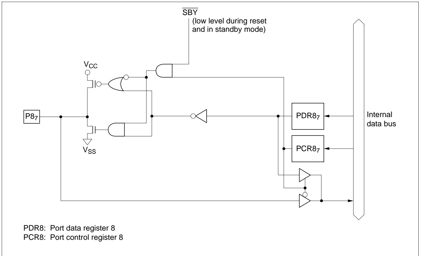
Figure C.7 (a) Port 8 Block Diagram (Pin P8 7 )
