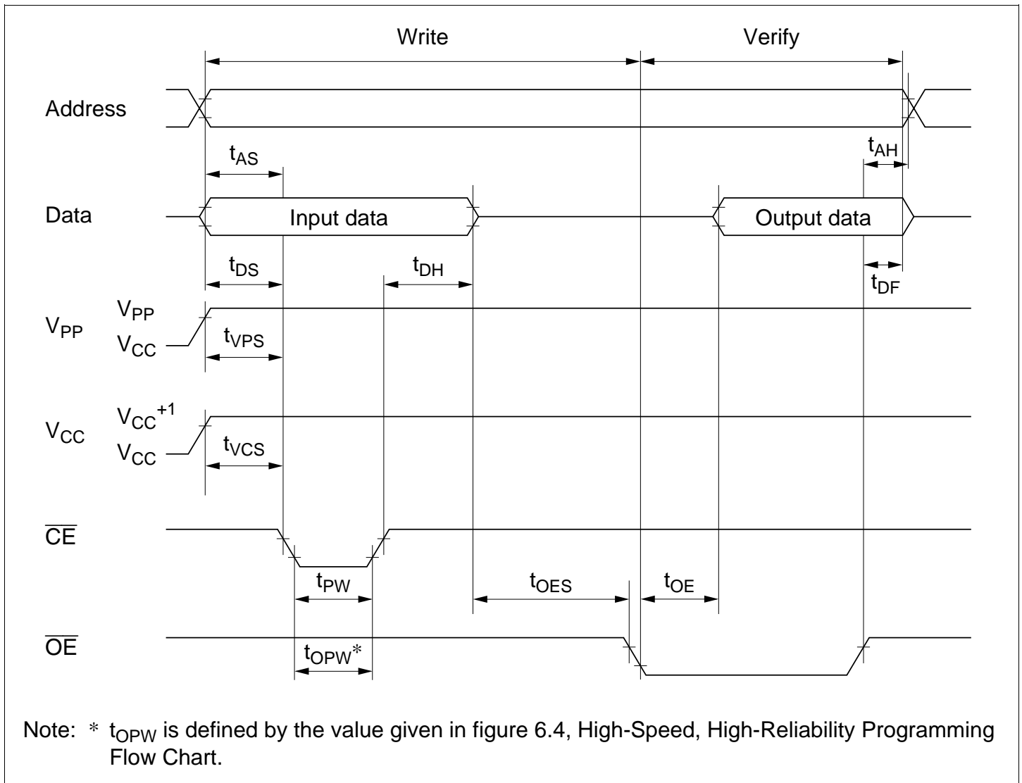
Figure 6.5 PROM Write/Verify Timing
