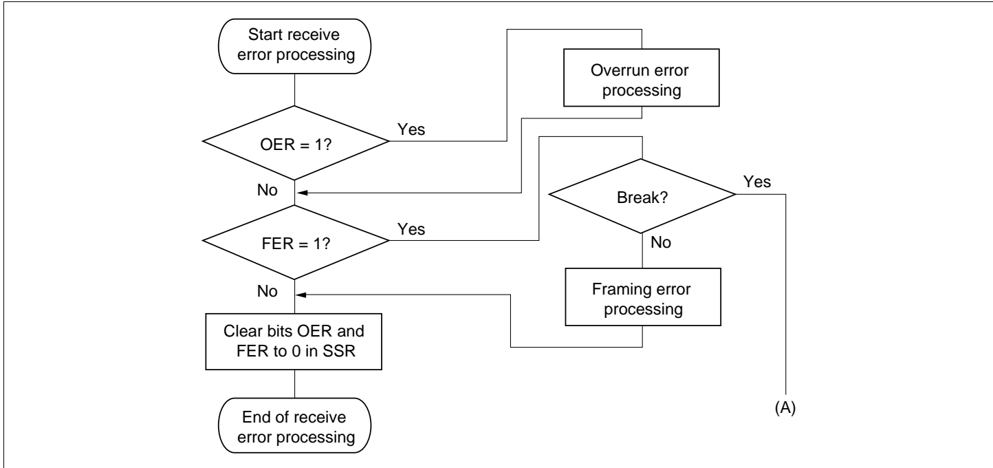
Figure 10.24 Example of Multiprocessor Data Reception Flowchart (cont)
