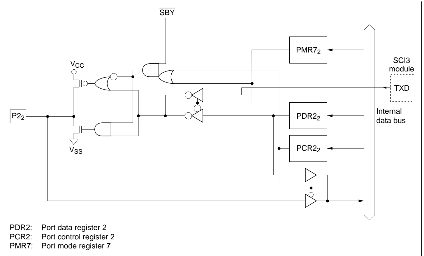
Figure C.2 (a) Port 2 Block Diagram (Pin P2 2 )
