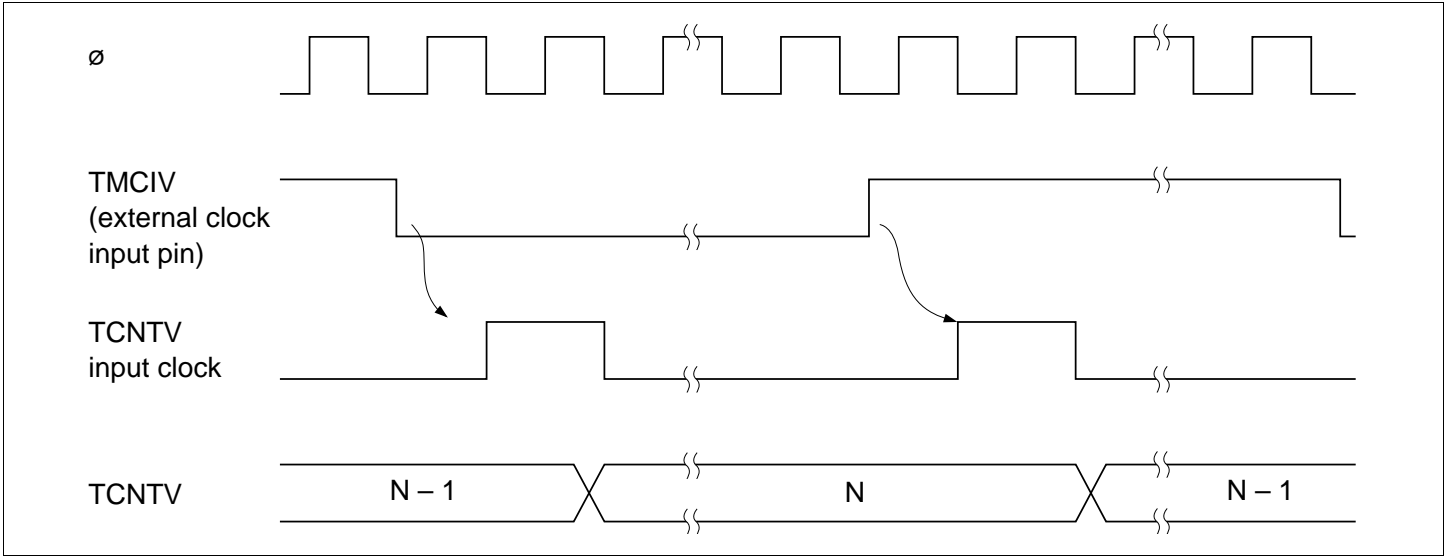
Figure 9.5 Increment Timing with External Clock
