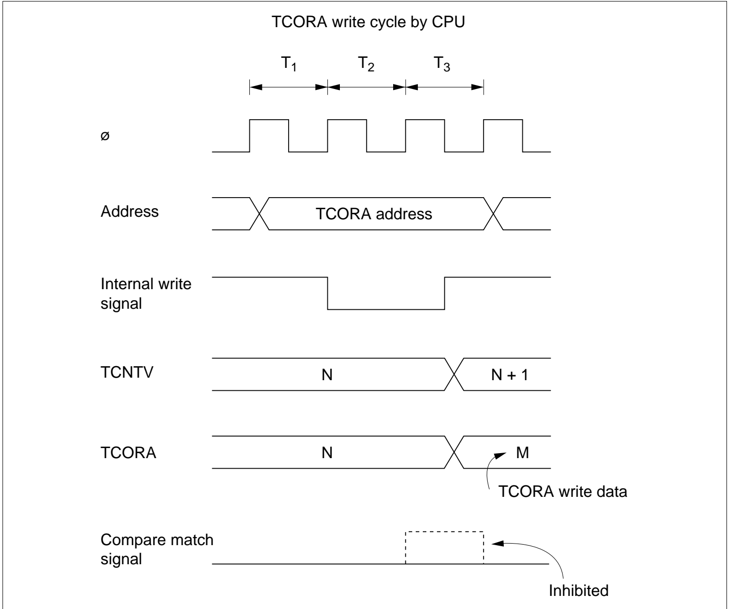
Figure 9.15 Contention between TCORA Write and Compare Match
