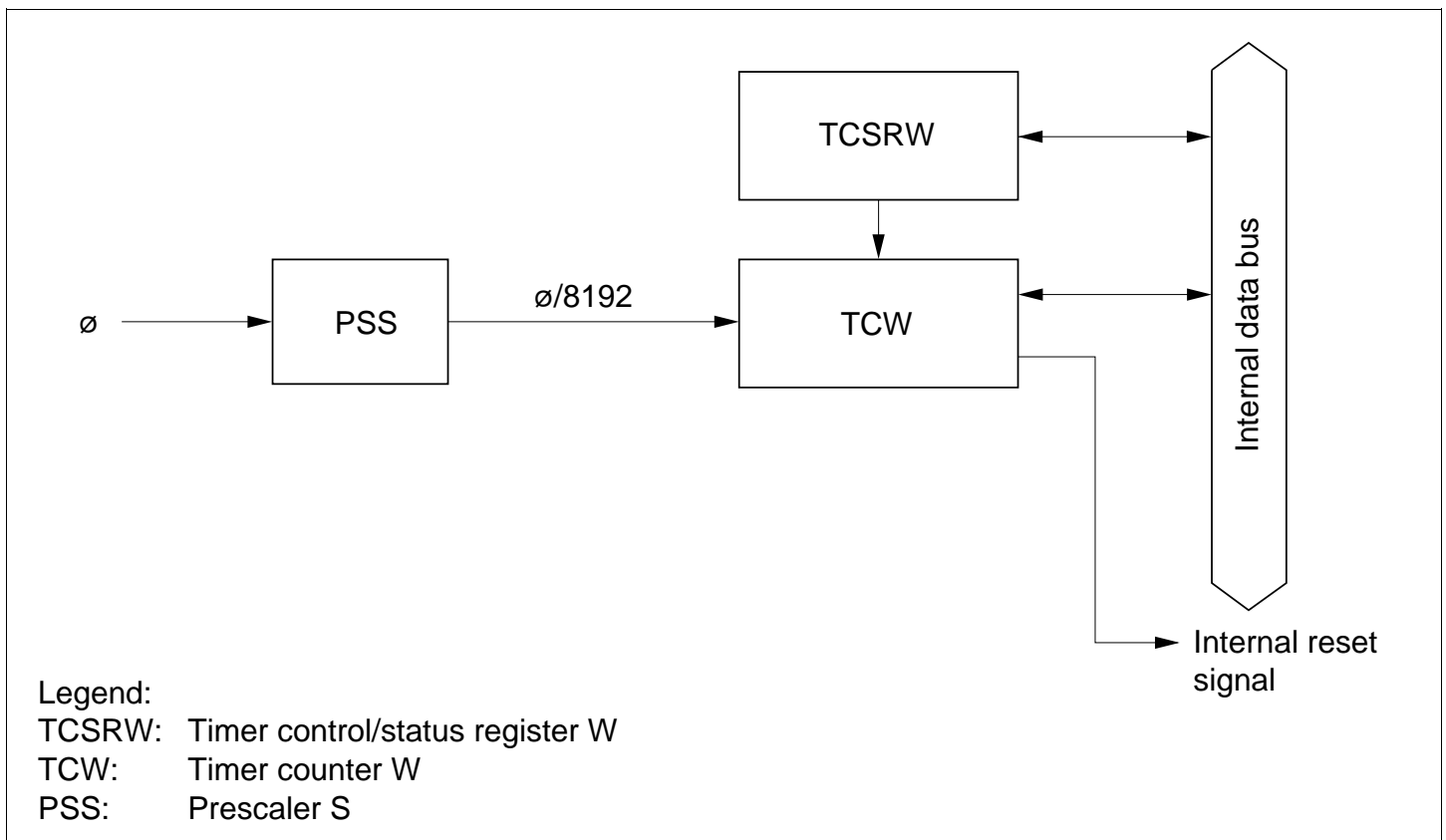
Figure 9.35 Block Diagram of Watchdog Timer
