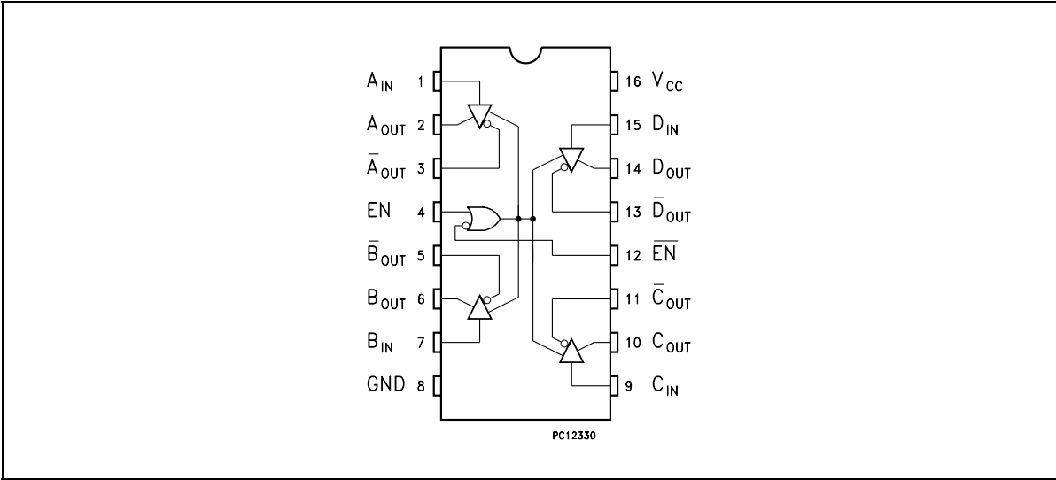
Figure 1. Pin connections
