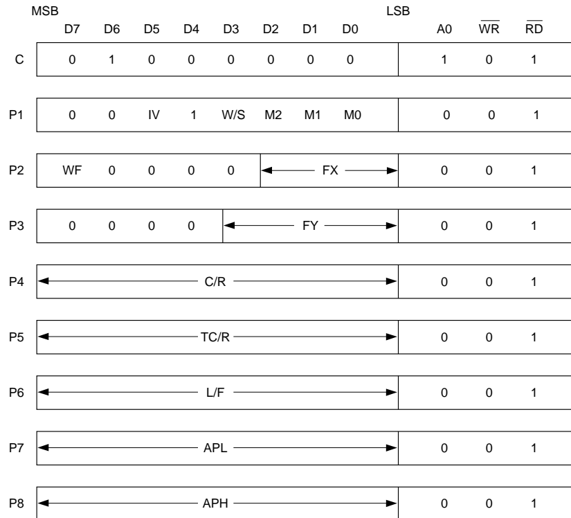
Figure 1. SYSTEM SET instruction
