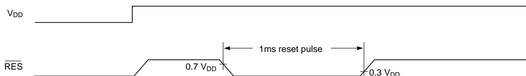
Figure 56. Reset timing
