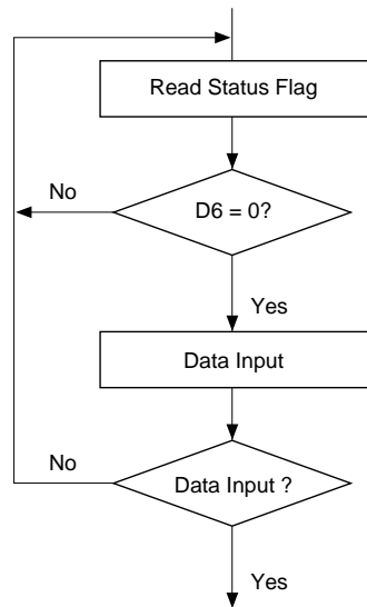
Figure 55. Flowchart for busy flag checking
