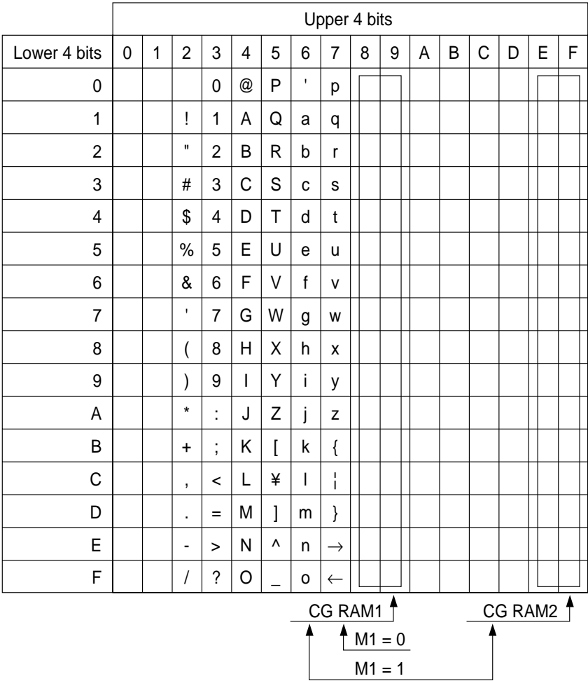
Figure 46. On-chip character codes
