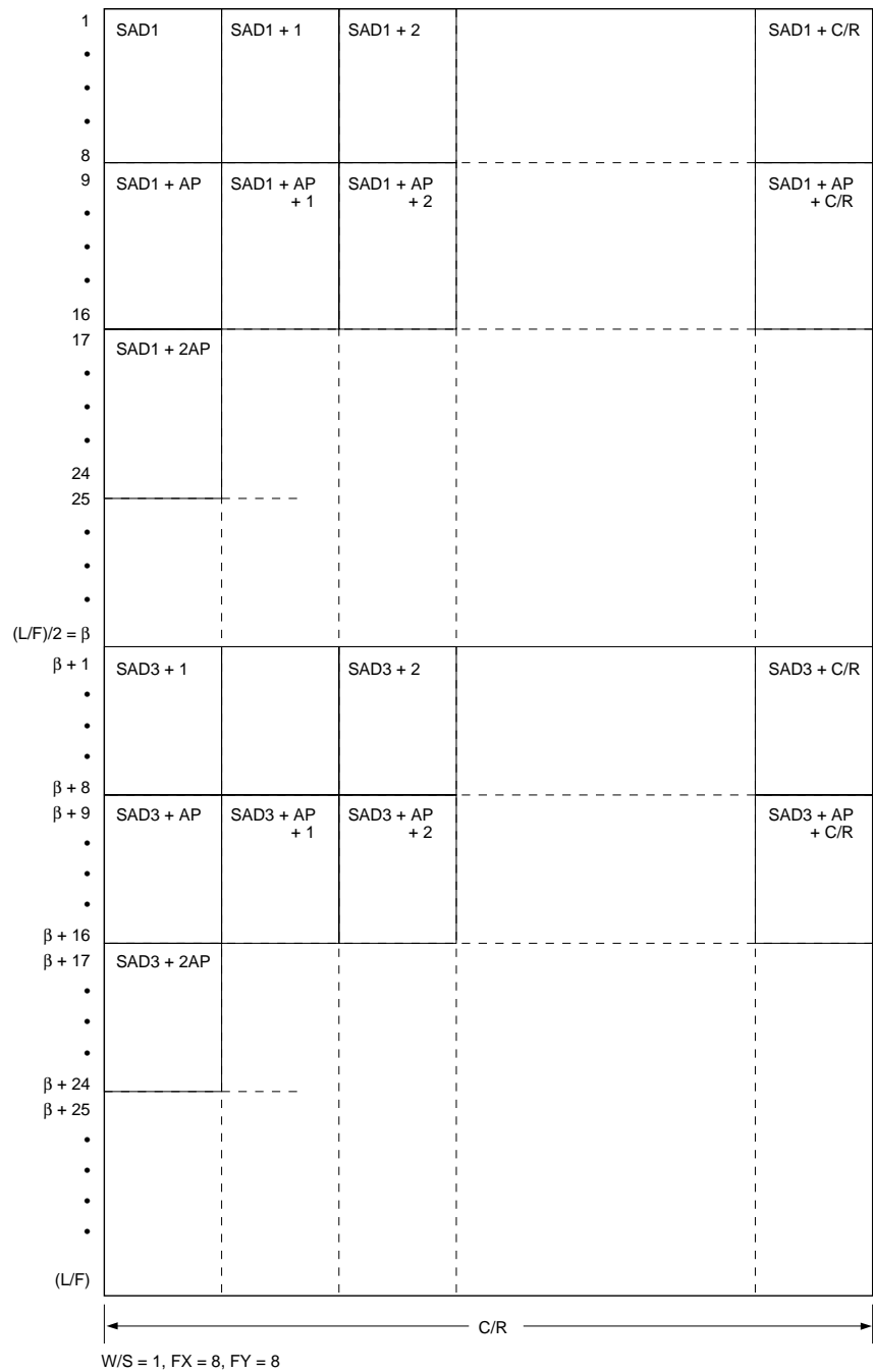
Figure 31. Two-panel display address indexing
