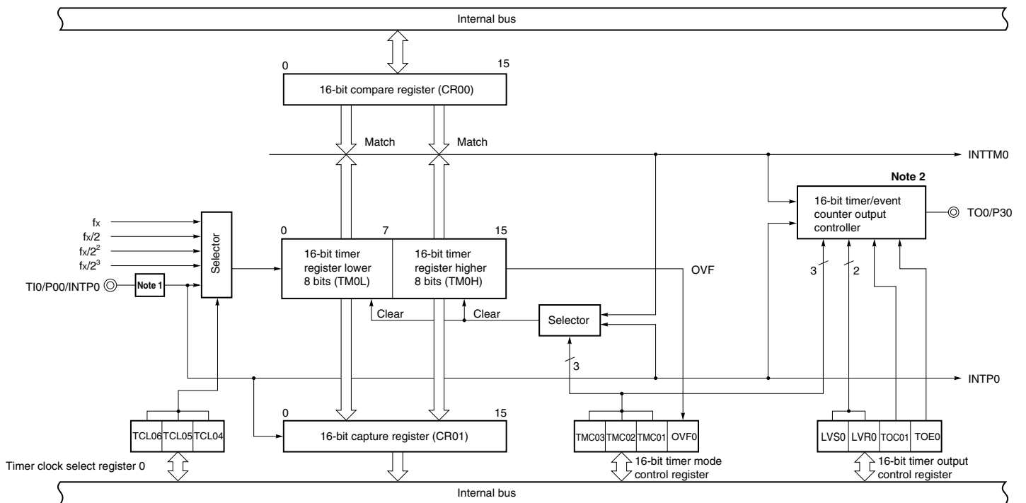
Figure 6-1. Block Diagram of 16-Bit Timer/Event Counter (Timer Mode)
