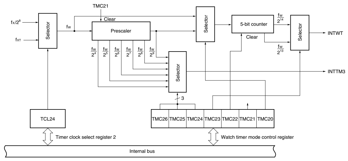
Figure 8-1. Watch Timer Block Diagram
