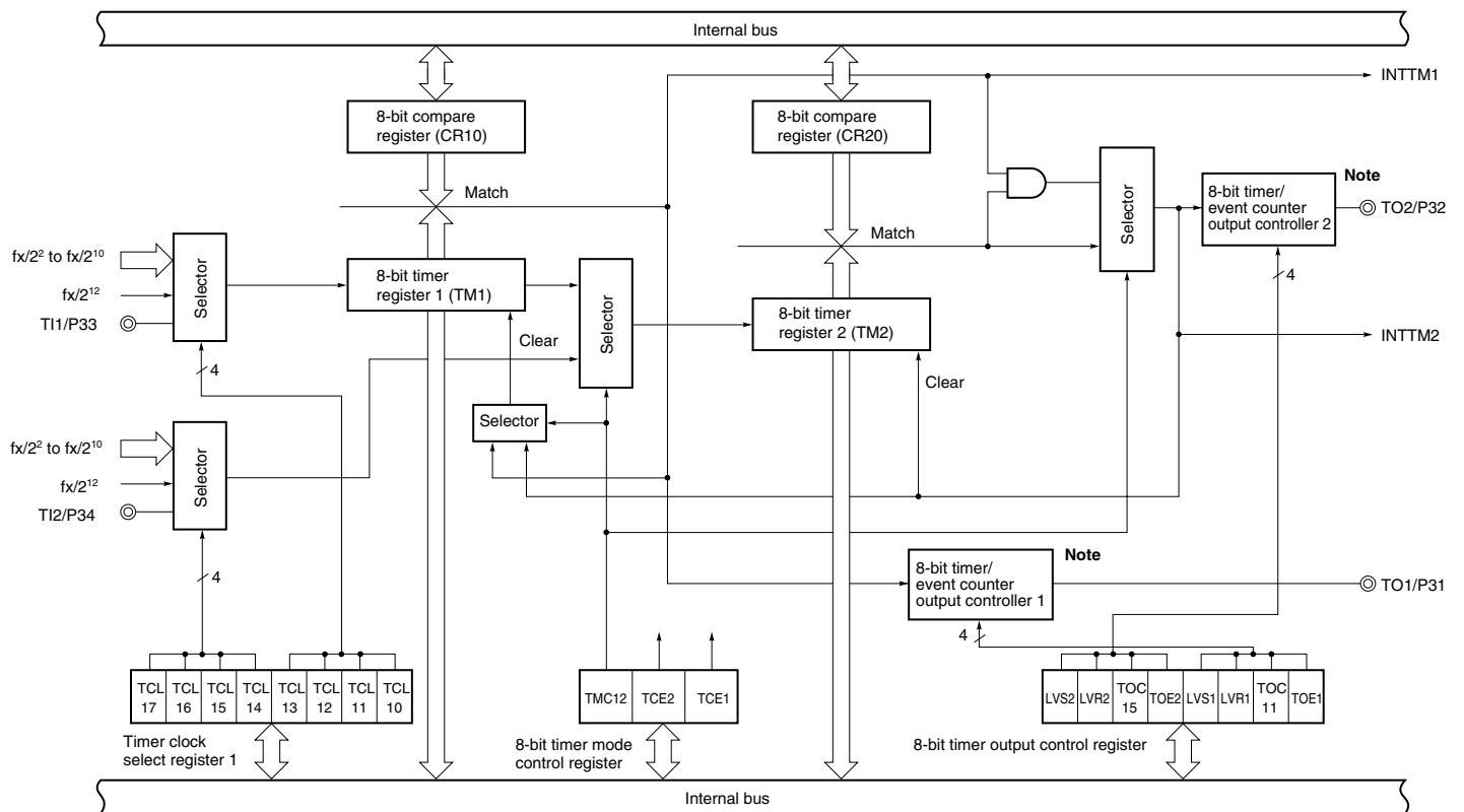
Figure 7-1. Block Diagram of 8-Bit Timer/Event Counter
