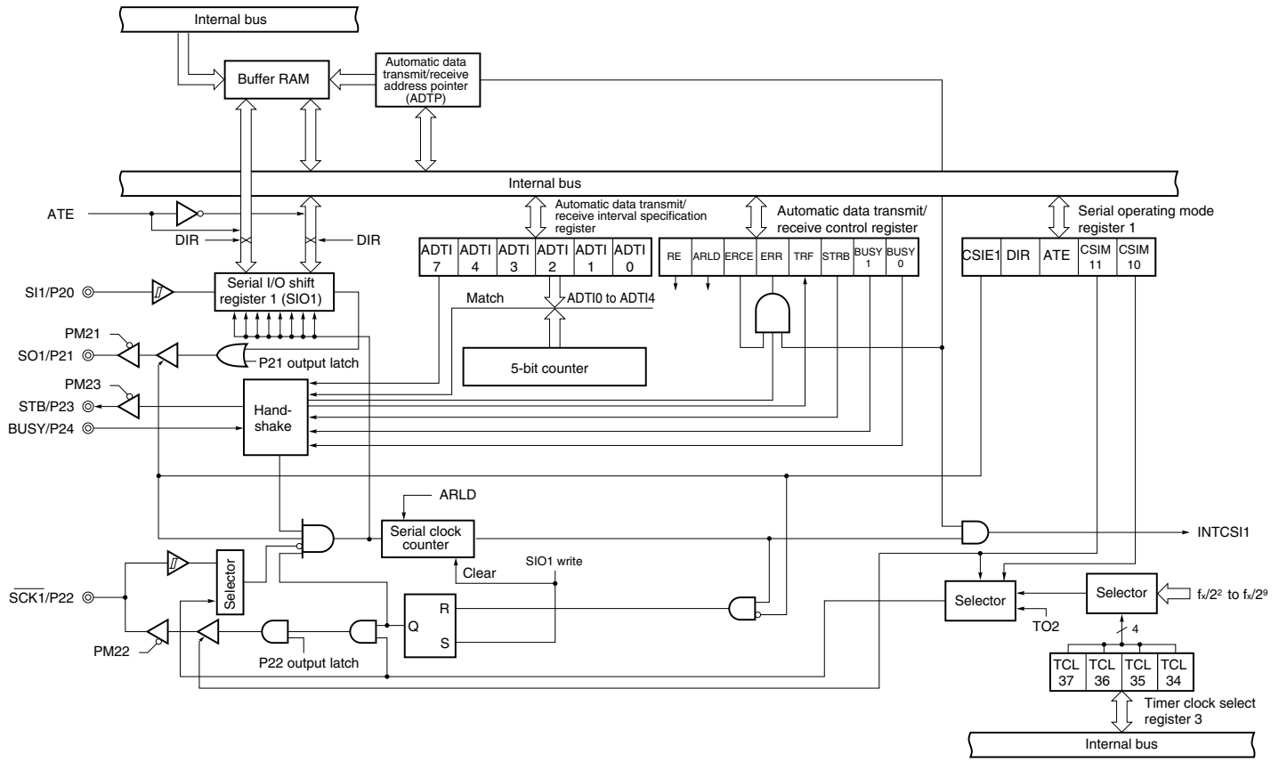
Figure 14-1. Block Diagram of Serial Interface Channel 1
