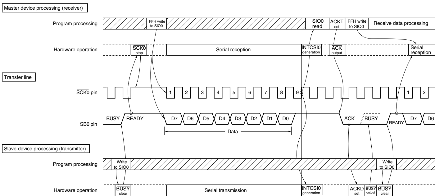
Figure 13-29. Data Transmission from Slave Device to Master Device
