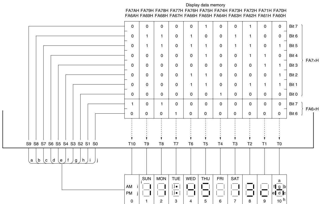
Figure 15-15. Relationship Between Display Data Memory Contents and Segment Outputs in 10-Segment x 11-Digit Display Mode
