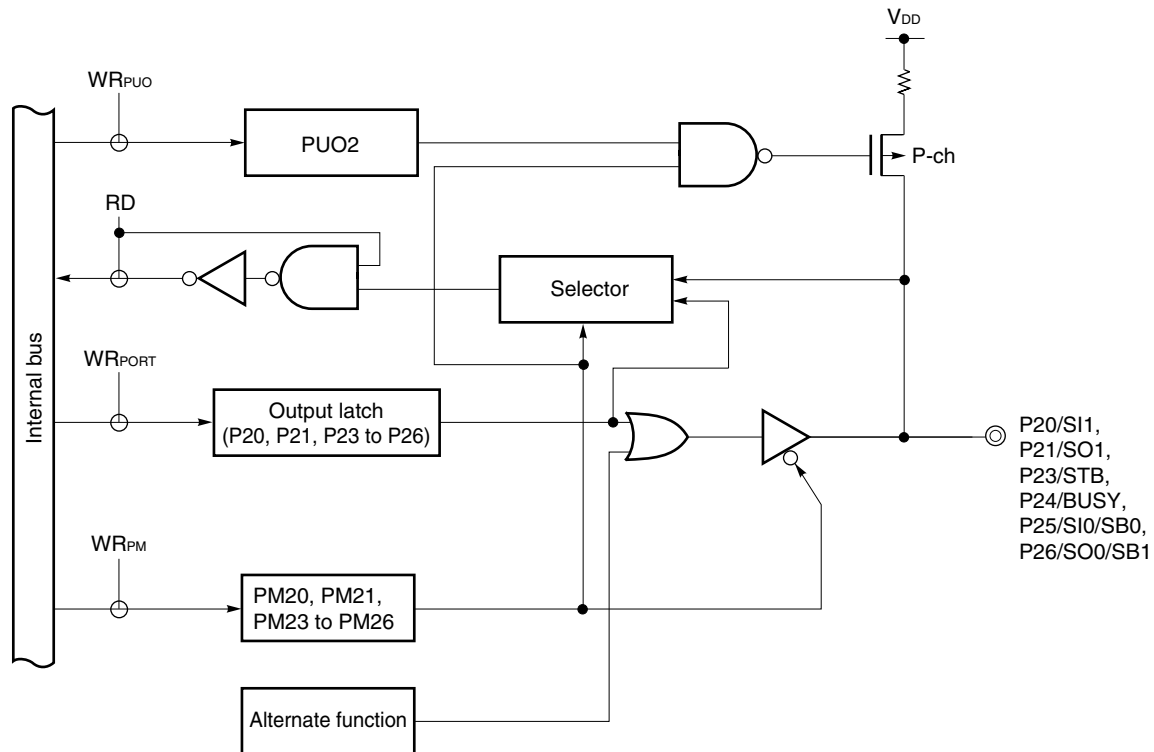
Figure 4-5. Block Diagram of P20, P21, P23 to P26
