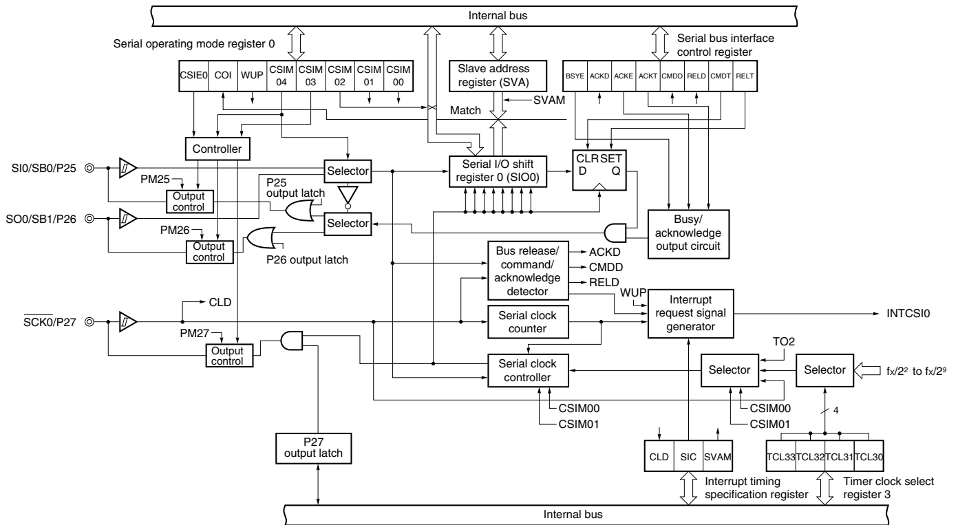
Figure 13-1. Block Diagram of Serial Interface Channel 0
