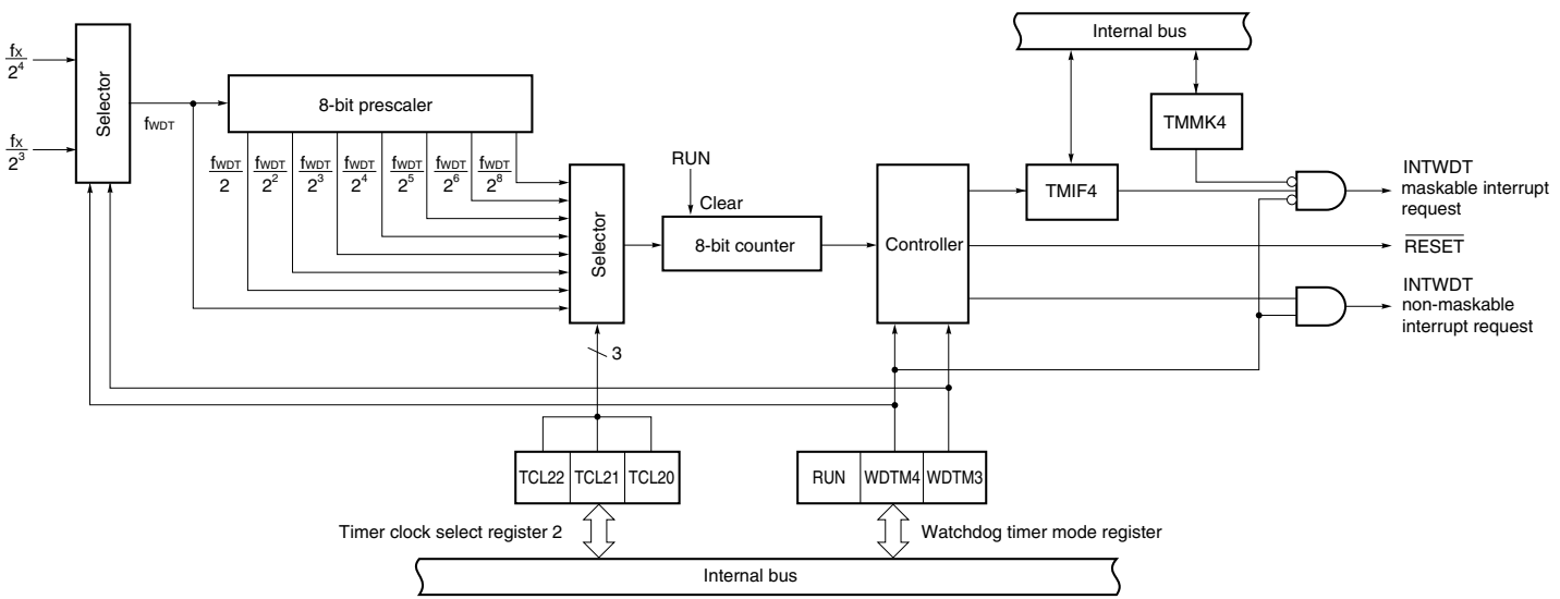
Figure 9-1. Watchdog Timer Block Diagram
