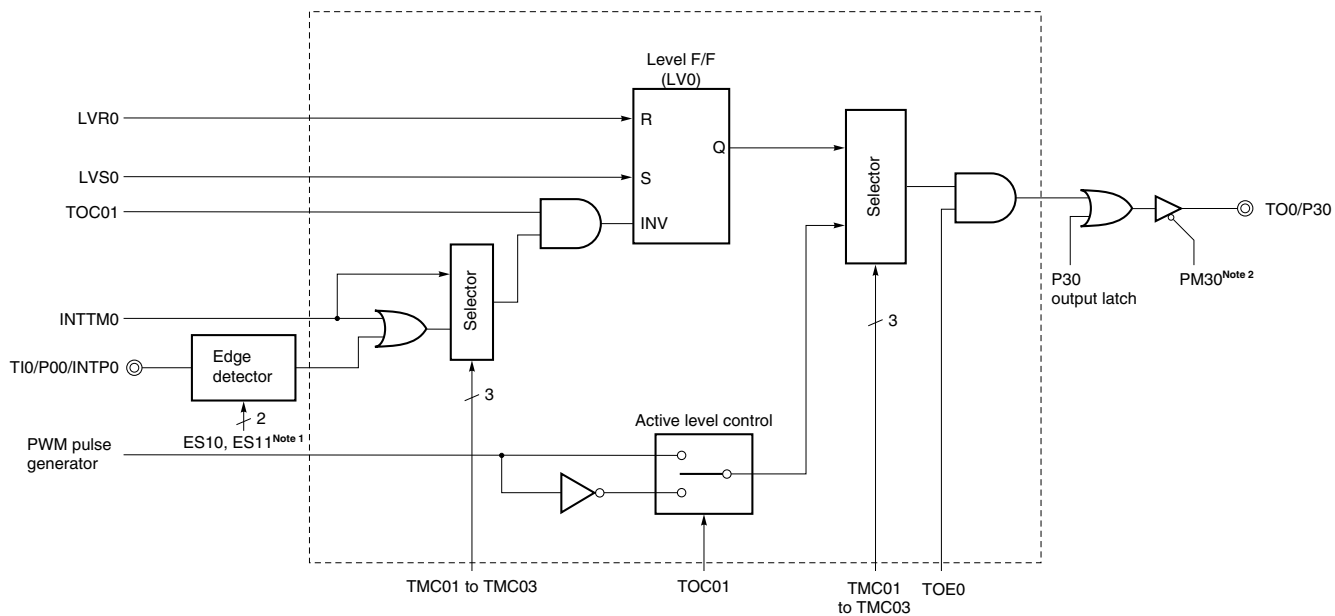
Figure 6-3. Block Diagram of 16-Bit Timer/Event Counter Output Controller
