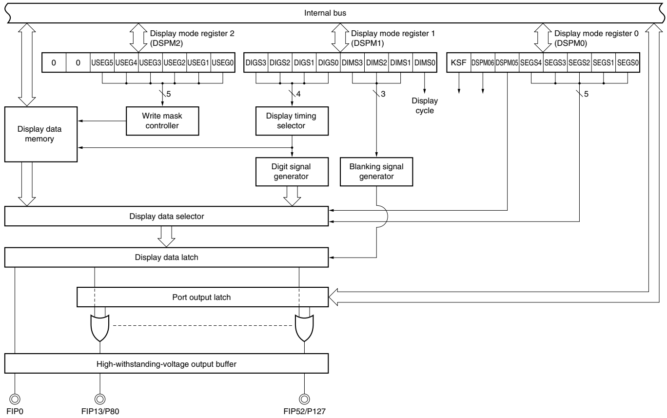
Figure 15-2. VFD Controller/Driver Block Diagram
