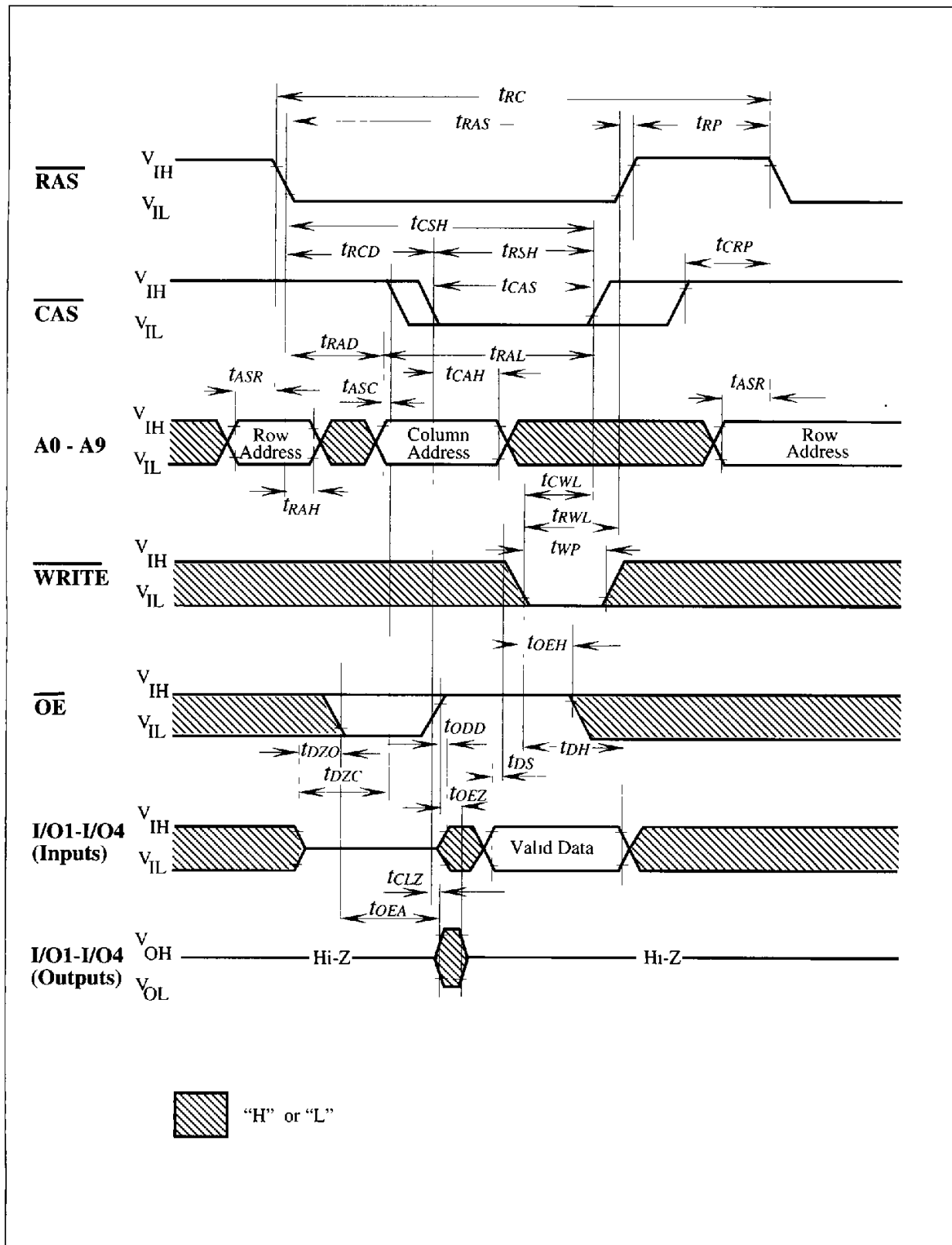
Write Cycle (OE Controlled Write)
