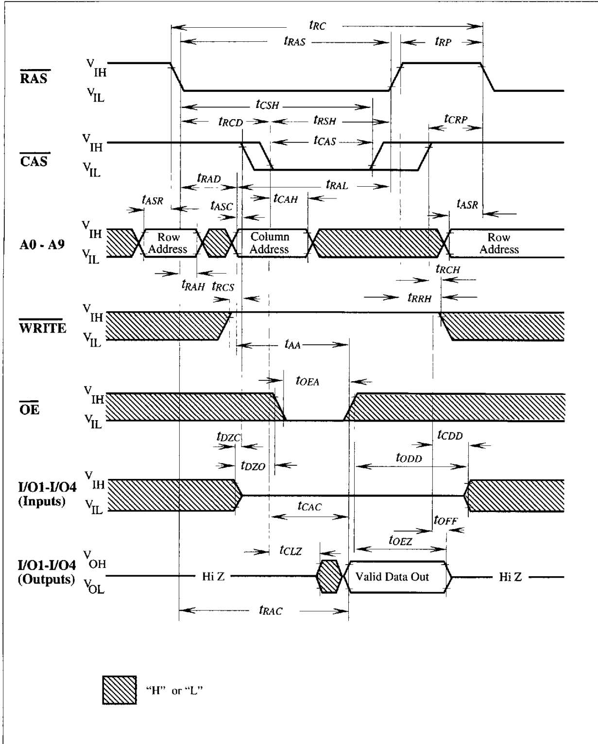
Read Cycle
