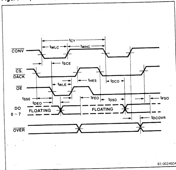
Figure 3. Timing Chart
