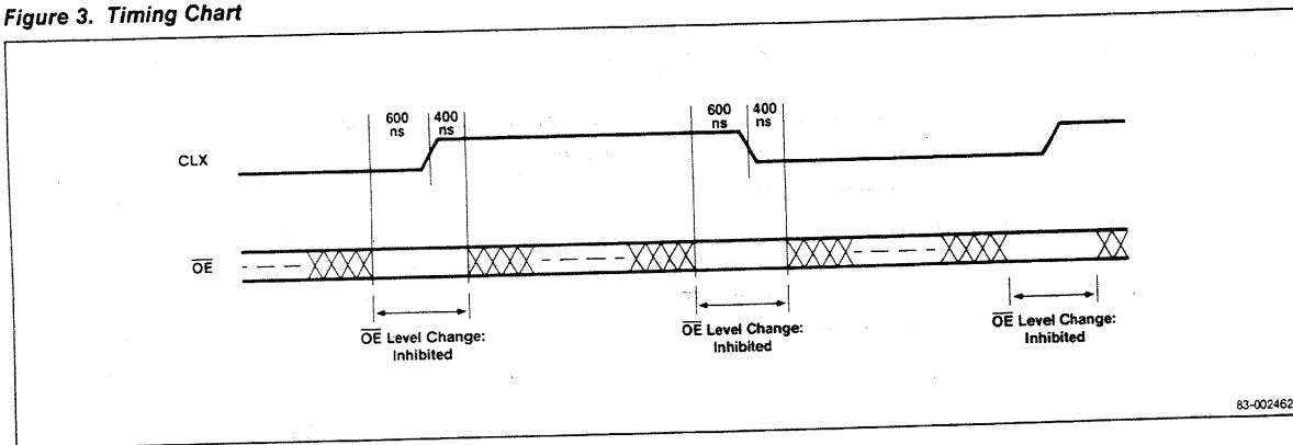
Figure 3. Timing Chart
