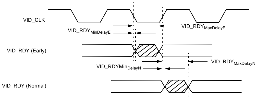
Figure 5-7. VID_RDY Delays
