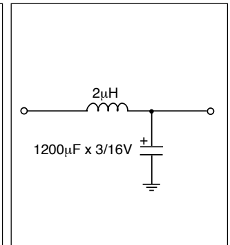
Figure 17: Input Filter
