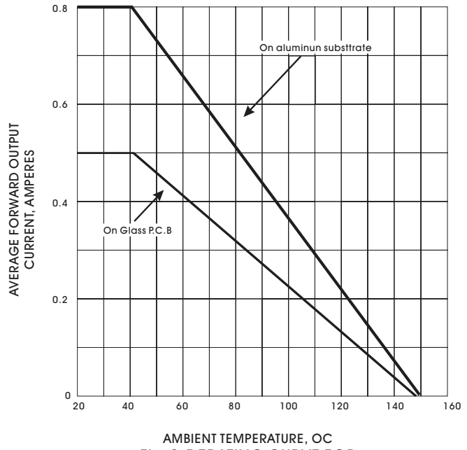
Fig. 2 - DERATING CURVE FOR OUTPUT RECTIFIED CURRENT
