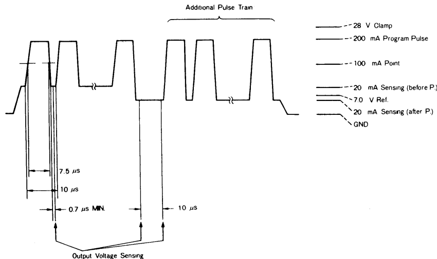
Fig. 2 Typical Output Voltage Waveform.
