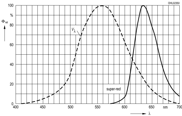
LED Relative spectral emission I_{rel} = f(\lambda) , T_A = 25^\circ\text{C} , I_F = 20\text{ mA} V(\lambda) = \text{Standard eye response curve}
