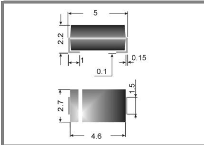
Surface mount diode
