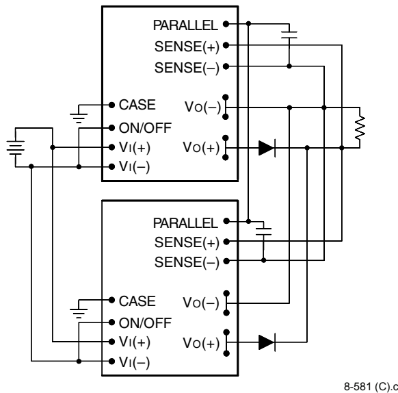
Figure 26. Wiring Configuration for Redundant Parallel Operation
