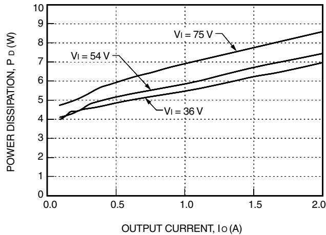
Figure 29. JFW050H Power Dissipation vs. Output Current at 25 °C
