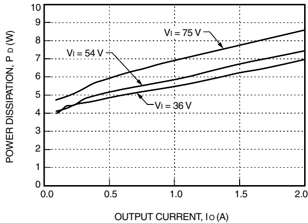
Figure 29. JFW050H Power Dissipation vs. Output Current at 25 °C
