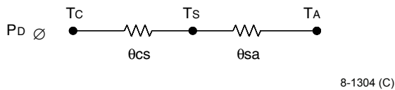
Figure 34. Resistance from Case-to-Sink and Sink-to-Ambient
