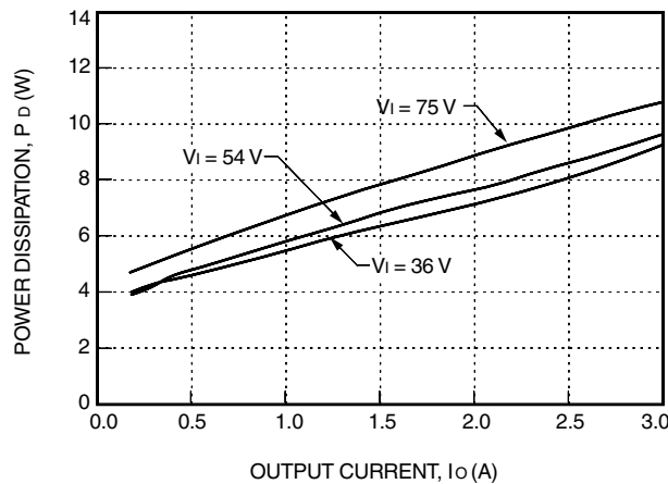
Figure 30. JFW075H Power Dissipation vs. Output Current at 25 °C
