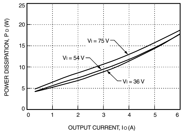
Figure 32. JFW150H Power Dissipation vs. Output Current at 25 °C
