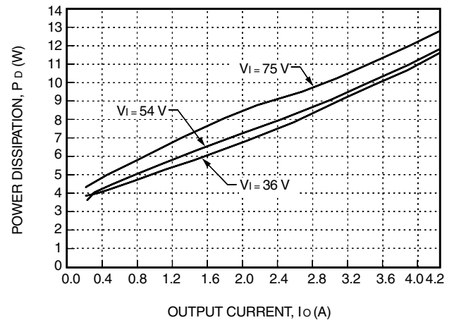
Figure 31. JFW100H Power Dissipation vs. Output Current at 25 °C
