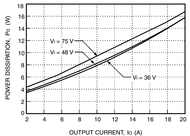
Figure 23. JFW100G Power Dissipation vs. Output Current at 80 °C
