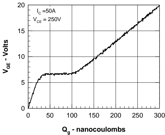
Fig. 9. Gate Charge
