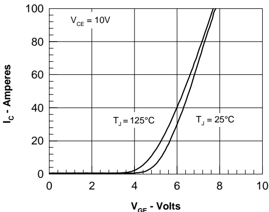
Figure 5. Admittance Curves
