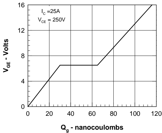
Figure 9. Gate Charge
