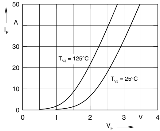
Fig. 10 Typ. forward characteristics of free wheeling diode
