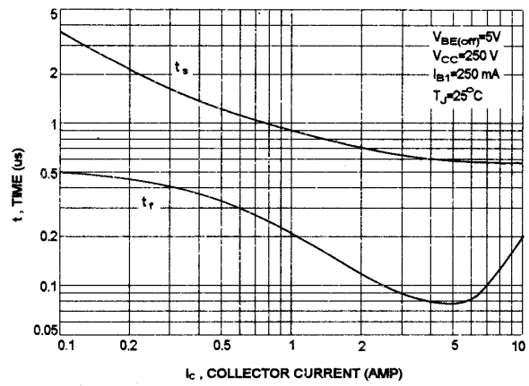
TURN-OFF TIME
