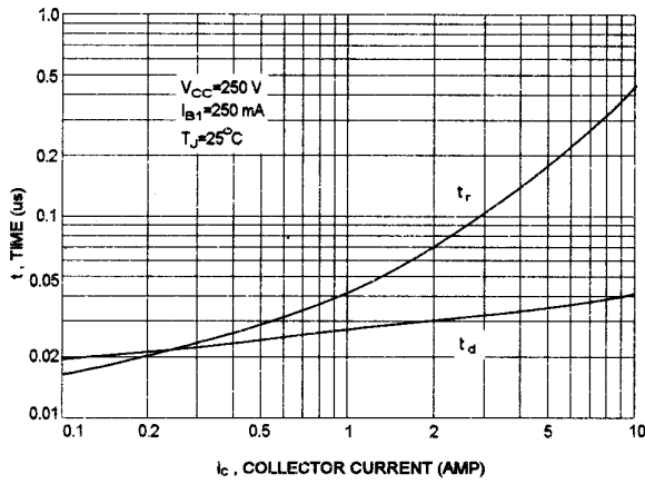
TURN-ON TIME
