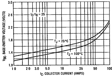
FIGURE 17 — BASE-EMITTER SATURATION VOLTAGE
