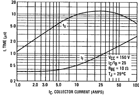
FIGURE 29 — TYPICAL TURN-OFF SWITCHING TIMES MJ10048
