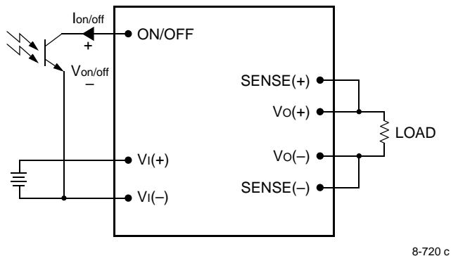
Figure 16. Remote On/Off Implementation
