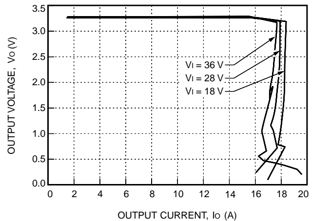
Figure 4. Typical JC075F Output Characteristics at Room Temperature
