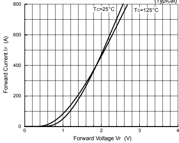
Fig.13- Forward Characteristics of Free Wheeling Diode (Typical)
