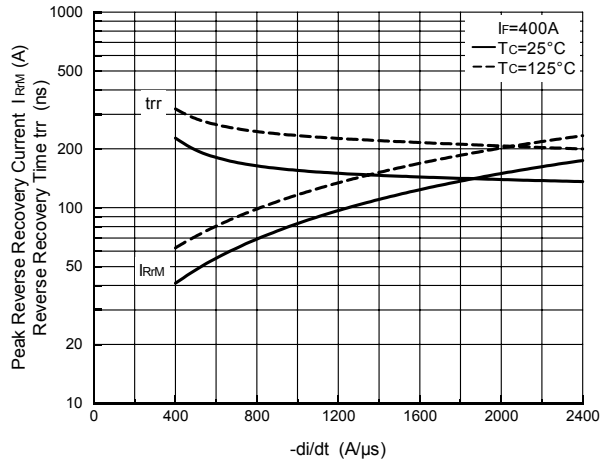
Fig.14- Reverse Recovery Characteristics (Typical)
