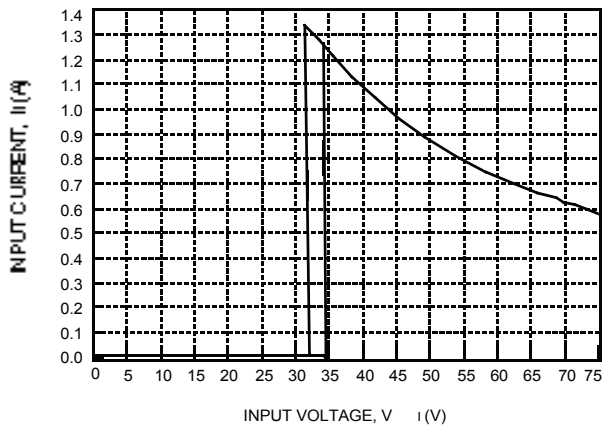
Figure 2. Typical JW075D Input Characteristics at Room Temperature
